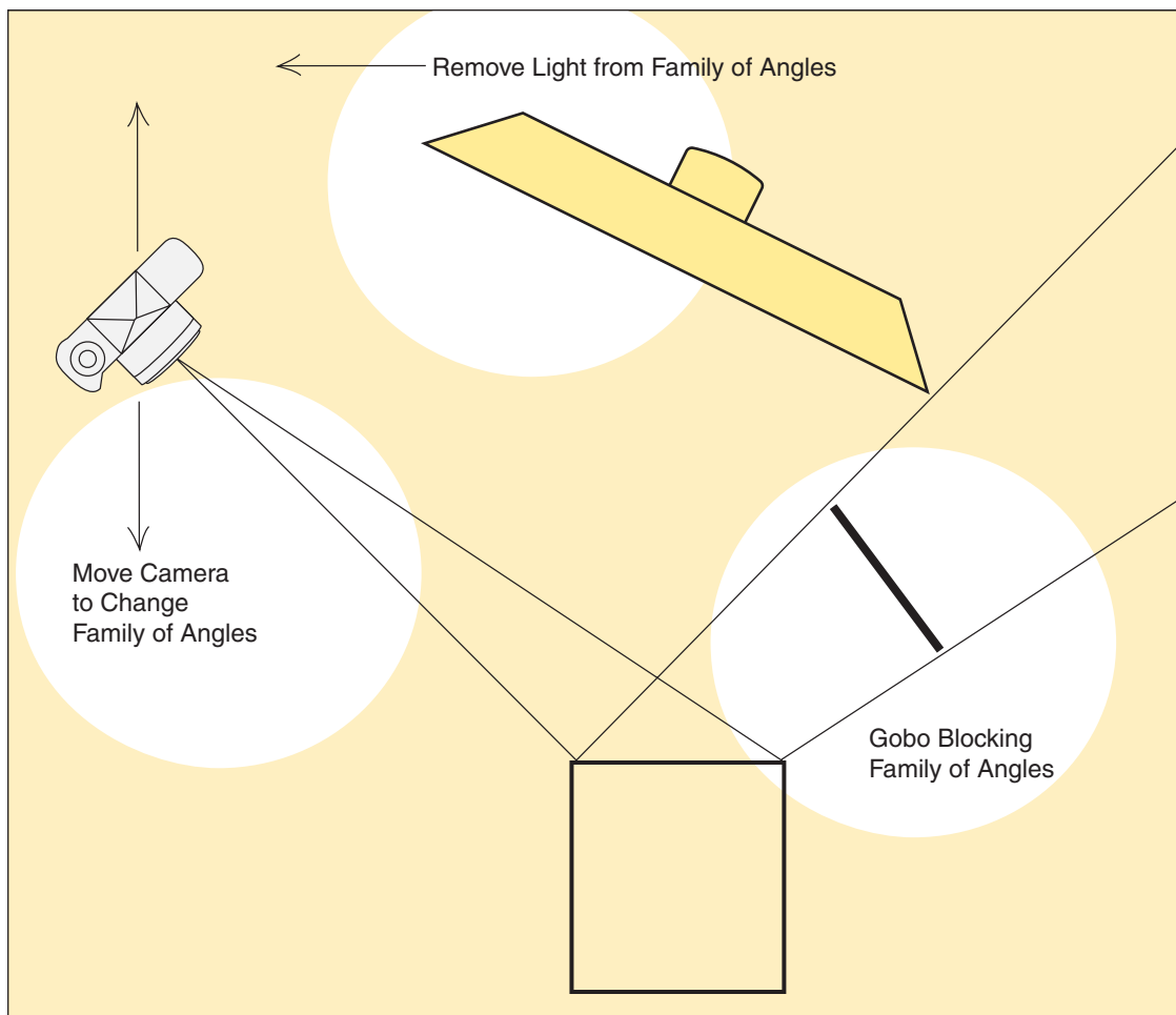
5.22 Here are some of the different ways to eliminate direct reflections from the box top. You can use any one or a combination of them.
