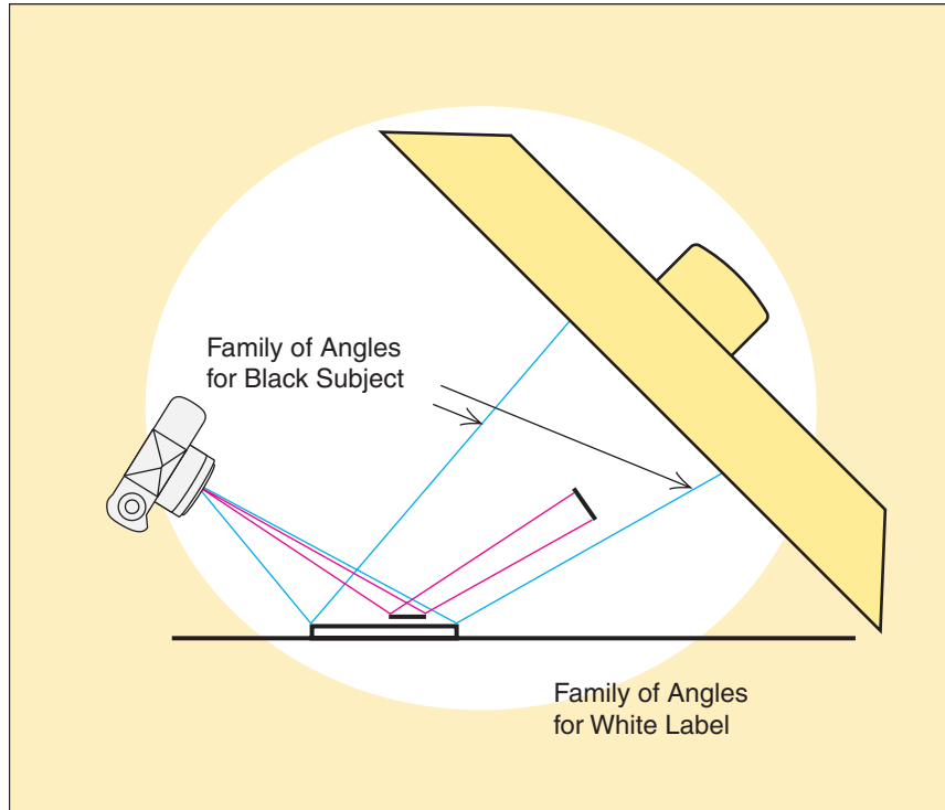
4.24 The small gobo blocks the family of angles that causes a direct reflection on the label but not the one that causes direct reflection on the rest of the subject.
