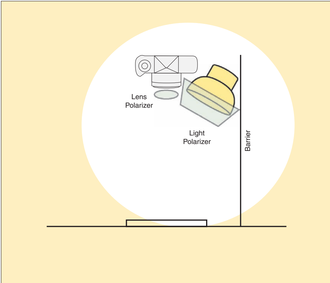
4.12 The solution to the “impossible” lighting requires placing the lights for even illumination and using polarizers to prevent glare. The axis of the light polarizer points to the camera; the axis of the lens polarizer is perpendicular to that.
