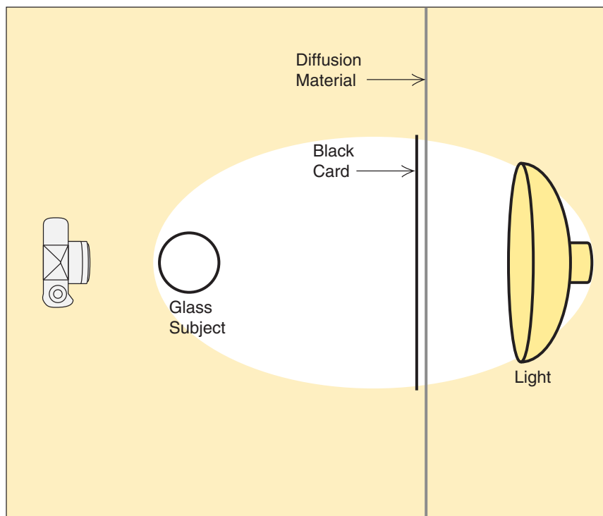
7.6 This is one good way to produce dark-field lighting.
