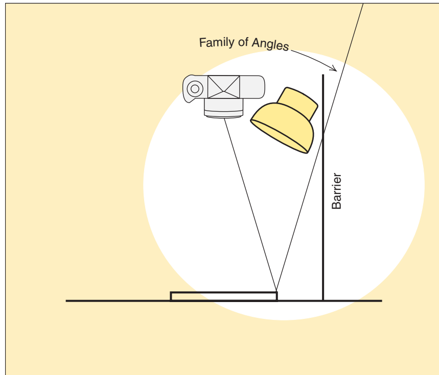
4.10 An “impossible” lighting situation: we cannot position the camera and lights to provide uniform, glare-free illumination.
