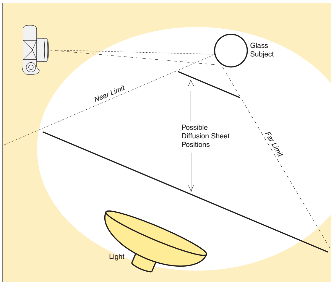
7.10 Creating a highlight on the indicated surface requires filling its family of angles with light. In this diagram, a lighted diffusion sheet reflects on the glass surface to produce the highlight.
