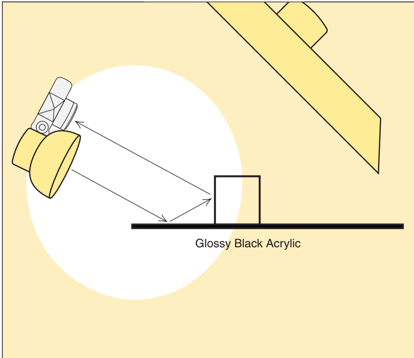
6.27 “Invisible” light reflected from the glossy black plastic lights the metal. No light reflects directly from the plastic to the camera, so the camera cannot see the light source for the metal.
