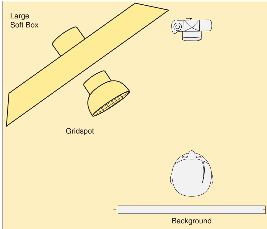
8.39 This diagram shows the “additive” lighting setup we used to make Figure 8.38.
