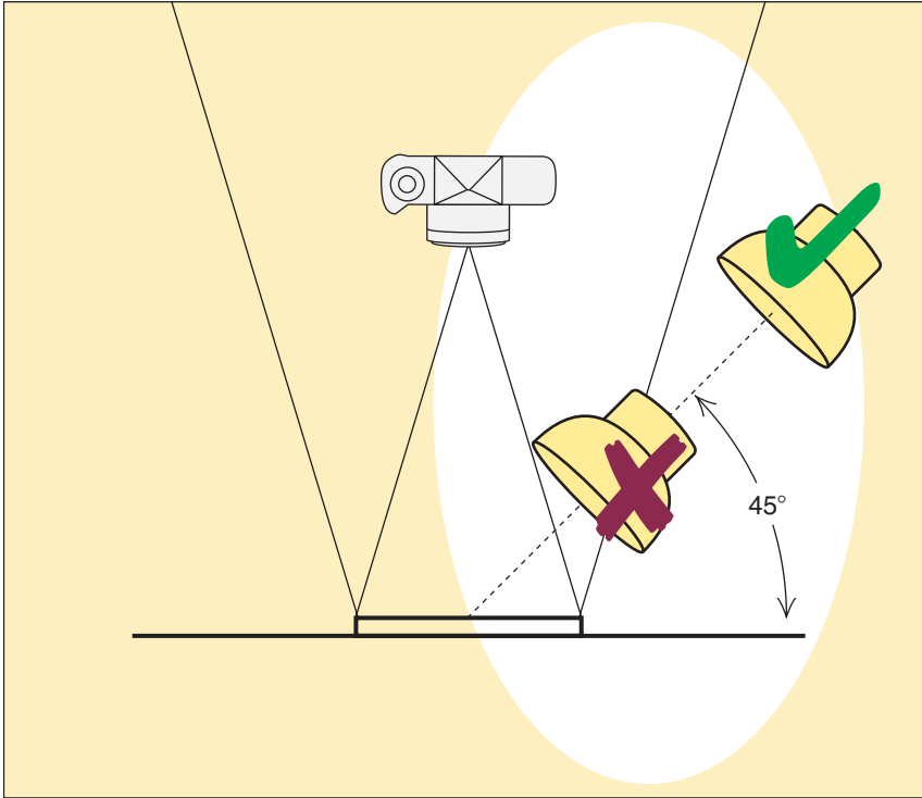
4.7 The importance of the distance from the light to the subject. Both of the lights shown are at 45 degrees to the center of the subject, but only one is satisfactory. The light inside the family of angles will produce direct reflection.
