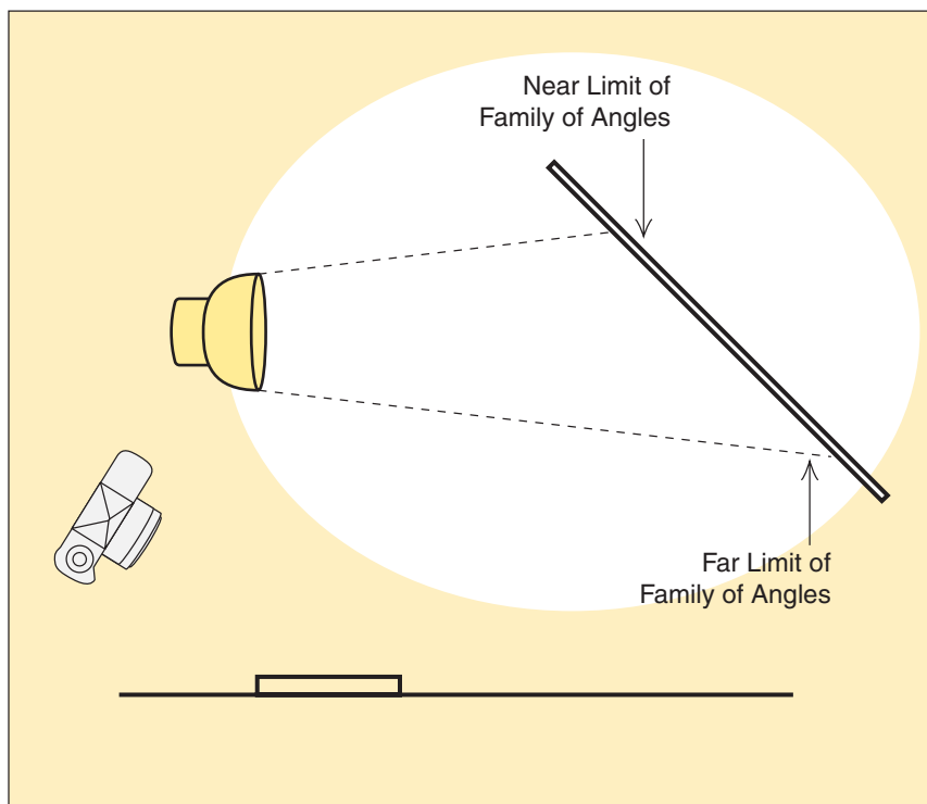
6.5 An alternative to the lighting shown in Figure 6.4 uses an opaque white reflector card and a spotlight focused to fill the family of angles.
