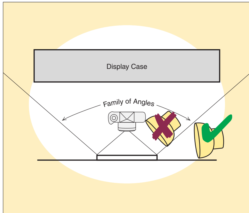
4.4 The family of angles has grown much larger in this arrangement using a wide-angle lens. The result is a small range of acceptable lighting angles. Only the light outside the family of angles will produce glare-free lighting.
