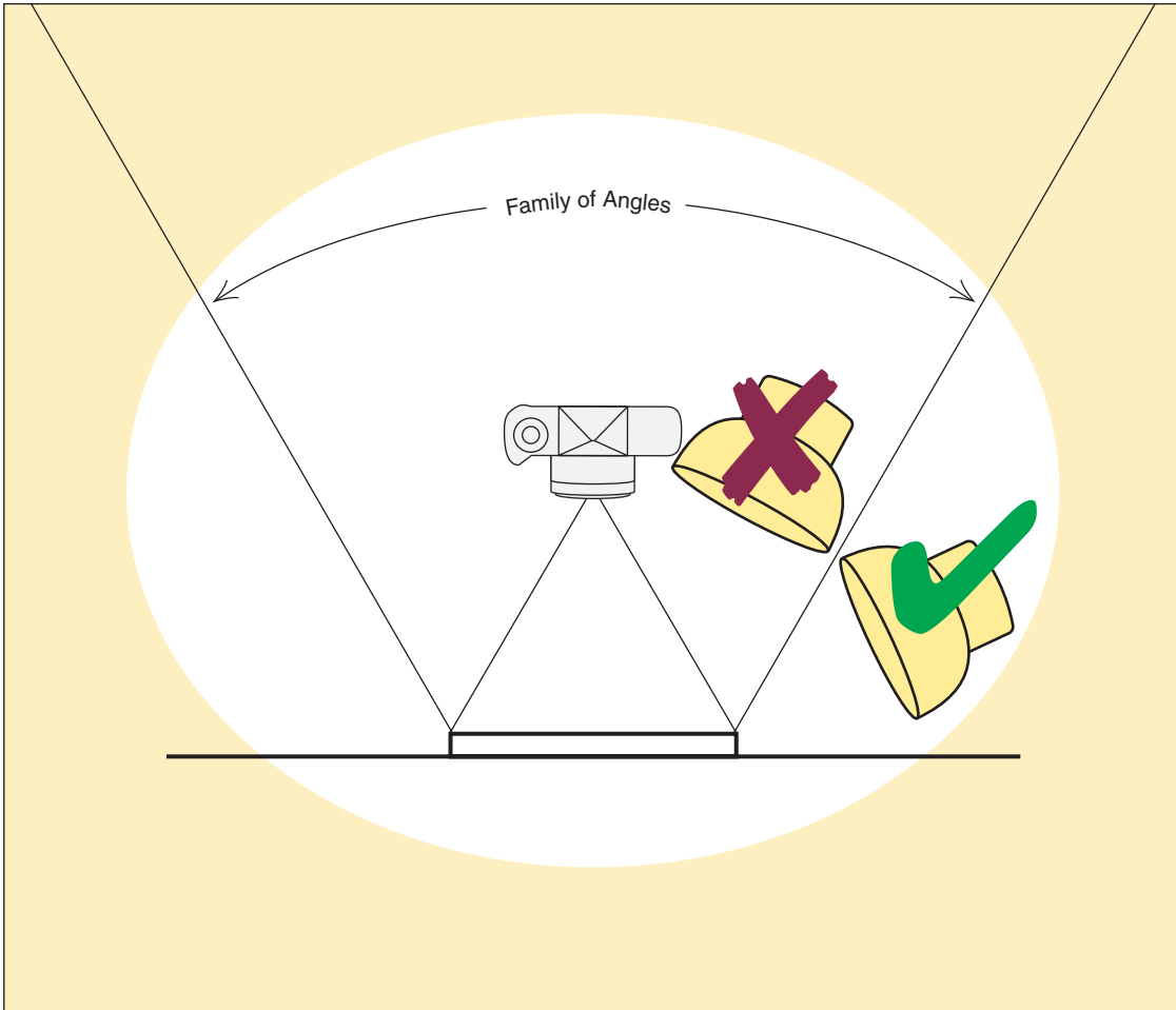
4.1 The family of angles that produces direct reflections in a “copy” lighting setup. The light inside the family of angles will produce direct reflection; the other will not. There is a similar family of angles on each side of the camera.
