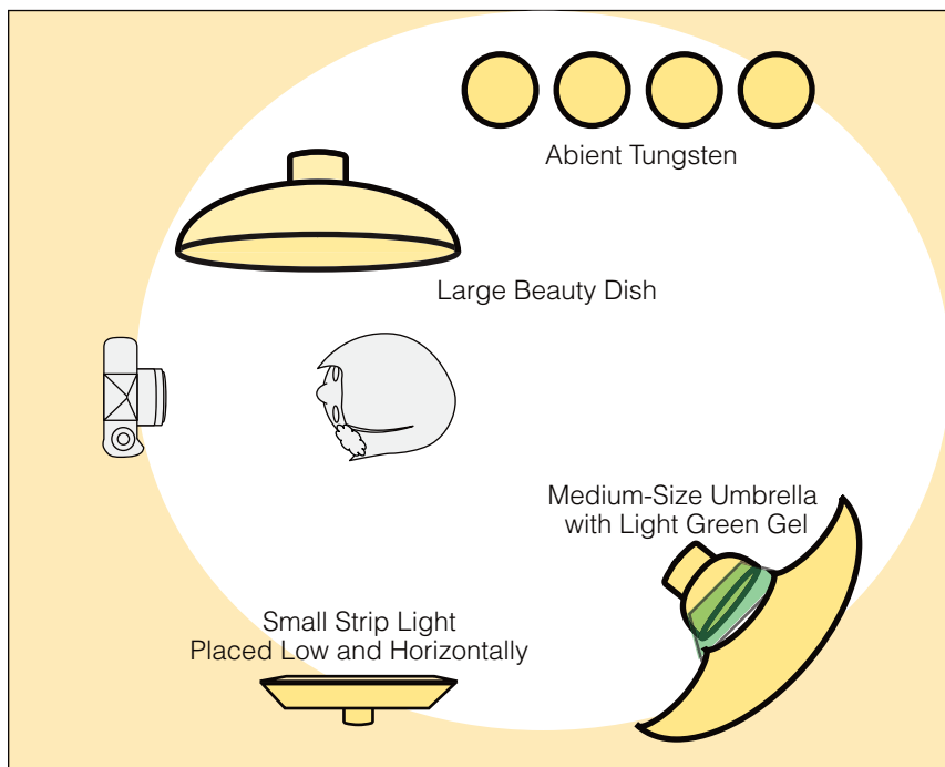
8.36 This diagram shows the setup we used to make Miss Prissy's on-location mixed ambient light and flash portrait.
