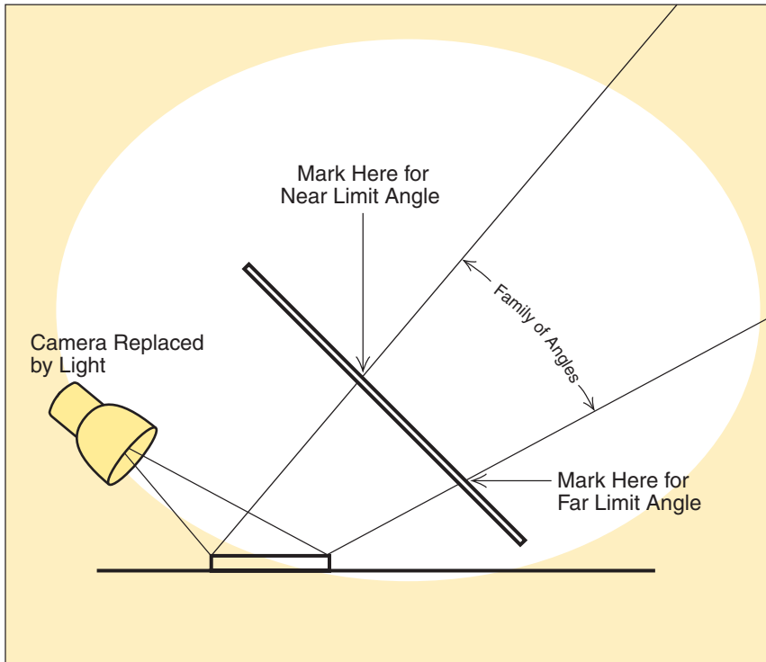
6.3 A test light in place of the camera reflects from the metal to show where the family of angles is located. News flash: Since the last printing of this book, a clever reader has suggested using a laser pointer as the test light. Should work well!
