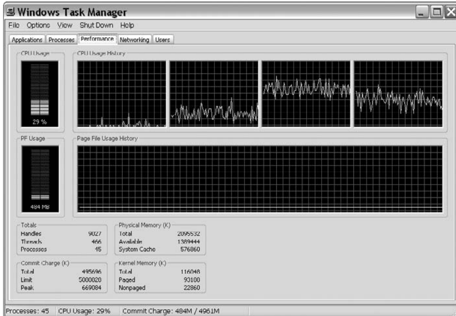
Figure 11.4 More threads are balanced more equitably on a multi-core processor.
