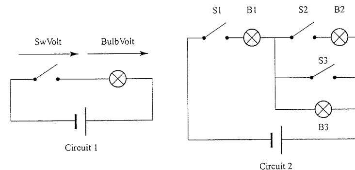
Figure 20.2 Simple circuits made of switches, bulbs and batteries.
