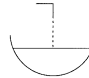
Figure 20.1 Bath tub with some input flow and closed drain.
