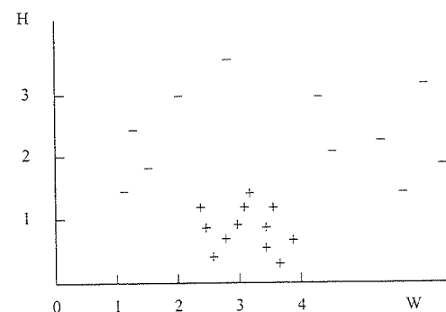
Figure 18.1 Examples for learning about mushrooms. The attributes are W (width) and H (height) of a mushroom. The pluses indicate examples of edible mushrooms, the minuses examples of poisonous ones.
