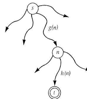
Figure 12.1 Construction of a heuristic estimate f(n) of the cost of the cheapest path from s to t via n : f(n) = g(n) + h(n) .
