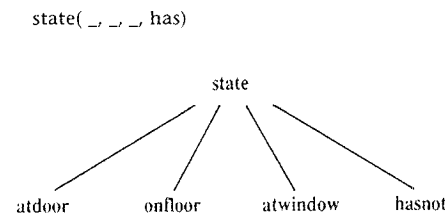
Figure 2.12 The initial state of the monkey world represented as a structured object. The four components are: horizontal position of monkey, vertical position of monkey, position of box, monkey has or has not banana.
