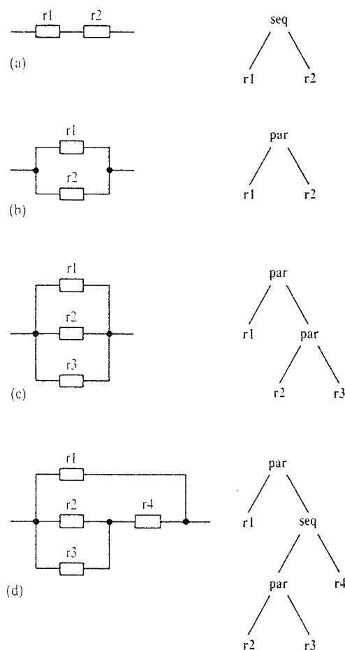
Figure 2.6 Some simple electric circuits and their tree representations: (a) sequential composition of resistors r1 and r2 ; (b) parallel composition of two resistors; (c) parallel composition of three resistors; (d) parallel composition of r1 and another circuit.
