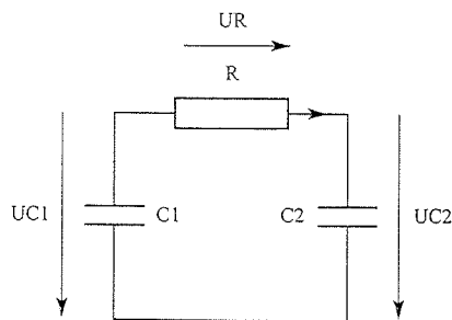
Figure 20.10 An electric circuit with two capacitors and a resistor.
