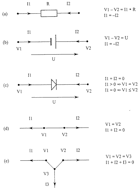
Figure 14.5 Components and connections for electrical circuits, and the corresponding constraints; (a) resistor; (b) battery; (c) diode; (d, e) connection between two or three terminals.
