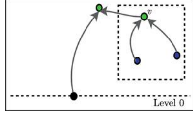
Fig. 5. A Section of a Reeb graph with unreachable vertices shown in the boxed rectangle. The unreachable component prevents the algorithm to proceed beyond the merge saddle v .
