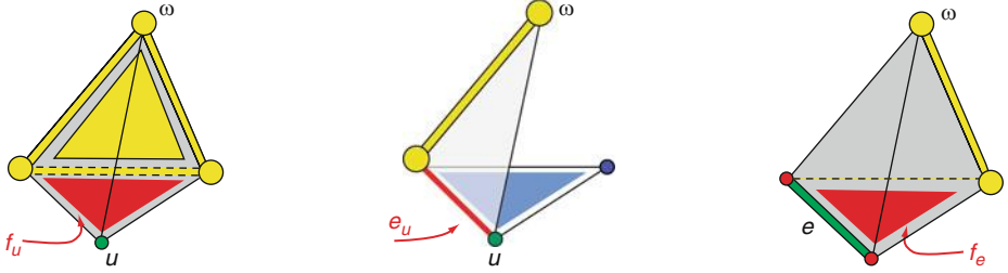
Fig. 5. Contribution to the links from the extended simplices around a reference simplex ( u or e shown in green). \omega represents the dummy vertex. The substructures are shown in red and the simplices to insert into the links in yellow.
