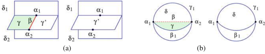
Fig. 2. Part of a 3D descending Morse complex before and after a removal (a) rem(\gamma, \beta, \gamma') , and (b) rem(\gamma, \beta, \emptyset) .
