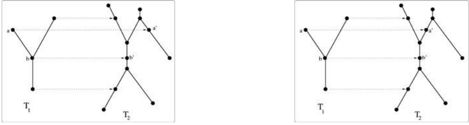
Fig. 1. Left: a mapping of vertices of T_1 into vertices of T_2 that does not define a height-preserving continuous map between trees (i.e. a morphism in S ). There is no monotone path between the images of vertices a and b in T_2 . Right: a mapping that does define a morphism in S . For every edge of T_1 there is a monotone path connecting the images of the endpoints in T_2 .
