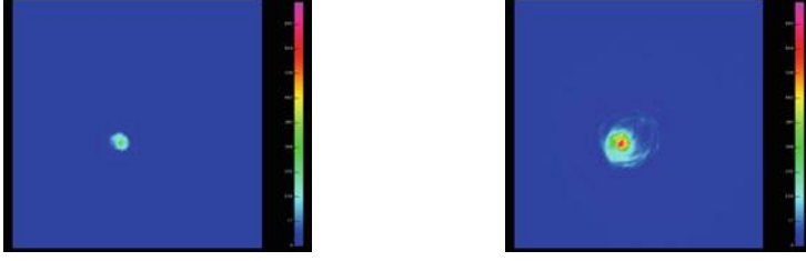
(a) Density of particles traced from one grid at t = 50 . (b) Density of particles traced from ten grids at t = 50, 52, \dots, 68 .
