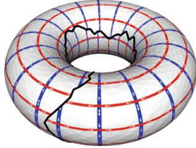
Fig. 6. Parameterization after the first stage. Grid lines are discontinuous across the cuts.
