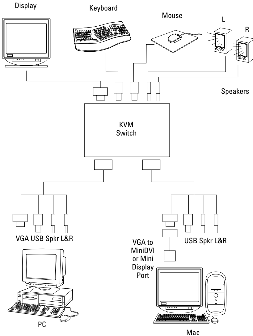
Figure 4-2: KVM wiring.
