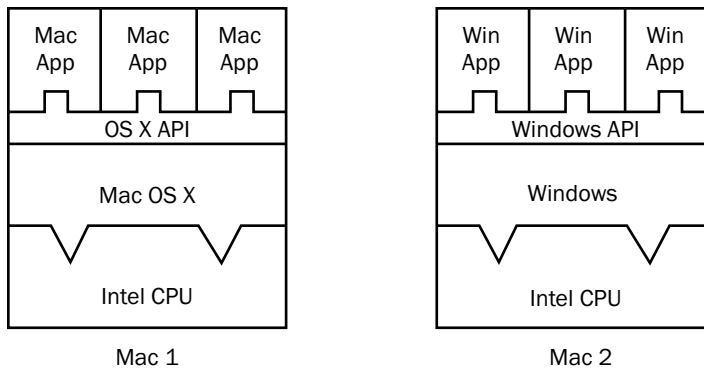
Figure 16-2: Two Macs, two operating systems.
