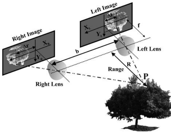
Figure 5.2 Principal parameters involved in stereoscopic vision
