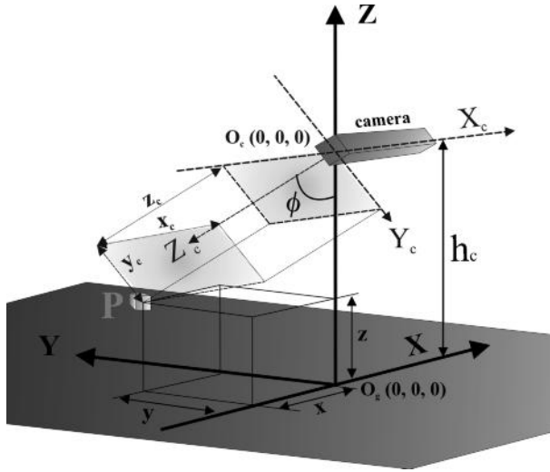
Figure 5.31 Transformation from camera coordinates to ground coordinates for ground images
