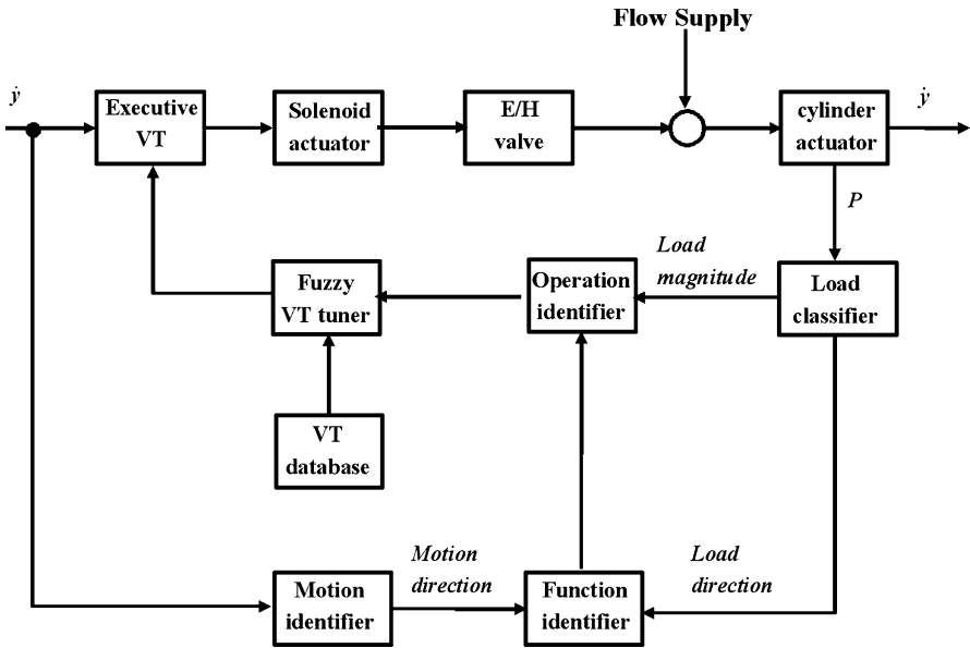
Figure 7.16 Working principle of a fuzzy adaptive navigation controller
