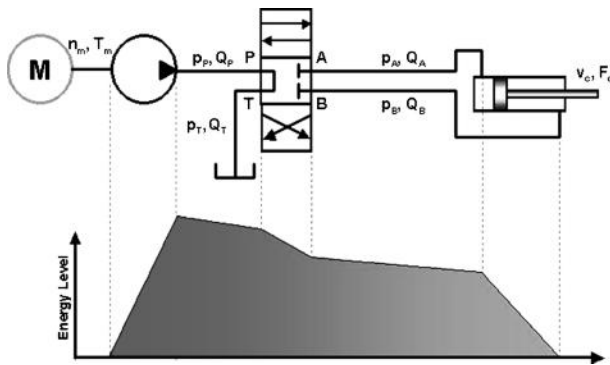
Figure 7.4 Transmission of energy in a fluid power circuit
