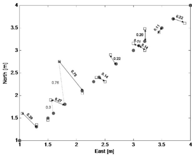
Figure 3.14 Simulated example for the trajectory matching algorithm
