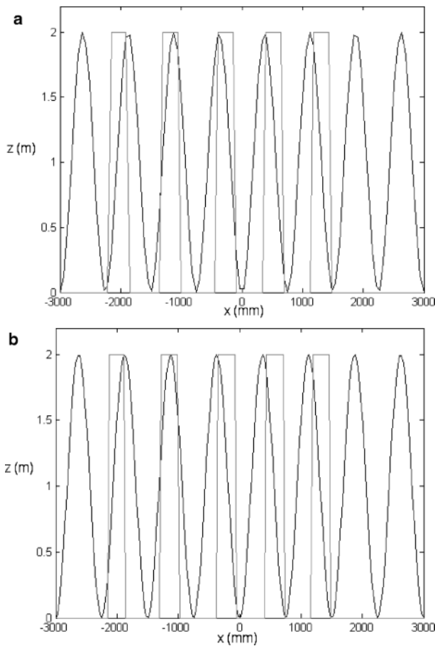
Figure 5.71 Cross-correlation results: (a) before correcting the offset; (b) after offset correction
