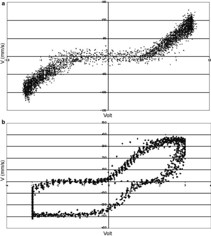
Figure 7.23 Responses to varying frequencies and amplitudes: (a) 0.1 Hz and 150 mm; (b) 2 Hz and 25 mm
