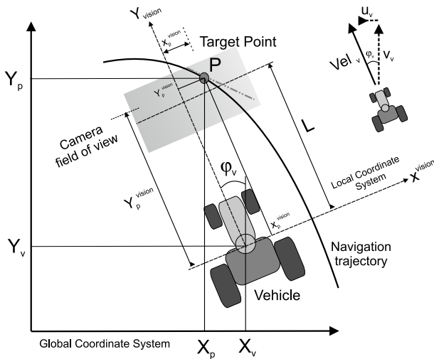
Figure 4.34 Geometry of navigation for global-local sensor fusion: basic parameters
