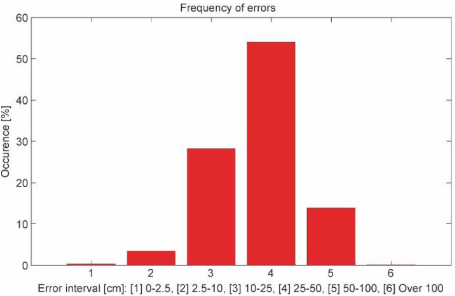
Figure 3.16 Error occurrence for a harvester automatically guided at 6 km/h
