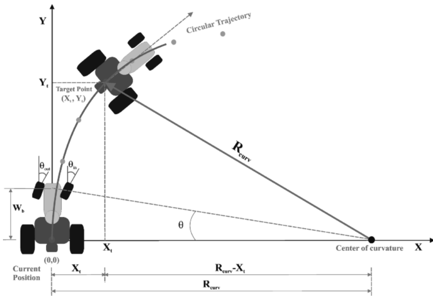
Figure 8.7 Geometry used to estimate steering commands with SAE Standard J695
