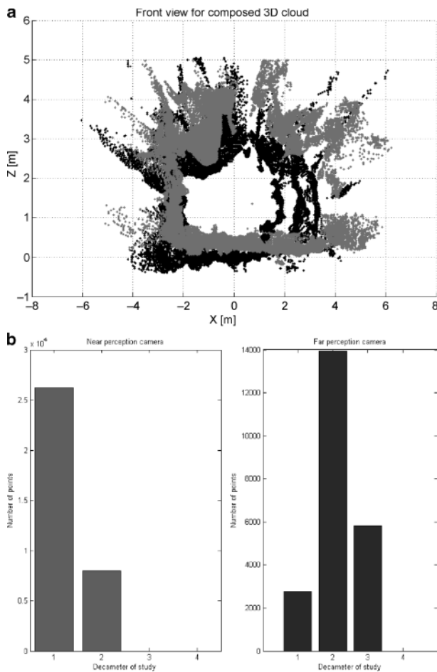
Figure 5.61 Front view (a) and distribution of points (b) for a bifocal camera 3D cloud
