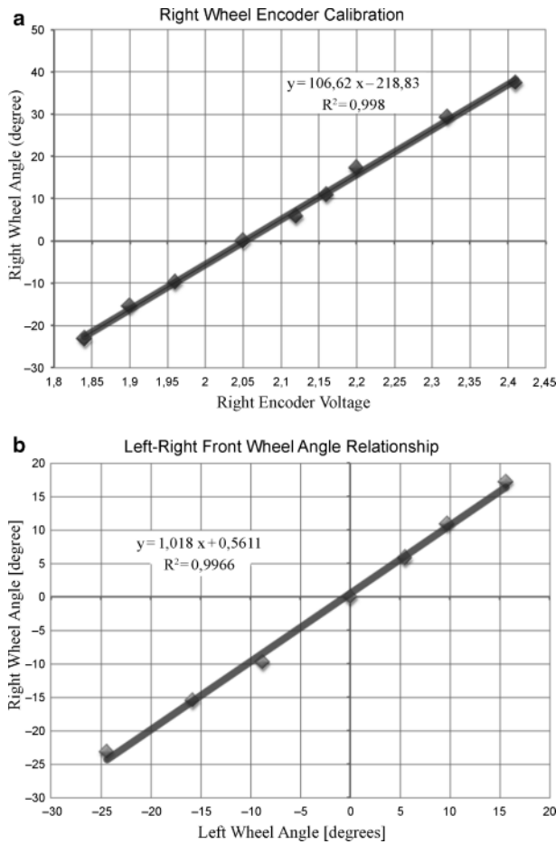
Figure 7.3 Calibration results for the encoder (installed in right wheel) shown in Figure 1.7a: (a) relationship between the voltage readings of the encoder and the corresponding angles turned by the right wheel; (b) angles turned by both front wheels for moderate angles
