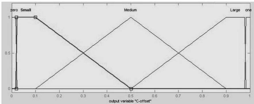
Figure 8.4 Fuzzy logic (output) membership functions for the offset mixing ratio
