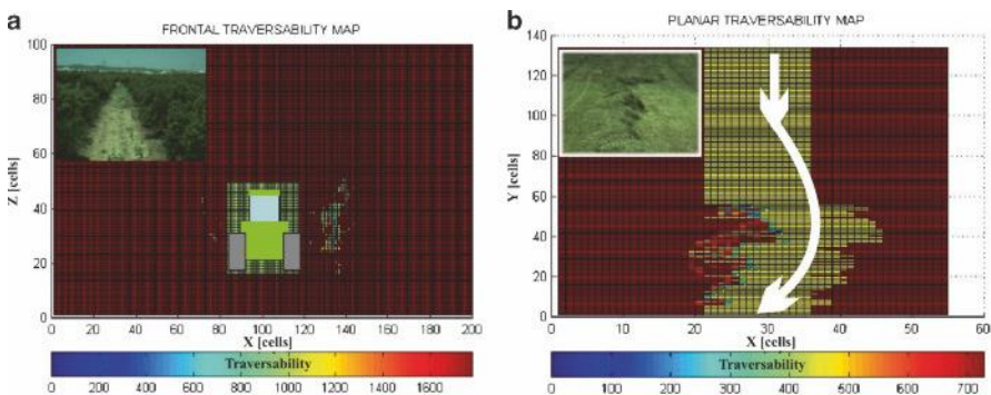
Figure 8.9 Traversability analyses of agricultural scenes: (a) frontal map (FTM) for orchards; (b) planar map (PTM) of a windrow
