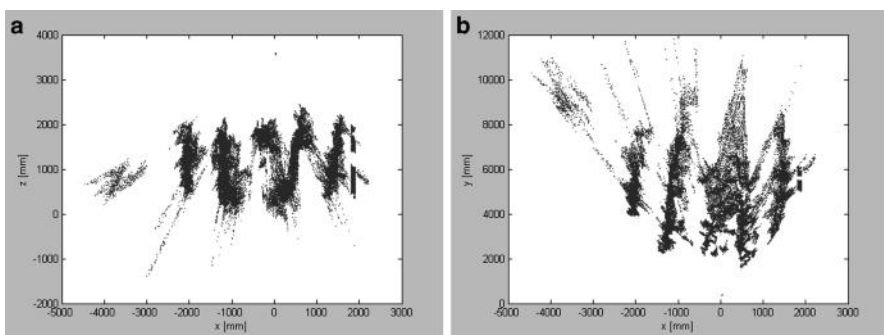
Figure 5.63 Point cloud from crop-tracking images: (a) front view; (b) top view
