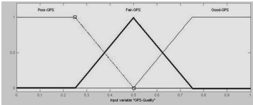
Figure 8.3 Fuzzy logic (input) membership functions for GPS quality estimates
