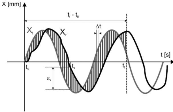
Figure 7.31 Graphical visualization of the concept of the error index (EI)
