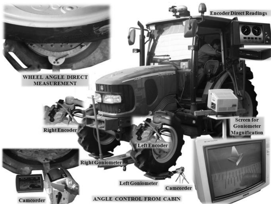
Figure 7.2 Calibration procedure for optical encoders mounted on the front wheels of a tractor
