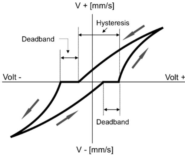
Figure 7.12 Characteristic curve of an electrohydraulic valve
