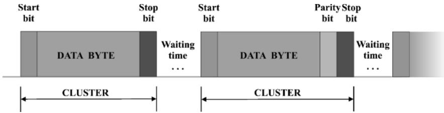
Figure 6.1 Asynchronous data transmission for serial communication
