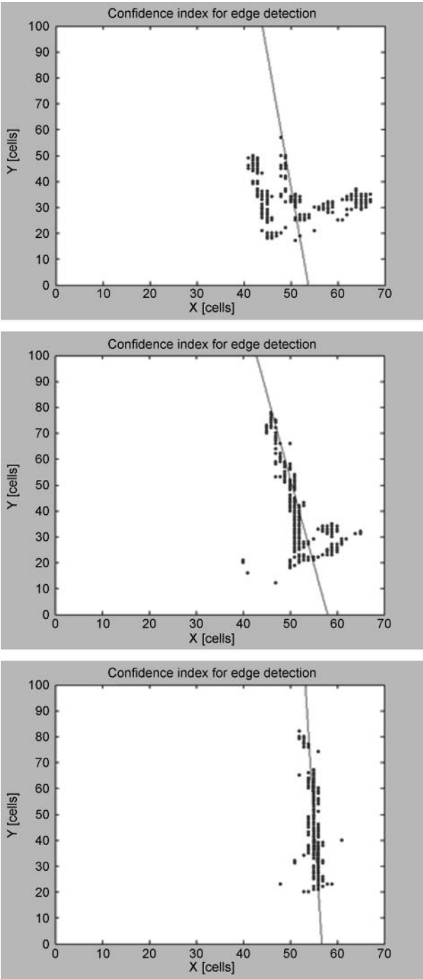
Figure 5.39 Confidence metrics for edge detection: (a) CI = 60%; (b) CI = 80%; (c) CI = 94%
