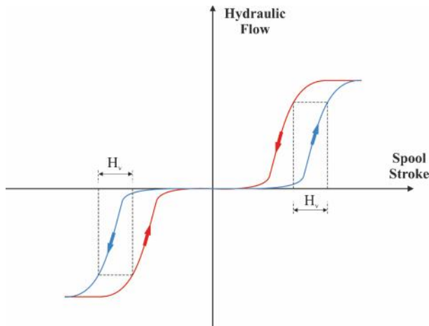
Figure 7.10 Spool valve hysteresis
