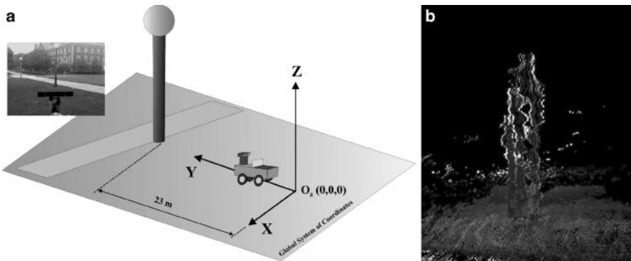
Figure 5.32 Erroneous global maps due to GNSS failures: (a) experiment; (b) 3D field map
