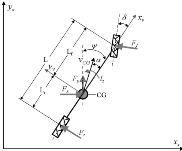
Figure 2.6 Definition of the bicycle model in site coordinates
