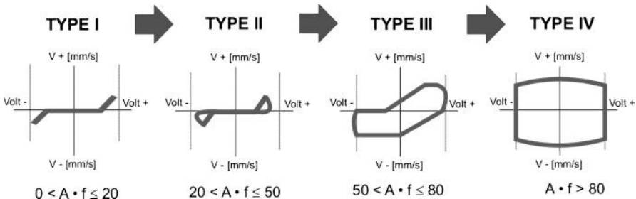
Figure 7.25 Evolution of characteristic curves according to the product of amplitude and frequency
