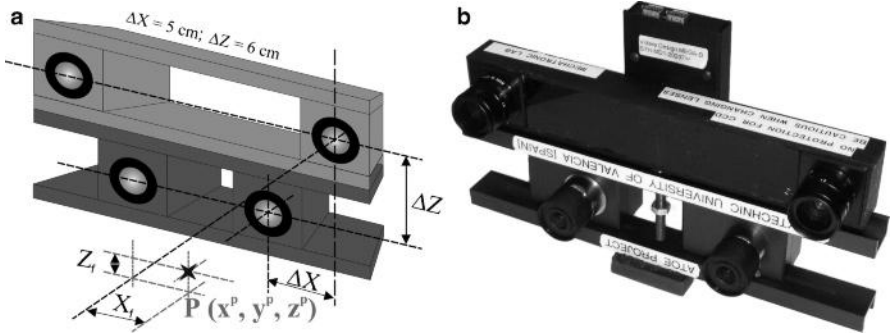
Figure 5.12 Bifocal stereo camera: conceptual design (a) and real head (b)
