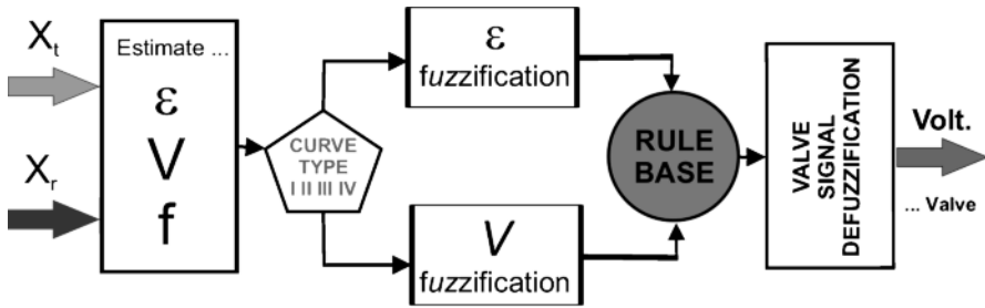
Figure 7.27 Fuzzy logic control system for hydraulic automatic steering
