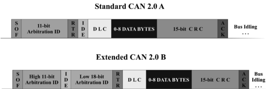
Figure 6.2 Frame formats for the standard and extended CAN protocols
