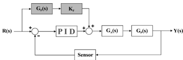
Figure 7.19 System diagram of a feedforward-PID control system
