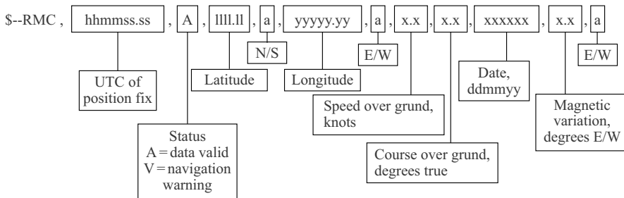
Figure 6.7 Specifications for RMC NMEA messages
