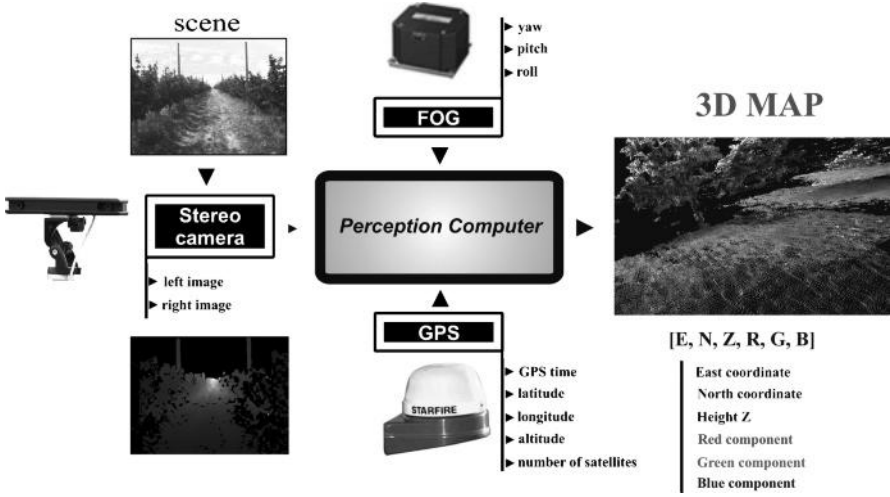
Figure 5.27 System architecture for a global 3D mapping platform
