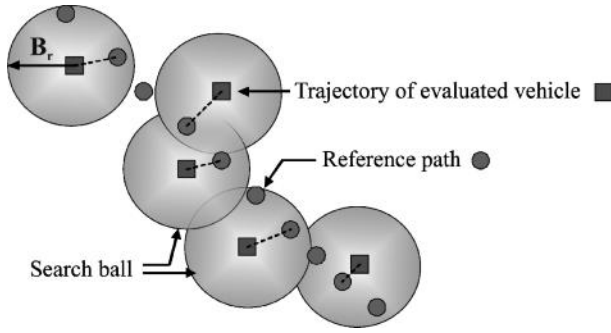
Figure 3.12 Conceptual representation of the trajectory matching algorithm
