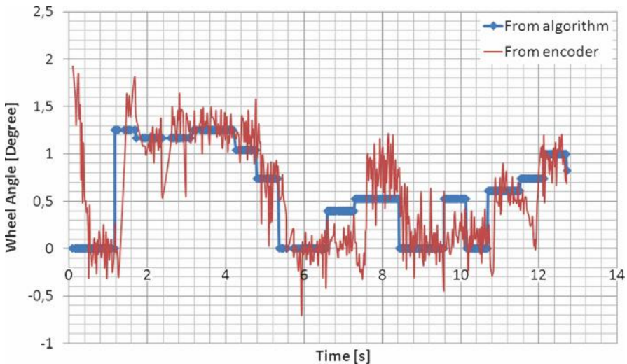
Figure 4.31 Theoretical and real angles turned by the front right wheel of an autosteered tractor
