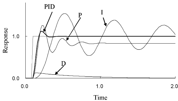
Figure 7.18 Contributions of the individual modes of PID controllers to the final response
