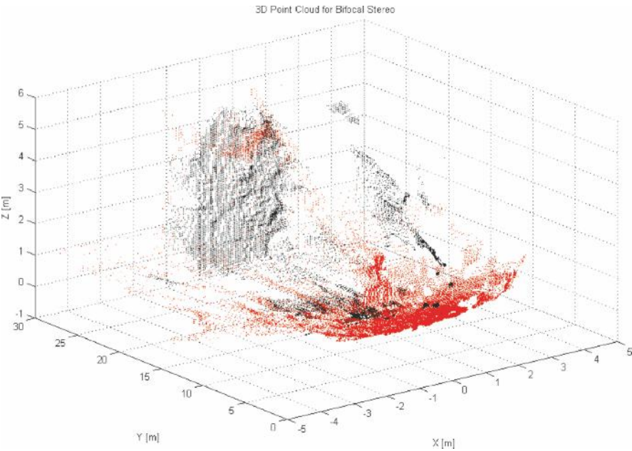
Figure 5.57 Perspective view of the merged point cloud for the scene represented in Figure 5.56
