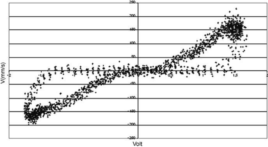
Figure 7.13 Characteristic curve for an EH valve tested at 1 Hz and for displacements of 25 mm
