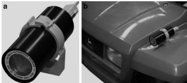
Figure 4.4 Ultrasonic sensor (a) used in the safety alert system of an agricultural vehicle (b)
