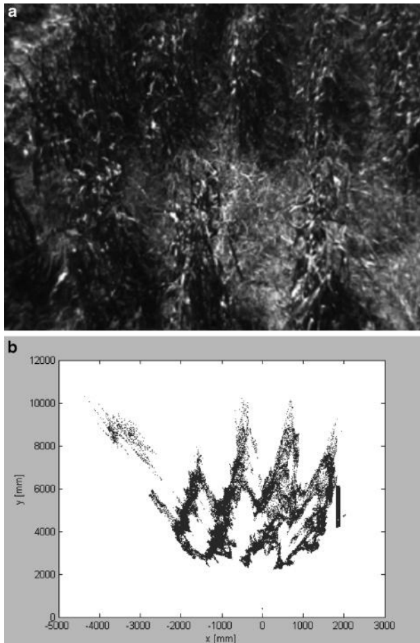
Figure 5.72 Tracking challenging (patchy) rows: (a) monochrome image; (b) top view of point cloud
