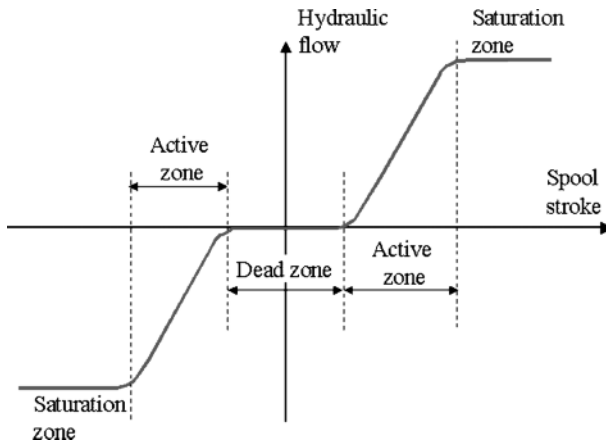
Figure 7.9 Typical valve transform curve for a general spool valve
