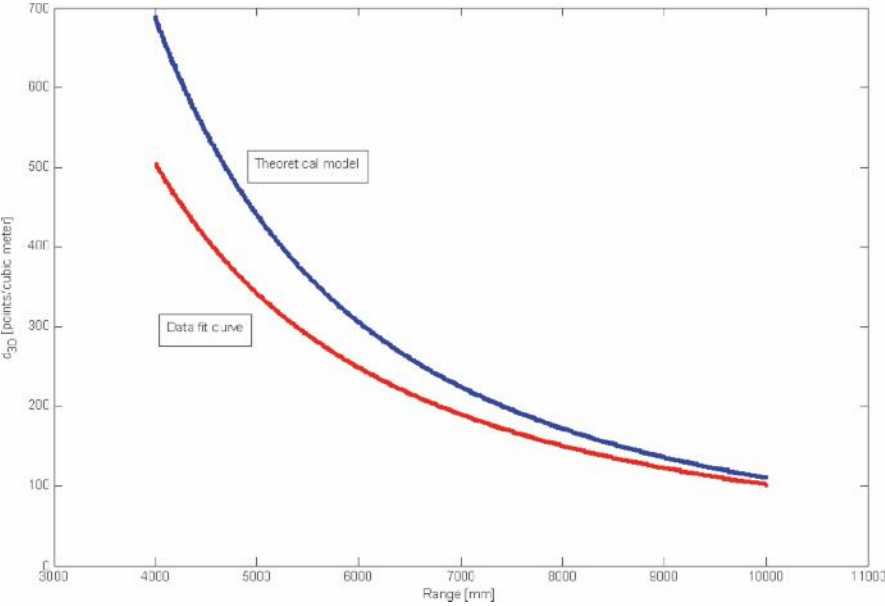
Figure 5.25 Theoretical and practical relationship between d_{3D} and stereo ranges
