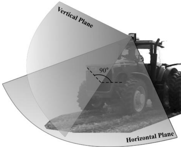
Figure 5.34 Nodding laser for rendering 3D agricultural maps
