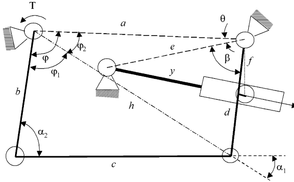
Figure 2.7 Four-bar steering mechanism used in agricultural tractors
