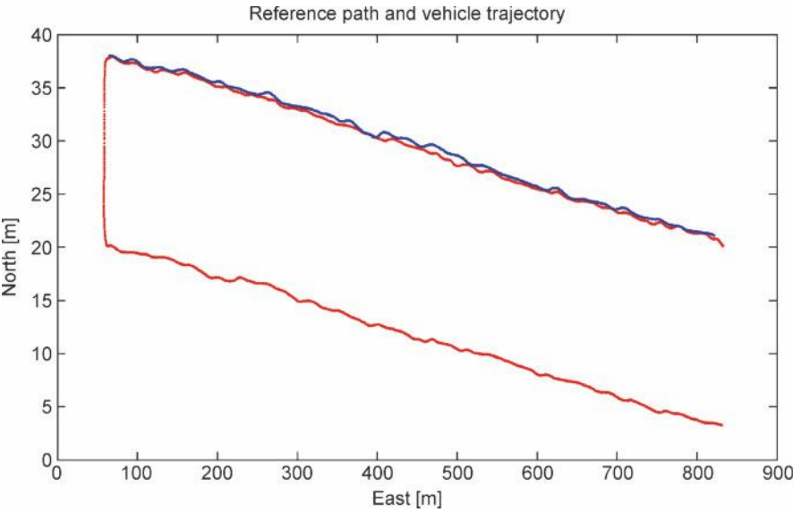
Figure 3.15 Reference path and trajectory followed by an autoguided harvester at 6 km/h
