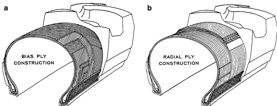
Figure 2.14 Tire constructions: (a) bias ply; (b) radial ply [9]
