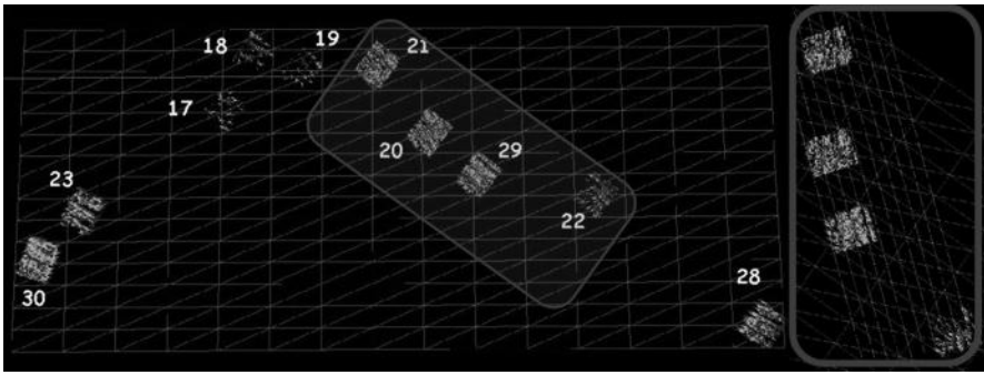
Figure 5.48 Virtual 3D map of a maize field generated from aerial stereoscopic images
