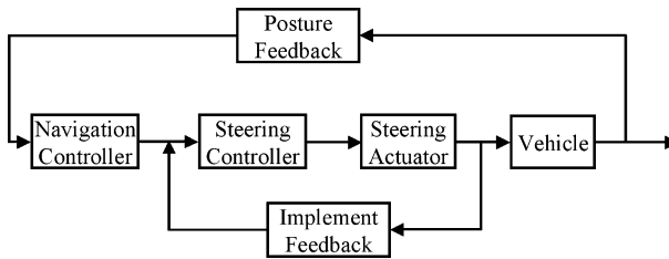
Figure 7.15 Basic components of intelligent steering controllers
