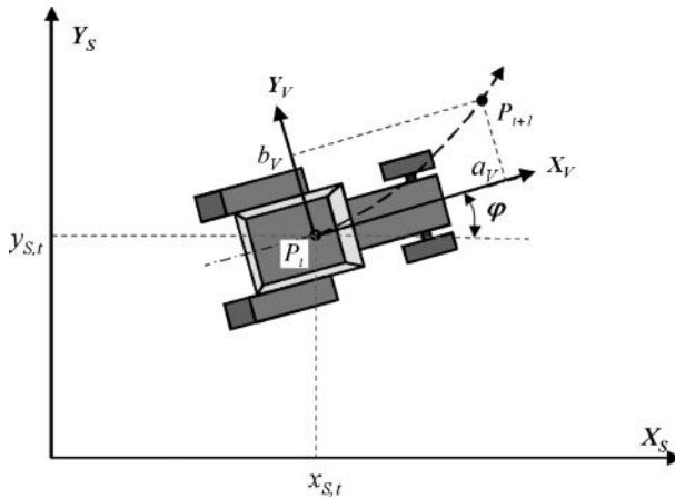
Figure 2.2 Relationship between site-specific and vehicle-fixed coordinate systems
