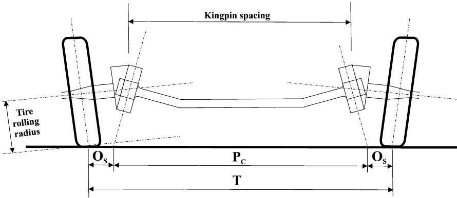
Figure 8.8 Key parameters of front-axle configuration vehicles
