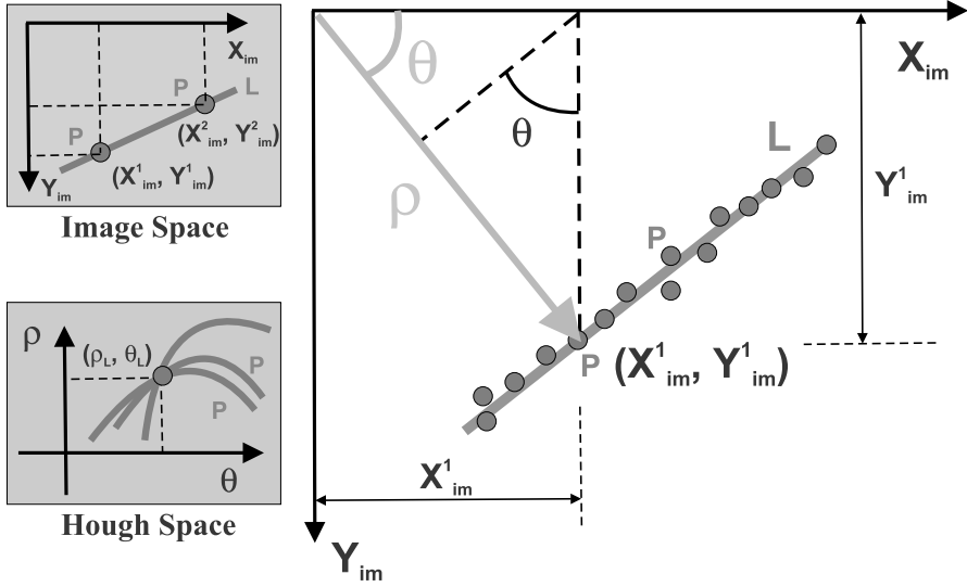
Figure 4.15 Parametric representation of a line with the Hough transformation
