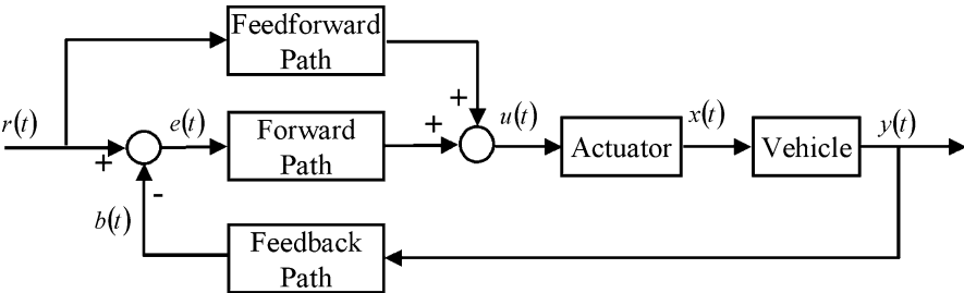
Figure 7.14 Block diagram of a generic steering controller
