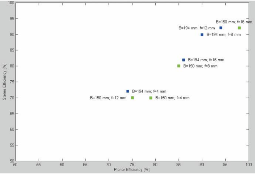
Figure 5.22 Efficiency chart for a range of 12 m
