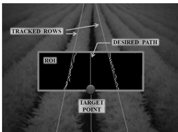
Figure 4.29 Typical outcome from the vision algorithm implemented for Case Study I
