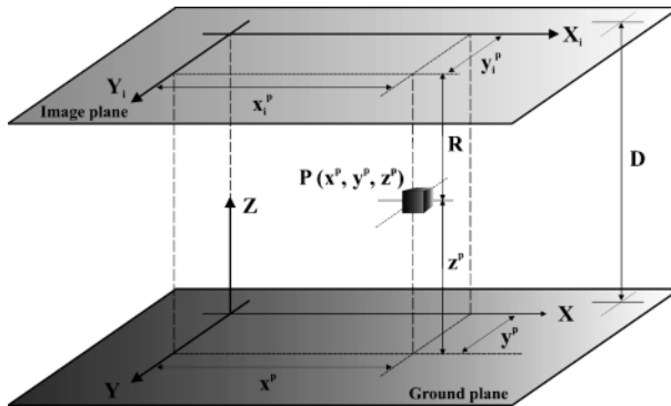
Figure 5.29 Transformation to ground coordinates for aerial images
