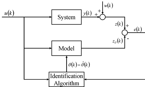
Figure 7.22 Principles of empirical system identification
