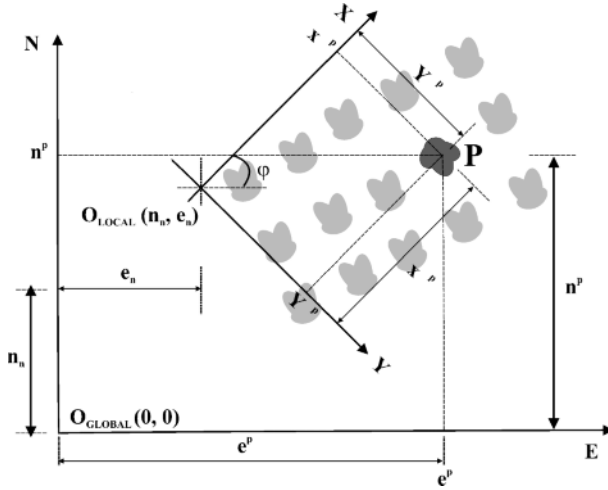
Figure 5.30 Transformation from local coordinates to global coordinates for aerial images
