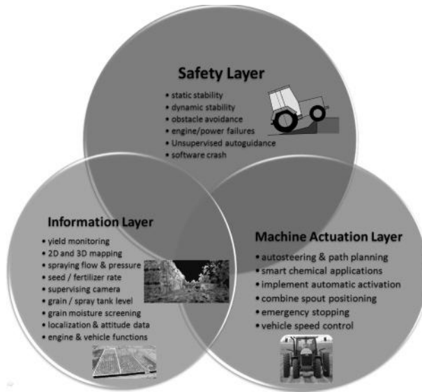
Figure 8.1 Basic tasks assigned to off-road intelligent vehicles in agricultural fields
