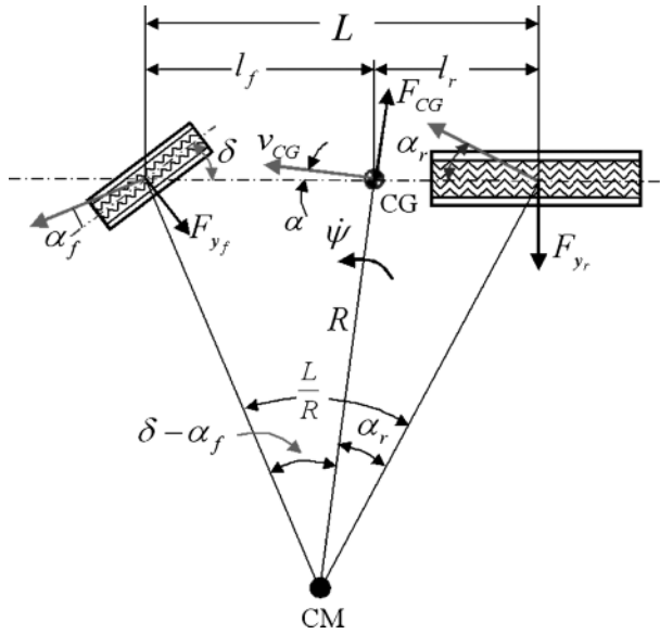
Figure 2.5 Bicycle model for analyzing the steering systems of rigid-body vehicles
