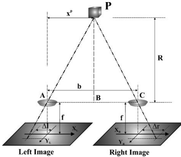
Figure 5.3 Calculation of ranges from disparities
