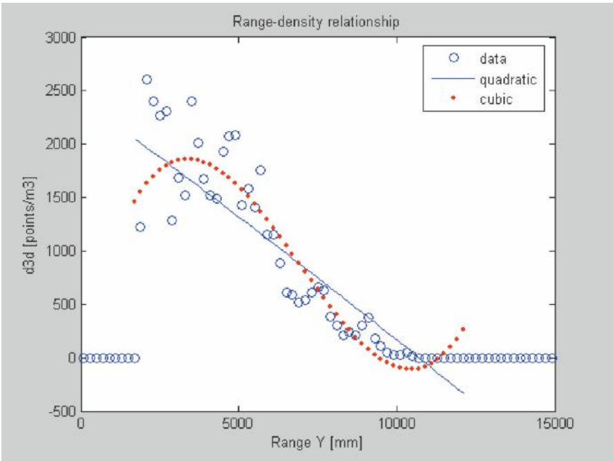
Figure 5.65 Distribution of 3D densities according to range for crop-tracking images
