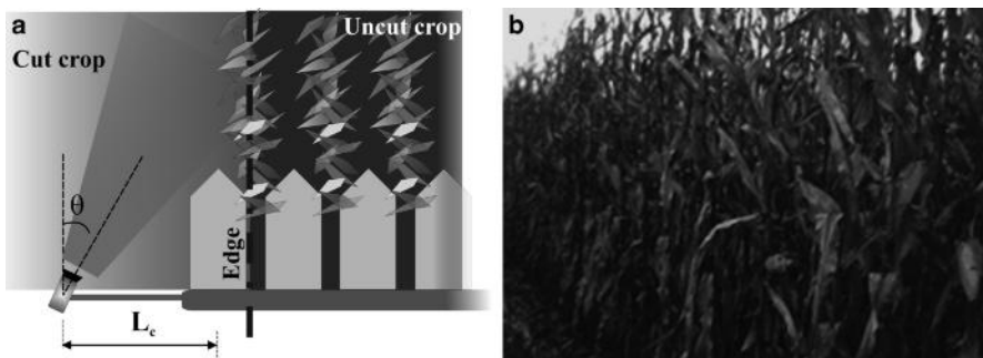
Figure 5.36 The camera's position and orientation on the corn harvester (a), and a sample image of the cut–uncut edge (b)
