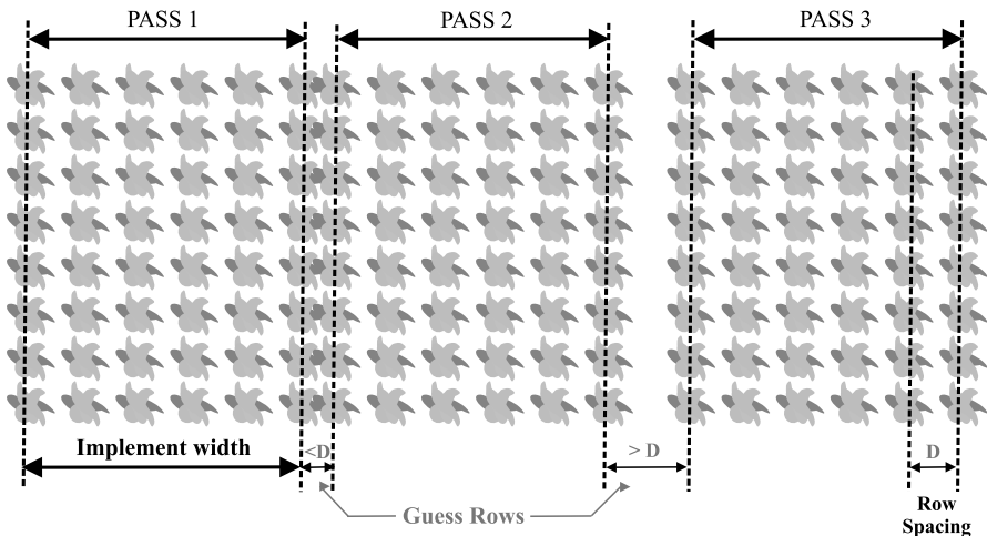
Figure 4.3 The problem of guess rows for parallel tracking autoguidance
