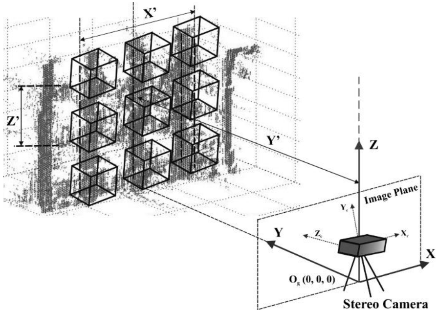
Figure 5.20 Experimental setup for evaluating the perceptive performances of stereo cameras
