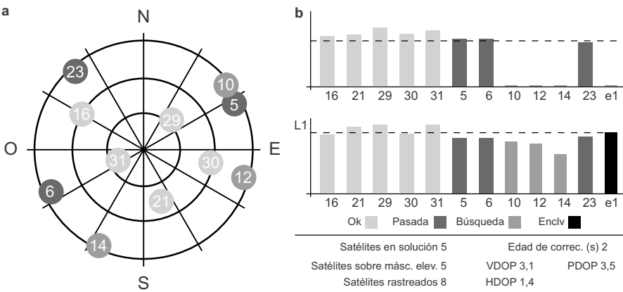
Figure 3.11 Satellites in view for a vehicle-mounted DGPS (a); HDOP and VDOP (b) (courtesy of Deere & Co.)
