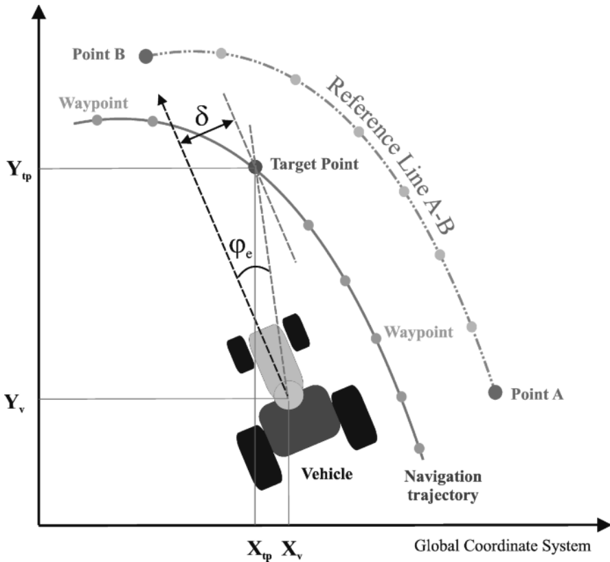
Figure 3.7 Geometry of the GPS guidance of an intelligent off-road
