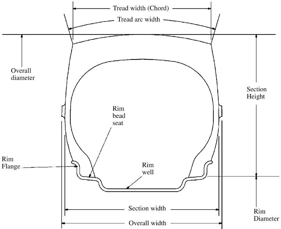
Figure 2.13 Tire dimensions and terminology [8]
