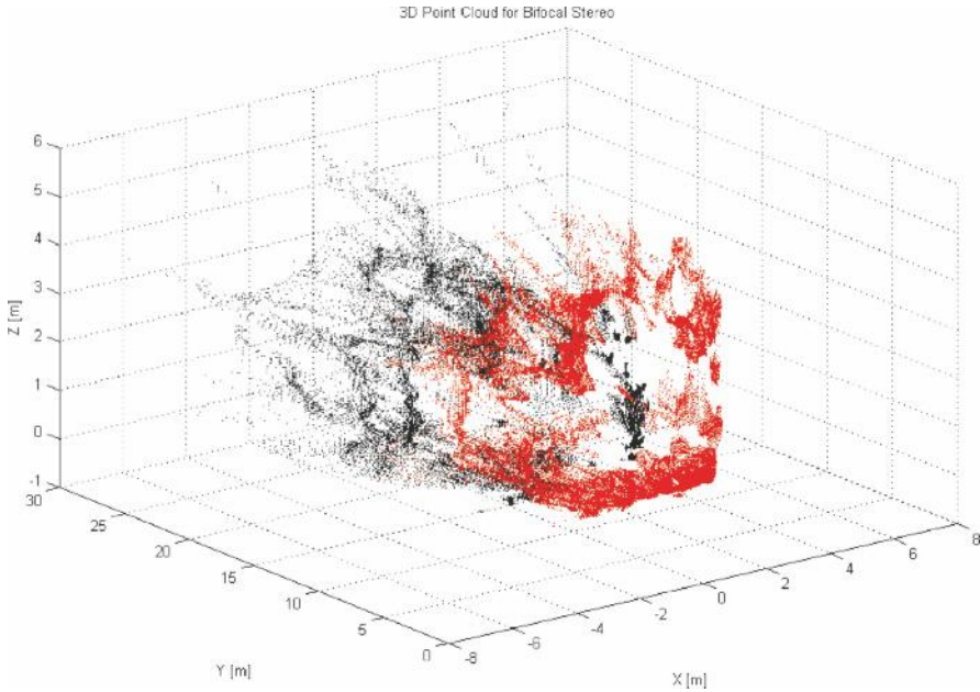
Figure 5.60 Perspective view of the merged point cloud for the scene represented in Figure 5.59
