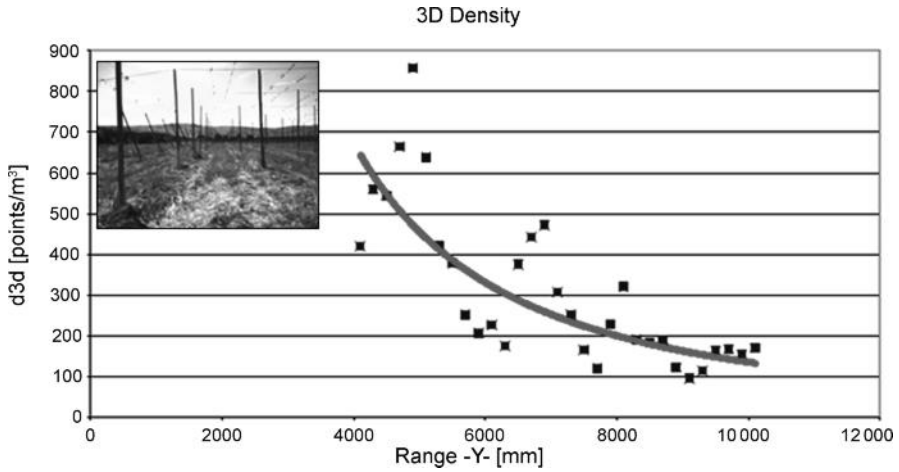
Figure 5.24 Distribution of 3D density with range for a field stereo image
