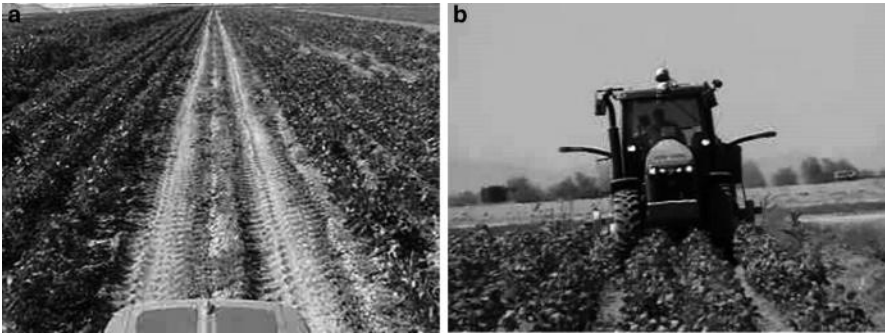
Figure 4.26 Automatic guidance with deteriorated rows (a) and at high speeds (b)
