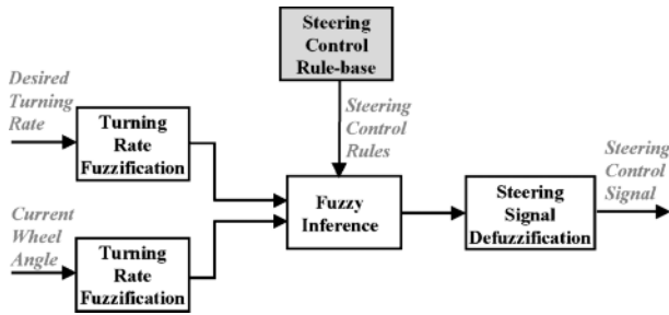
Figure 7.21 Fuzzy steering controller for off-road vehicles
