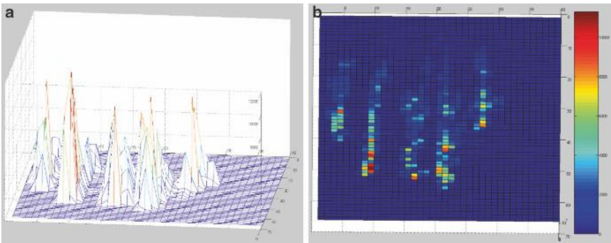
Figure 5.64 Density grid for crop-tracking images: (a) 3D perspective view; (b) top view
