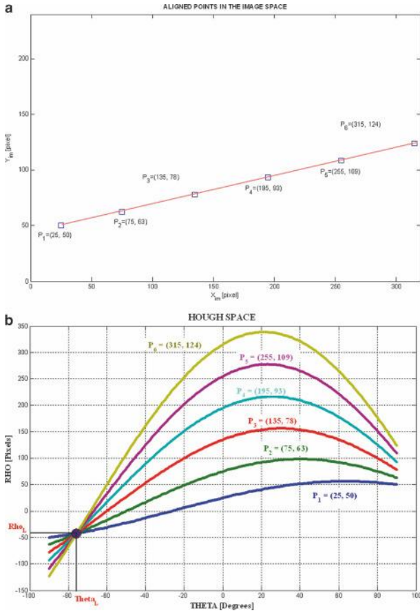
Figure 4.16 Example of the application of the Hough transform for line detection
