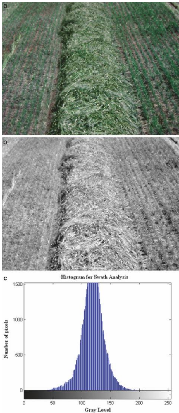
Figure 4.18 Cut swath selected as a tracking feature for machine vision based autoguidance: (a) original image; (b) monochrome image; (c) resulting histogram
