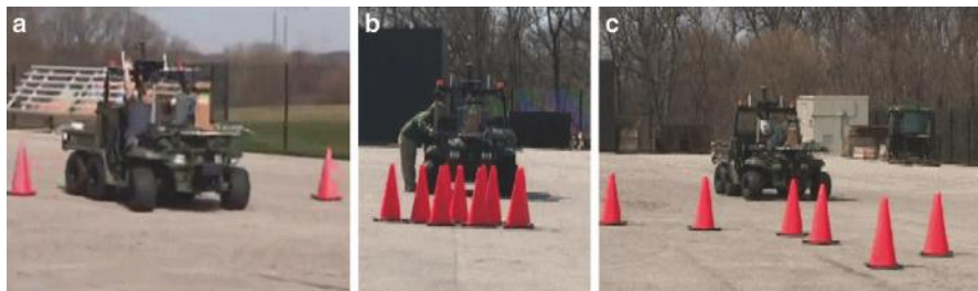
Figure 5.54 Intelligent vehicle performing obstacle avoidance tests
