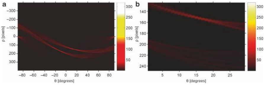
Figure 4.17 Parameter space for the detection of two lines (crop rows inside the ROI)
