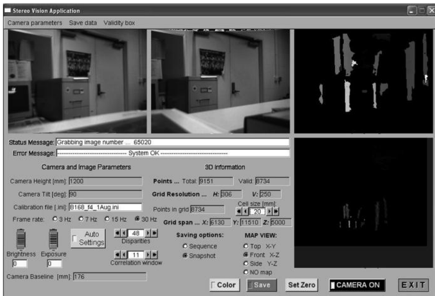
Figure 5.18 Stereo application software for evaluating fundamental camera parameters
