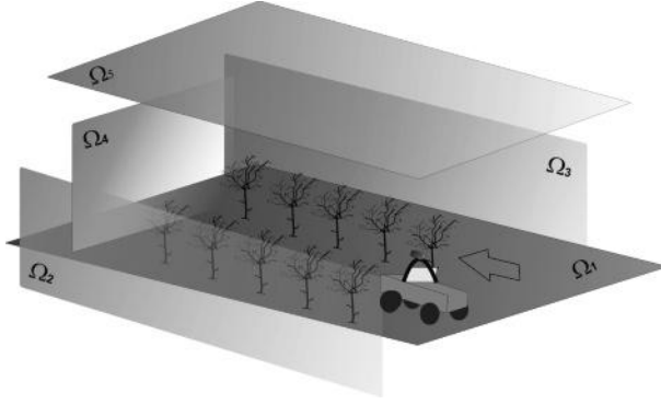
Figure 5.14 Concept of a validity box for filtering out outliers
