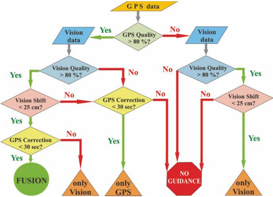
Figure 8.5 Selective fusion algorithm for enhancing autonomous navigation
