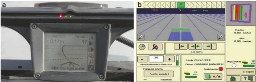
Figure 3.3 GPS-based steering assistance: (a) lightbar system; (b) GUI screen
