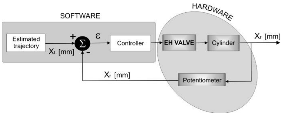
Figure 7.11 Block diagram for the control system of a hardware in-the-loop hydraulic simulator
