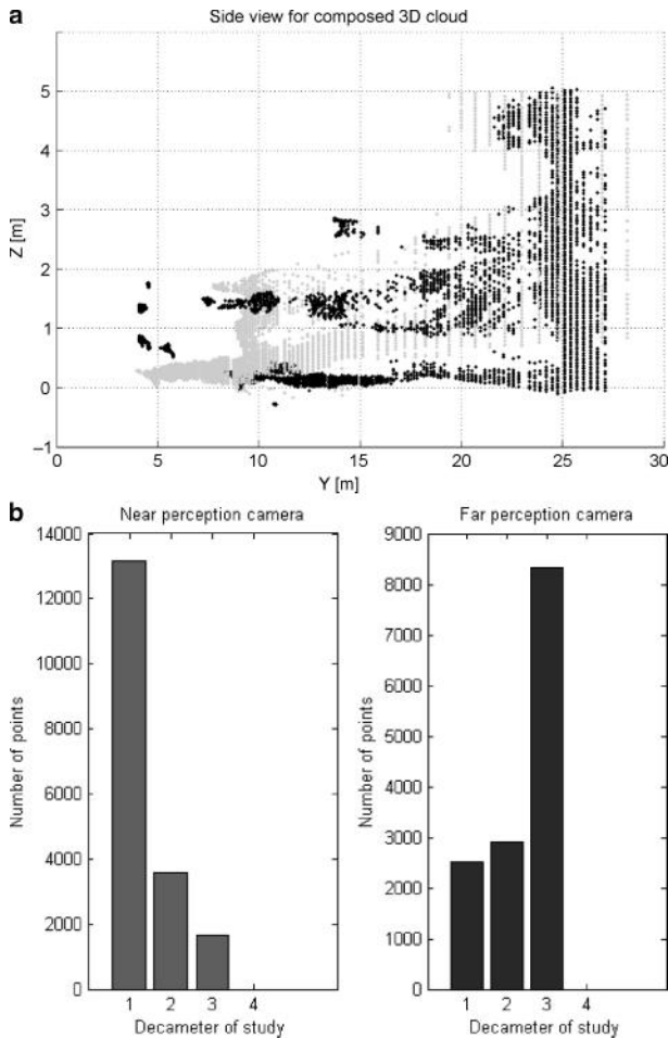
Figure 5.58 Side view (a) and distribution of points (b) for a bifocal camera 3D cloud
