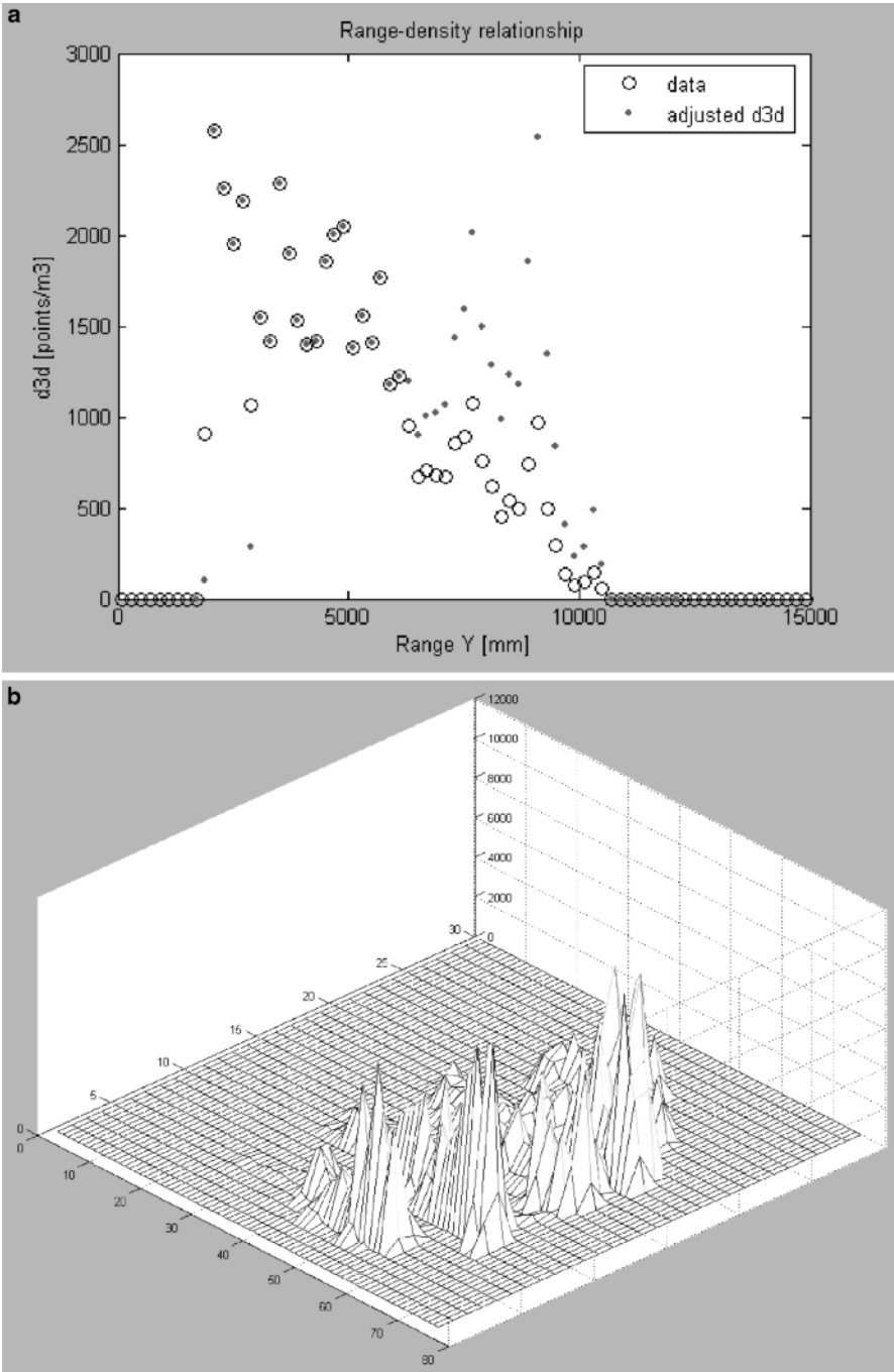
Figure 5.66 Density grid after compensation: (a) range–density relationship; (b) 3D view
