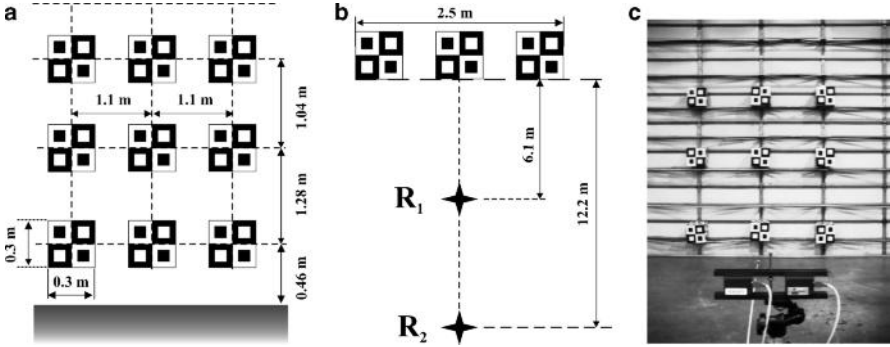
Figure 5.19 Test bench for evaluating the perceptive qualities of stereo cameras
