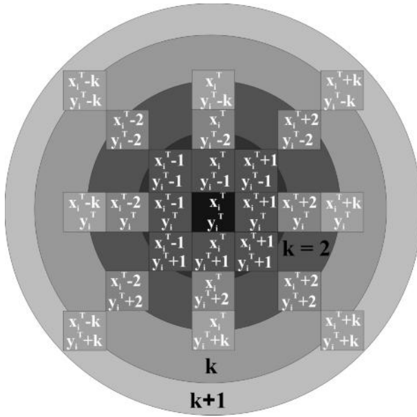
Figure 5.43 Pick-point algorithm used to determine the target point
