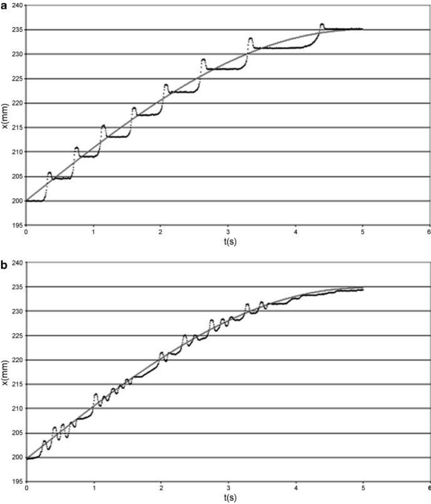
Figure 7.32 Rod positions and input commands (a) with and (b) without deadband compensation (rod stroke: 35 mm, frequency: 0.05 Hz)
