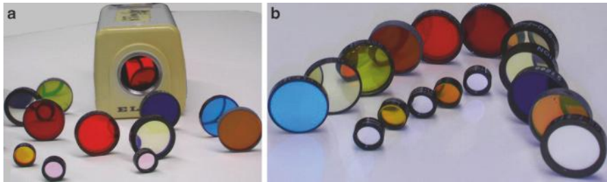
Figure 4.8 IR filters for enhancing agricultural images
