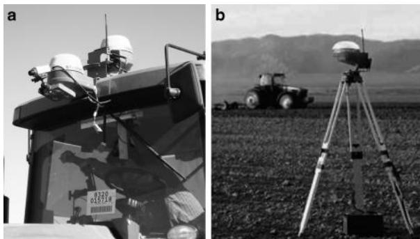
Figure 3.6 RTK-GPS receiver antenna mounted on a wheel-type agricultural tractor (a); base station (b) (courtesy of Deere & Co)
