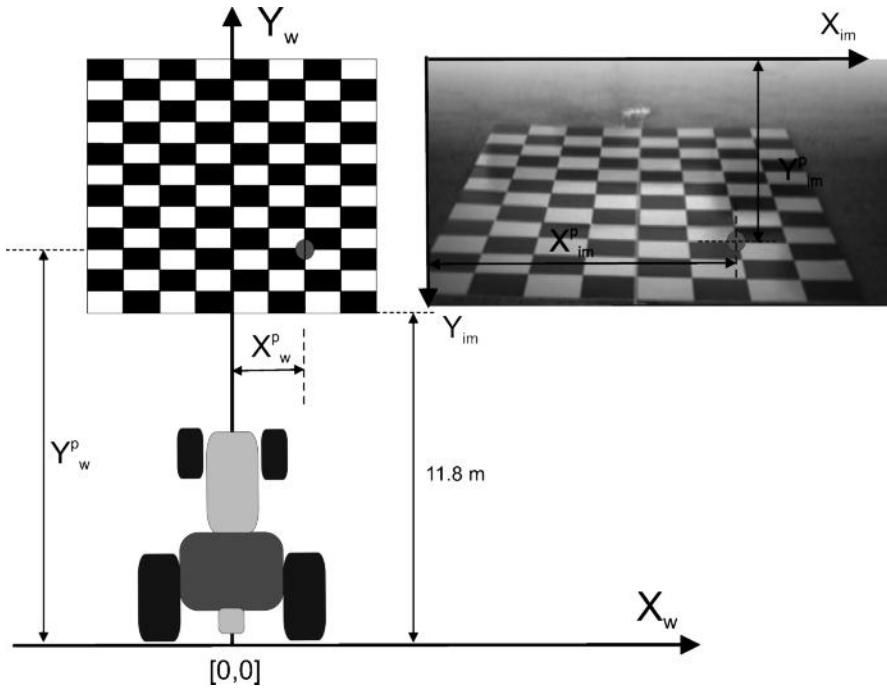
Figure 4.5 Calibration procedure for a monocular camera mounted on an agricultural tractor
