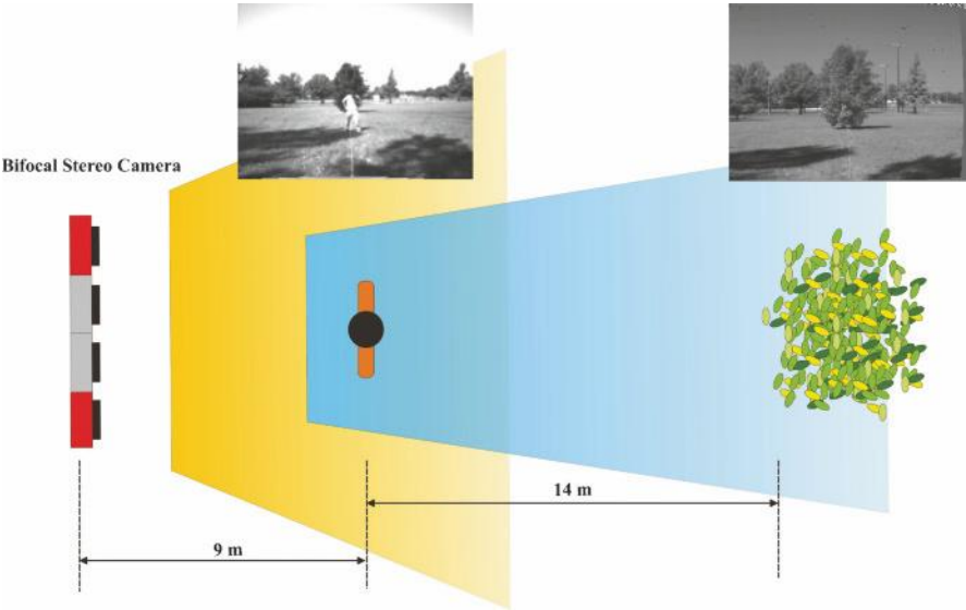
Figure 5.56 Simultaneous object detection at two separated locations with bifocal stereo
