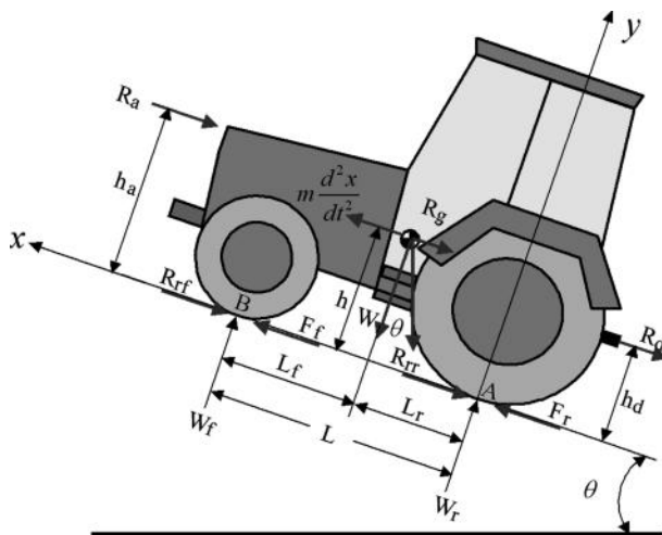
Figure 2.3 Dynamic analysis of a generic off-road vehicle
