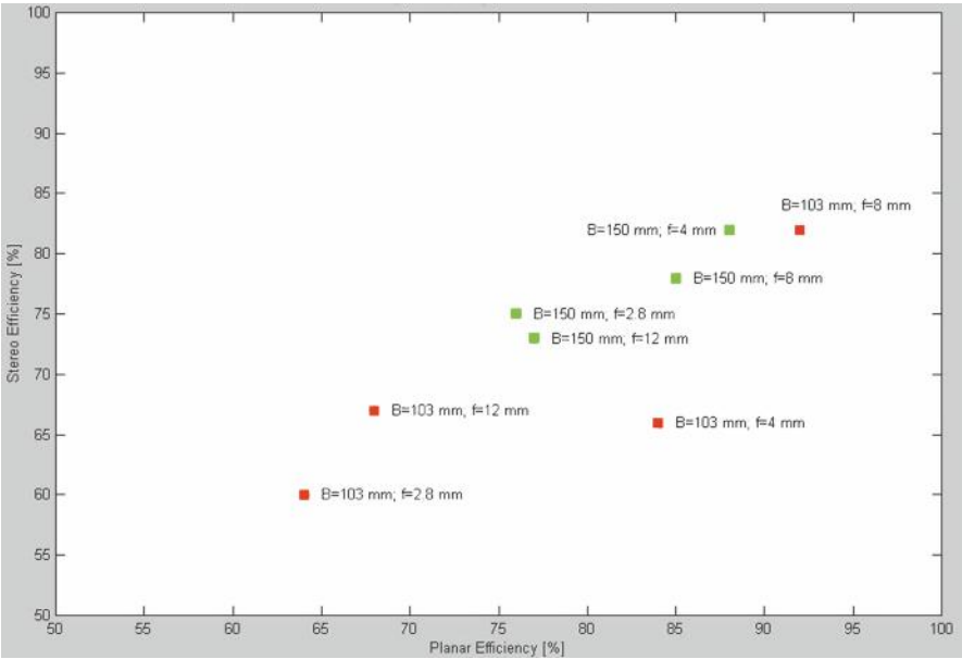
Figure 5.21 Efficiency chart for a range of 6 m
