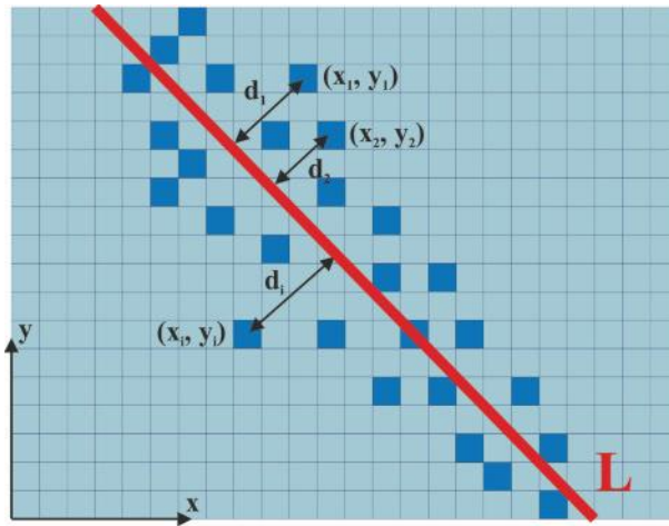
Figure 5.38 Calculation of the moment index M_x
