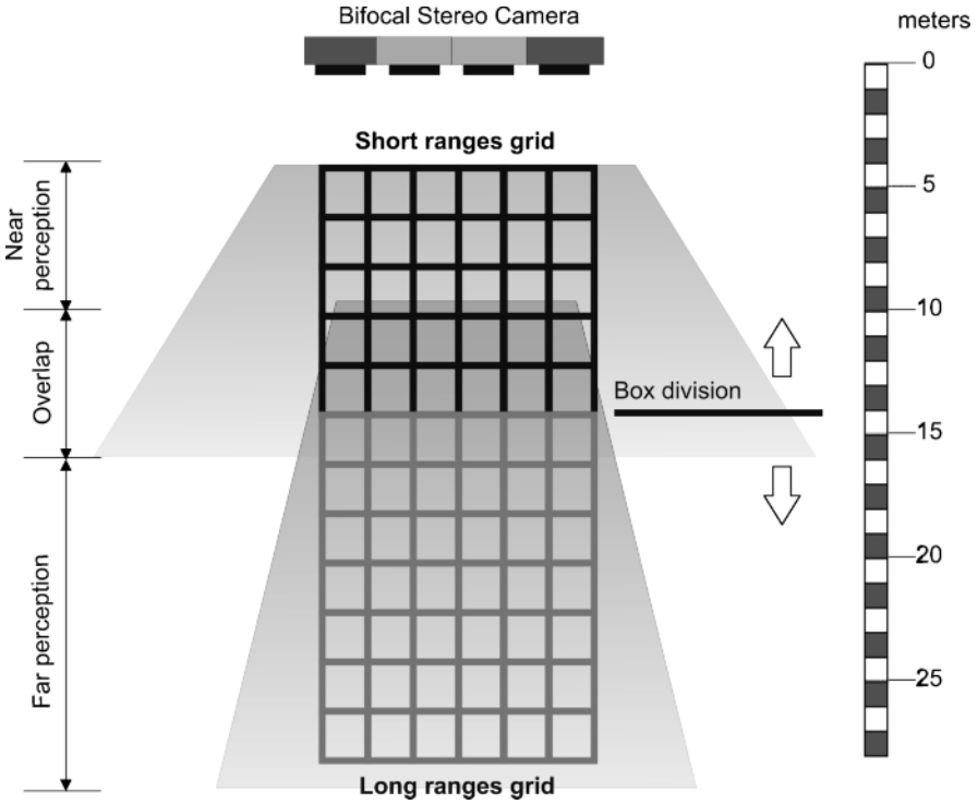
Figure 5.11 Composition of fields of view when expanding stereo perception capabilities
