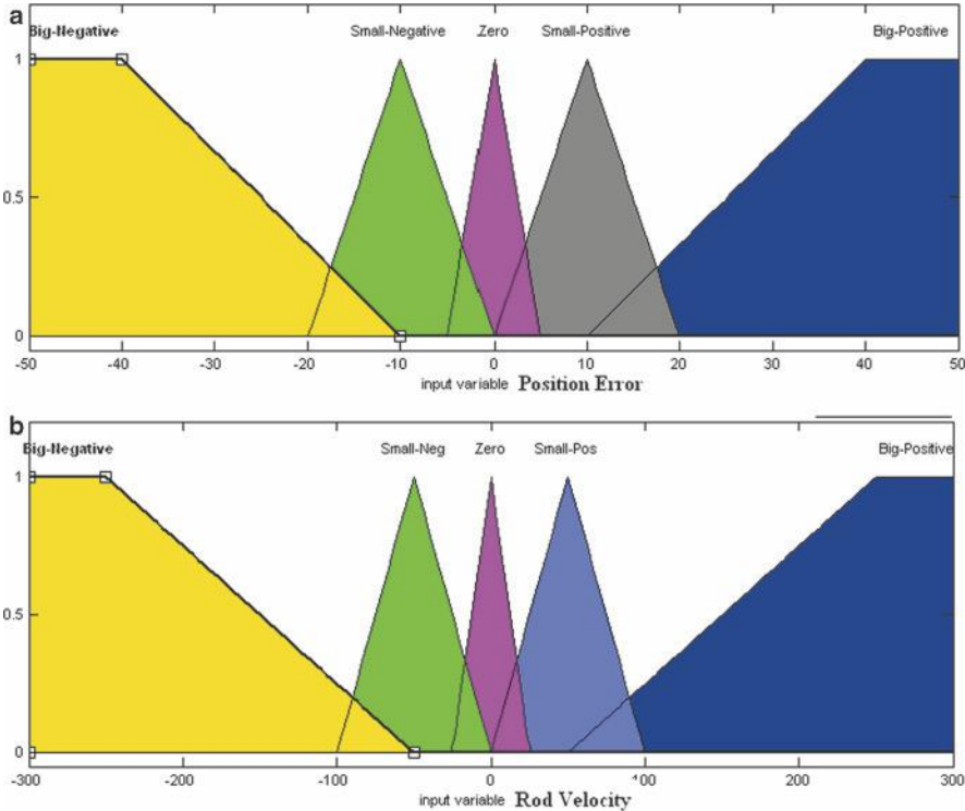
Figure 7.28 Membership functions for input variables of a fuzzy steering controller: (a) the position error \varepsilon ; (b) the rod velocity V
