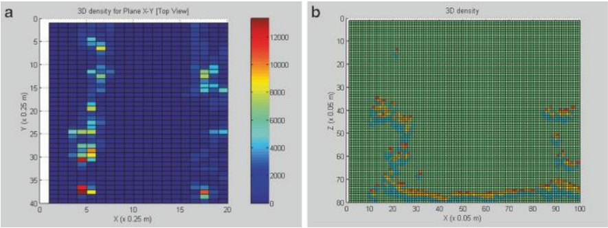
Figure 5.26 Two-dimensional density grids: (a) top-view grid; (b) front-view grid
