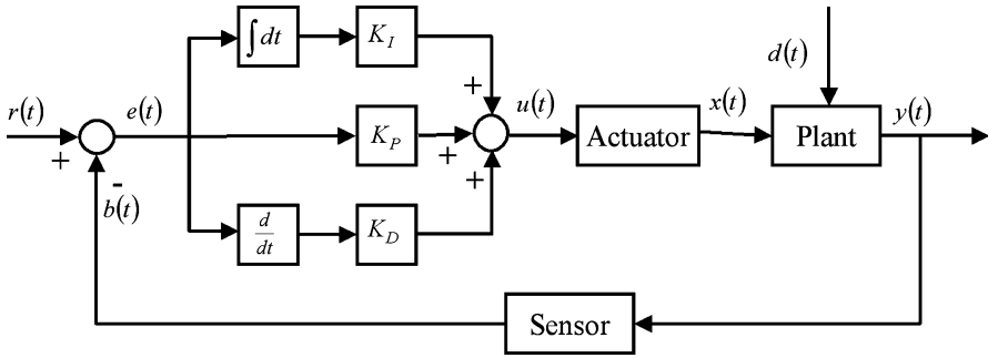
Figure 7.17 Implementation of a PID controller
