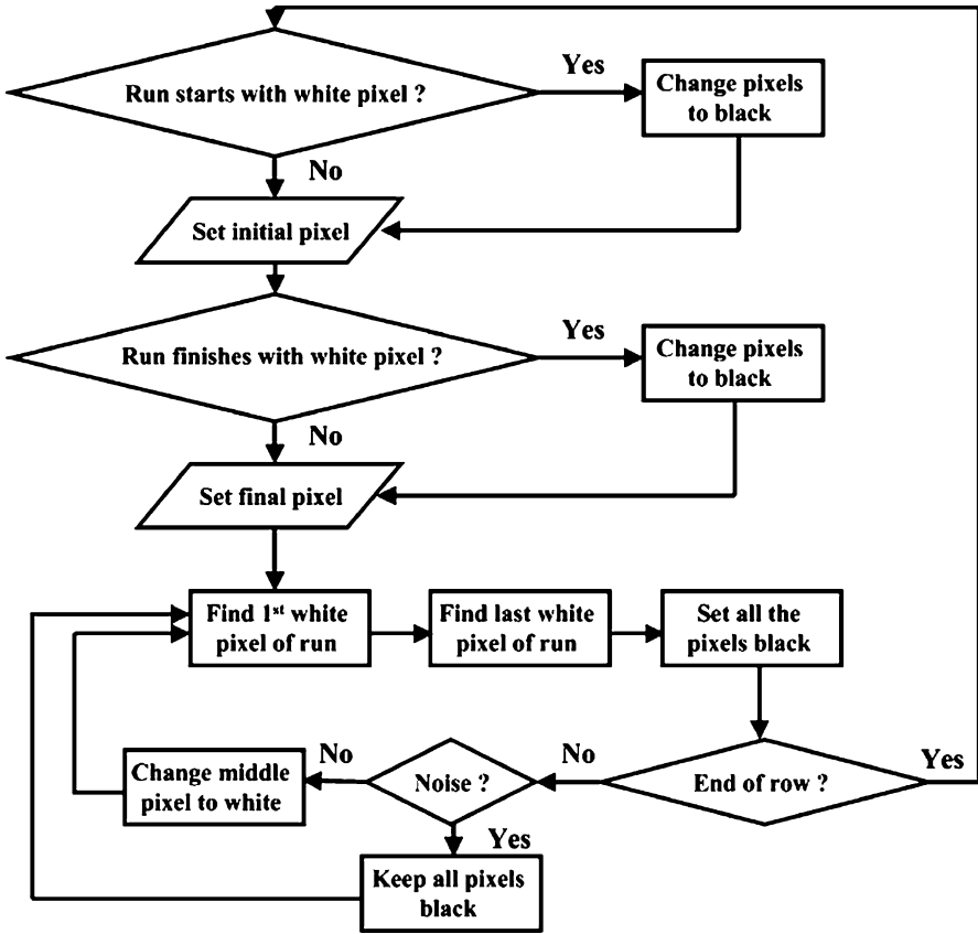
Figure 4.14 Flowchart of the midpoint encoder algorithm
