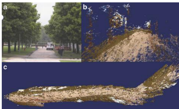
Figure 5.50 Virtual 3D terrain map of a campus scene: (a) photograph of actual scene; (b) 3D global map; (c) field map
