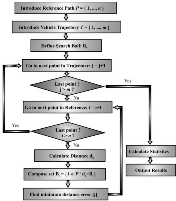
Figure 3.13 Flowchart of the trajectory matching algorithm
