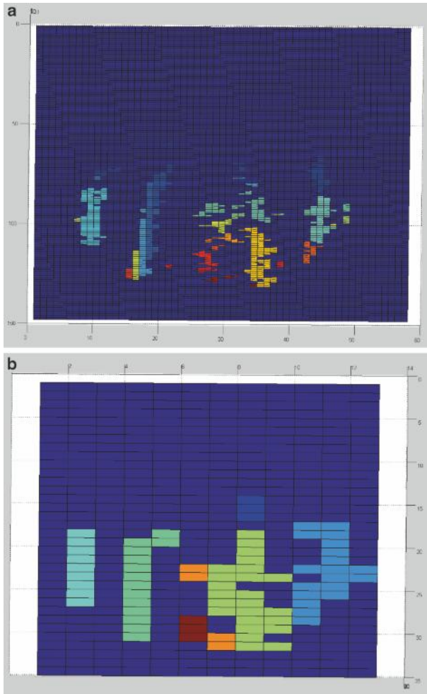
Figure 5.68 Effect of grid resolution on blob analysis: (a) high resolution; (b) low resolution
