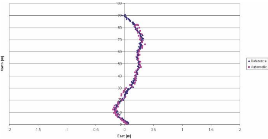
Figure 5.46 System evaluation achieved by comparing manual and automated trajectories
