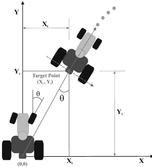
Figure 8.6 Basic methodology used to estimate steering commands
