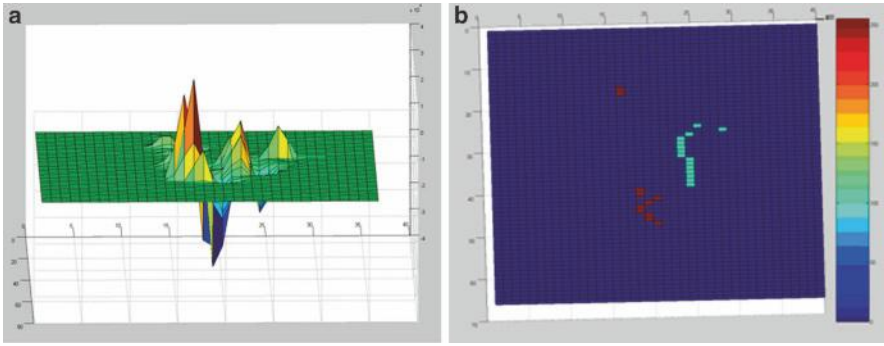
Figure 5.37 Edge enhancement by the application of a gradient mask: (a) 3D view; (b) 2D map
