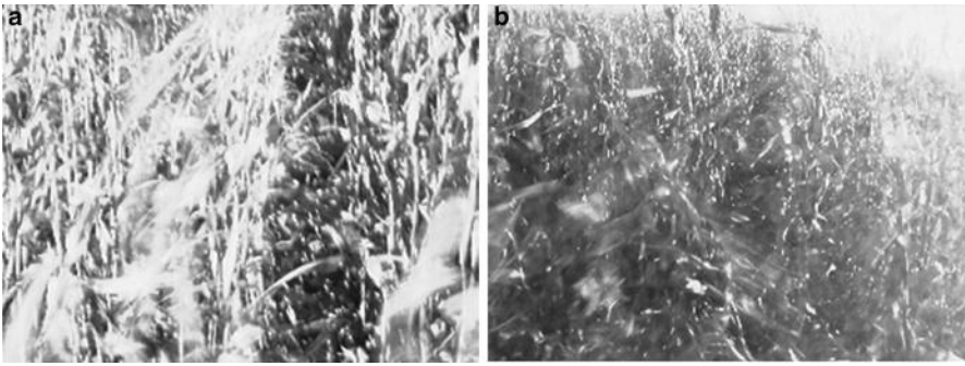
Figure 4.24 Images with difficult illumination for machine vision guidance
