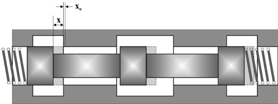
Figure 7.8 Operating principles of spool valves
