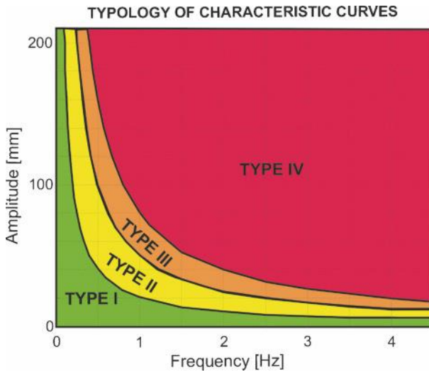
Figure 7.26 Typology chart for characteristic curves of EH valves
