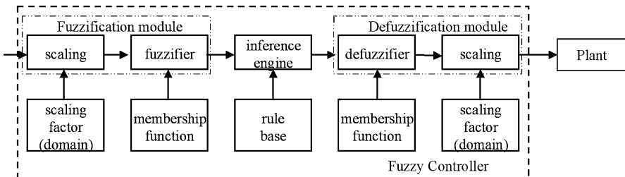
Figure 7.20 Overall structure of a fuzzy controller
