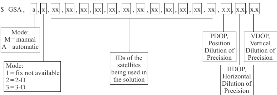
Figure 6.4 Specifications for GSA NMEA messages
