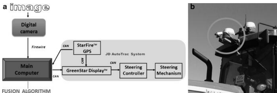
Figure 4.32 System architecture: (a) block diagram; (b) local and global sensors
