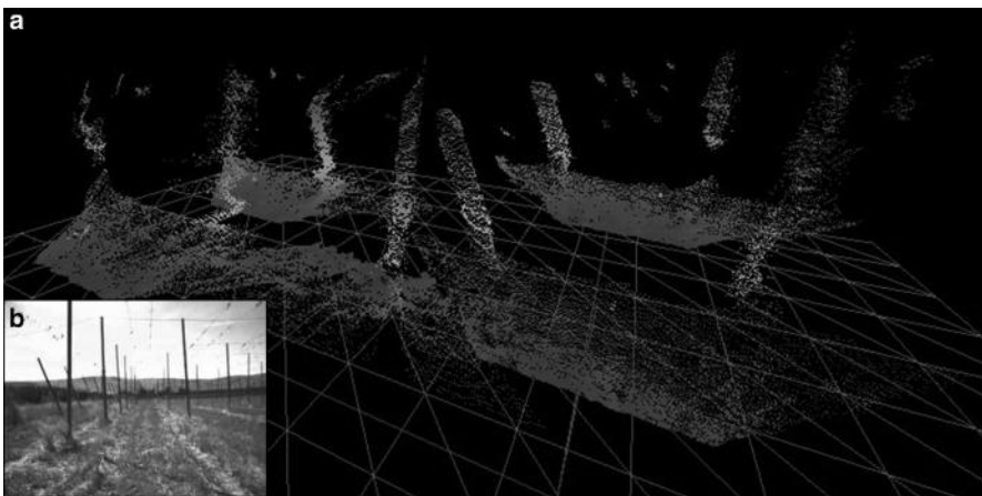
Figure 5.49 Virtual 3D global map (a) of a barren field with crop-supporting structures (b)
