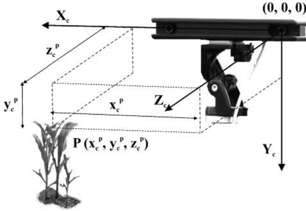
Figure 5.4 Definition of camera coordinates for binocular stereo sensors
