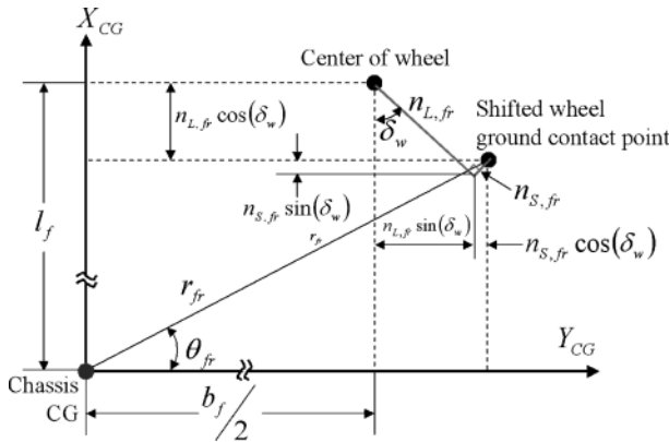
Figure 2.11 Calculation of the distance between the CG and the WGCP for the front right wheel
