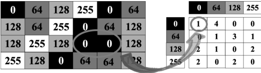
Figure 4.20 Construction of the gray-level co-occurrence matrix (GLCM)
