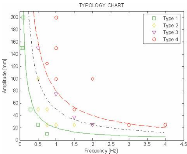
Figure 7.24 Frequency–amplitude chart for a hydraulic steering cylinder
