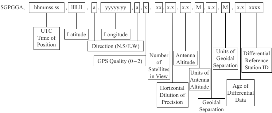
Figure 6.3 Specifications for GGA NMEA messages
