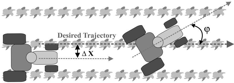
Figure 4.33 Principal navigation errors for intelligent vehicles: offset ( \Delta X ) and heading ( \phi )
