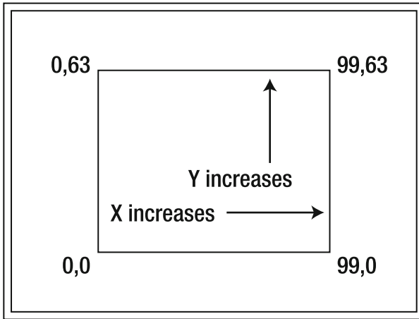
Figure A-3. The Brick's LCD screen's X/Y coordinate system
