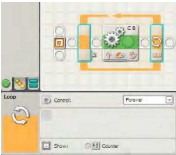
Figure 11-7. A LOOP block set to Forever
