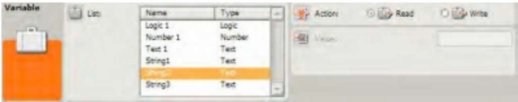
Figure 19-9. The fifth VARIABLE block's configuration panel
