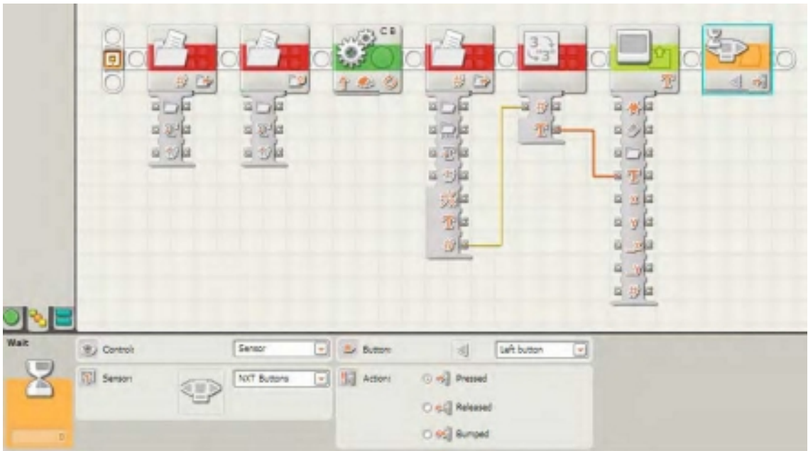
Figure 22-6. Read the value stored in the file.
