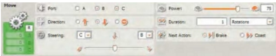
Figure 5-11. The second MOVE block's configuration panel
