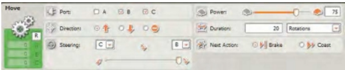
Figure 6-17. The MOVE block's configuration panel
