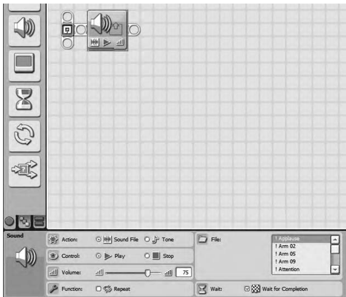
Figure 6-1. The SOUND block's configuration panel
