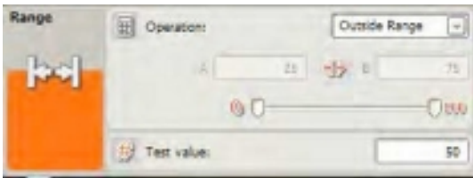
Figure 16-19. The RANGE block's configuration panel
