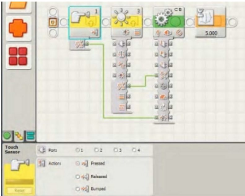
Figure 8-7. The complete program and the Touch sensor's configuration panel
