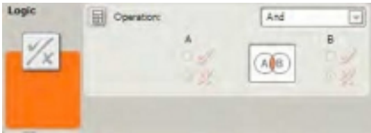
Figure 17-14. The LOGIC block's configuration panel
