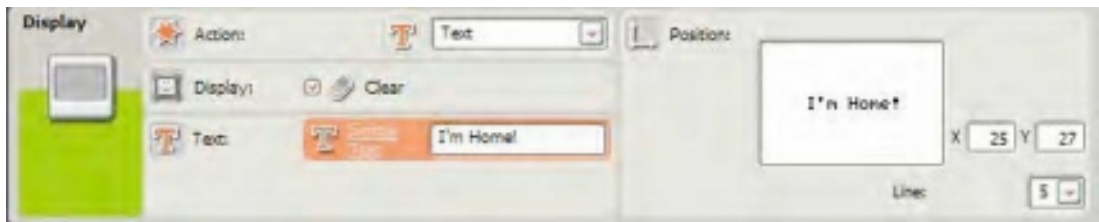
Figure 4-13. The DISPLAY block configuration panel
