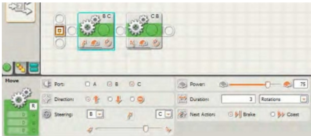
Figure 4-15. The complete program and the first MOVE block's configuration panel
