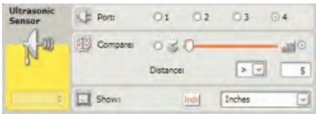
Figure 9-20. The Ultrasonic sensor block's configuration panel
