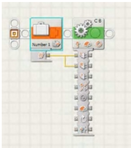
Figure 7-12. Data wires can be split and provide the same data to more than one port.
