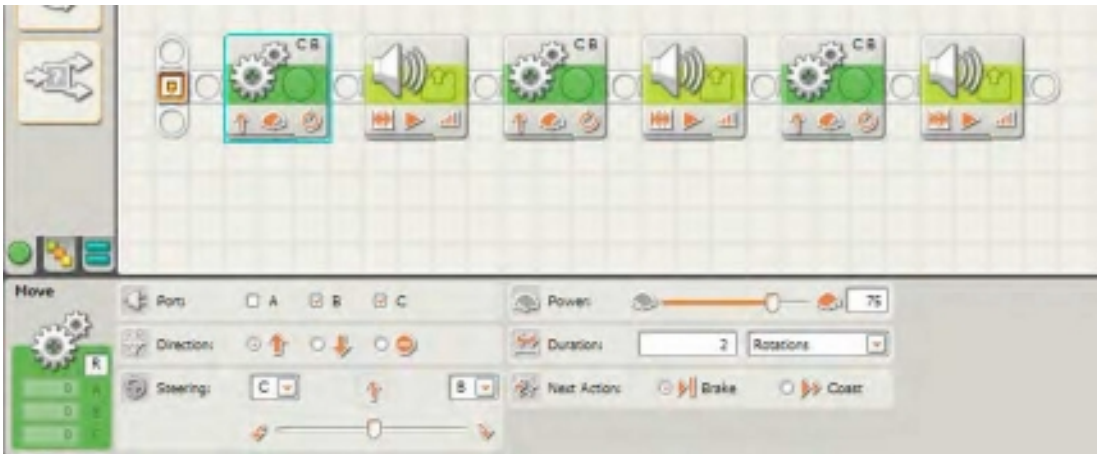
Figure 6-18. The complete program and the first MOVE block's configuration panel
