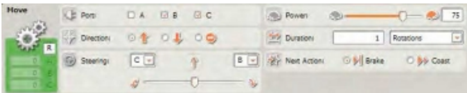
Figure 5-13. The third MOVE block's configuration panel
