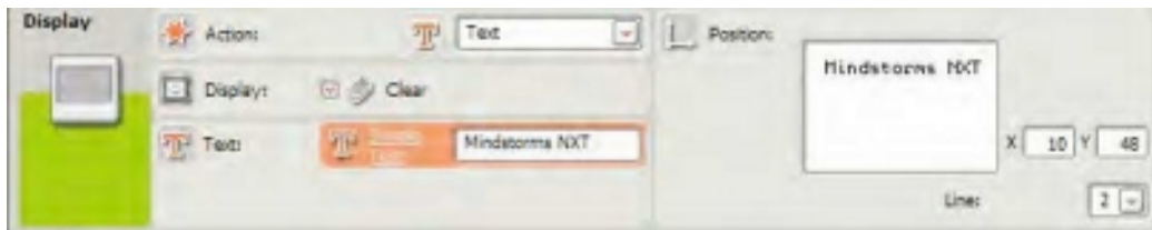
Figure 16-17. The first DISPLAY block's configuration panel
