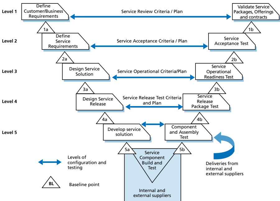
Figure 5.4 The service V model (Based on: OGC source) Copyright protected. Use is for Single Users only via a VHP Approved License. For information and printed versions please see www.vanharen.net
