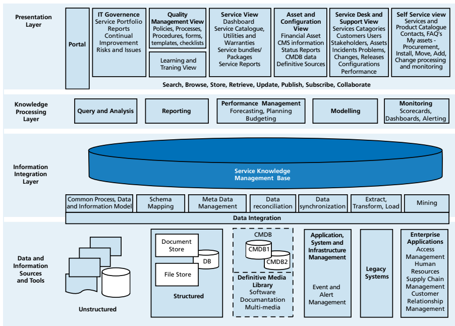
Figure 5.7 The Service Knowledge Management System (SKMS) (Based on: OGC source)
