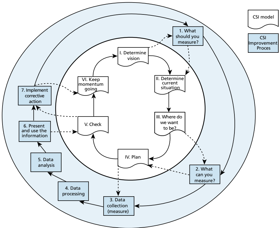
Figure 7.3 Connections between CSI Model and the CSI Improvement process (Based on: OGC source)
