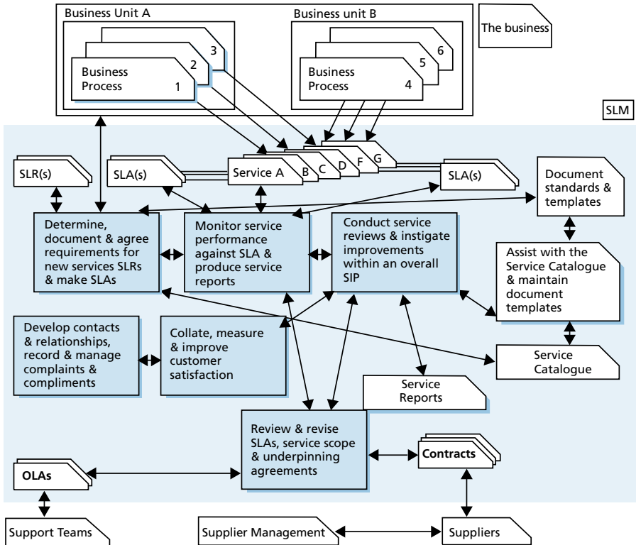
Figure 4.2 Service level management (Based on: OGC Source)
