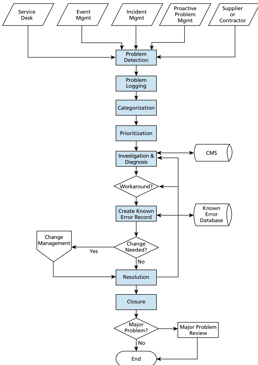
Figure 6.3 Problem management (Based on: OGC source)
