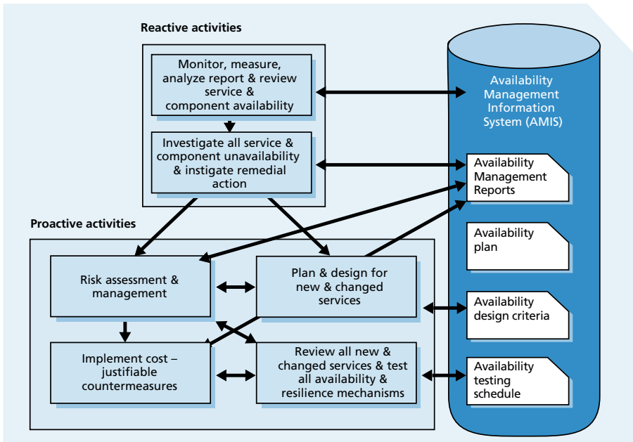
Figure 4.6 Availability management (Based on: OGC source)
