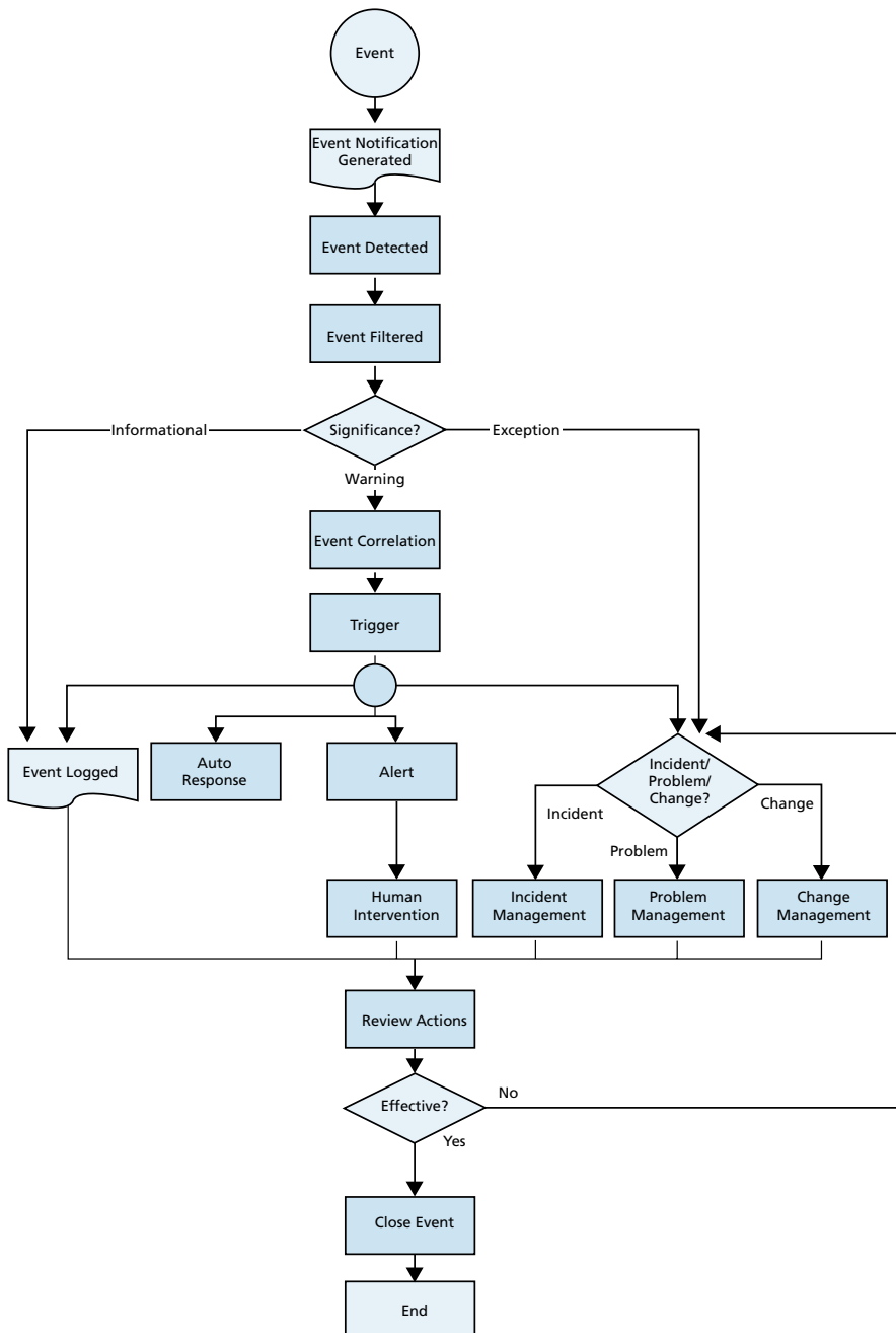
Figure 6.1 Event management (Based on: OGC source)
