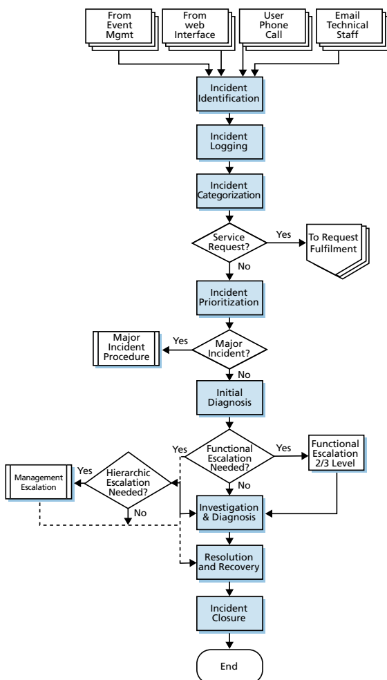
Figure 6.2 Incident management (Based on: OGC source)
