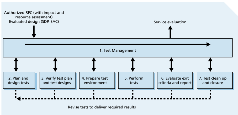
Figure 5.5 Service validation and testing (Based on: OGC source)
