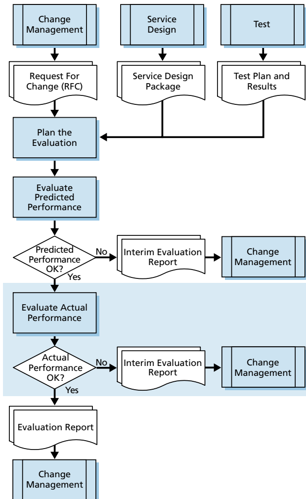
Figure 5.6 Evaluation (Based on: OGC source)
