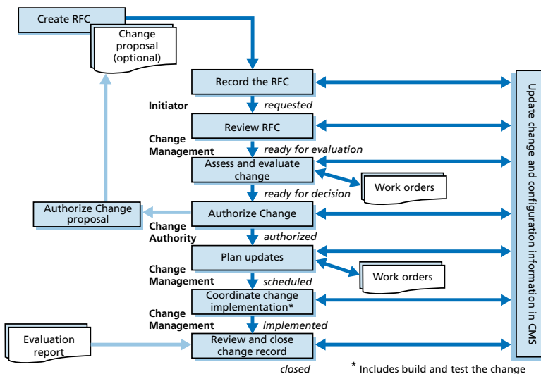
Figure 5.1 Change management (Based on: OGC source)
