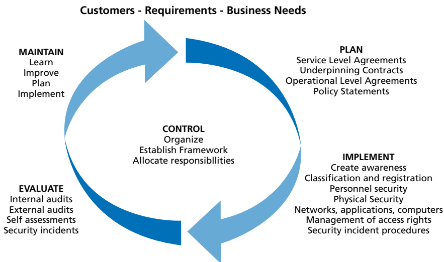
Figure 4.8 Framework for managing IT security (Based on: OGC source)
