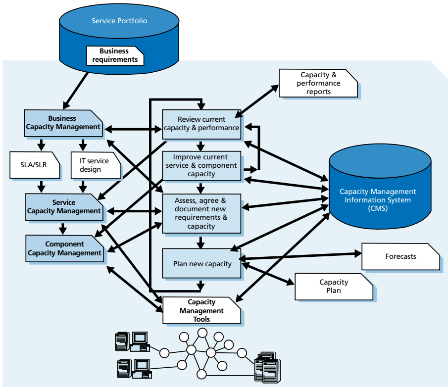
Figure 4.4 Sub-processes of capacity management (Based on: OGC source)
