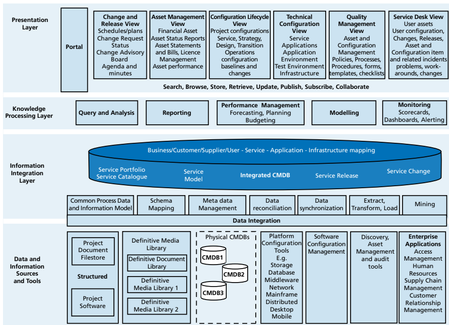
Figure 5.3 Example of a CMS (Based on: OGC source)
