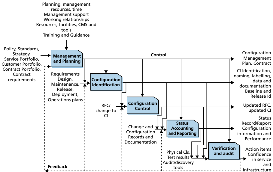
Figure 5.2 Service asset and configuration management (Based on: OGC source)
