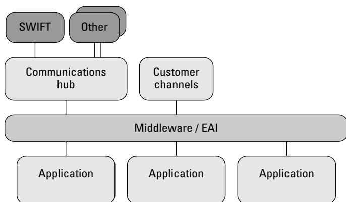
Figure 2-3: Enterprise Application Integration software (middleware) connects applications to each other and to external networks such as SWIFT.
