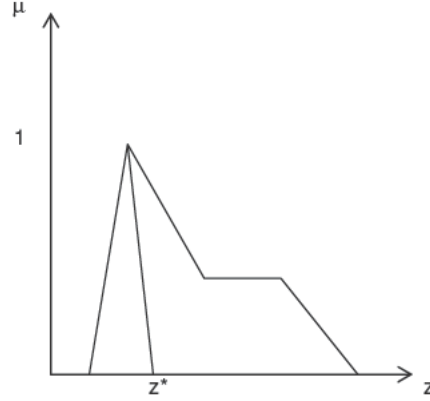
Fig. 5.2. Max-membership method
