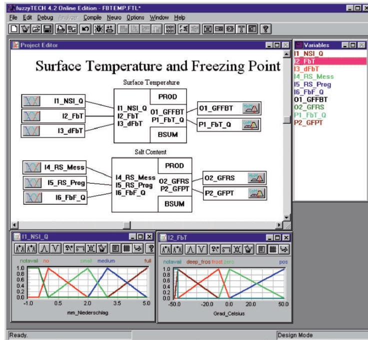
Fig. 8.45. Road temperature fuzzy logic module
