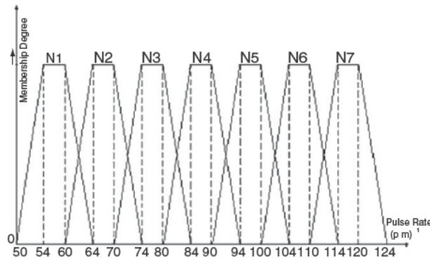
Fig. 8.26. Membership of pulse rate
