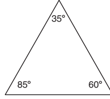
Fig. 4.7. A given triangle
