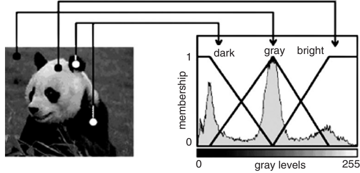
Fig. 8.15. Histogram fuzzification
