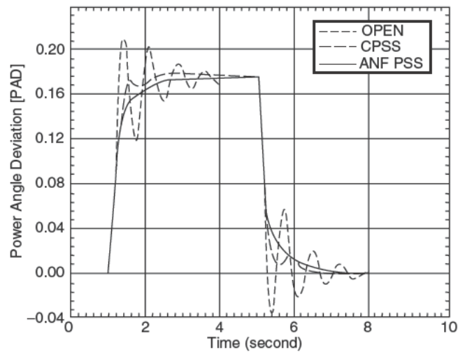
Fig. 8.115. Response curve
