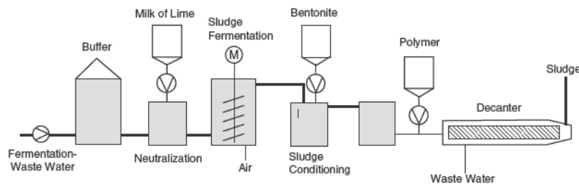
Fig. 8.53. Process diagram of sludge draining
