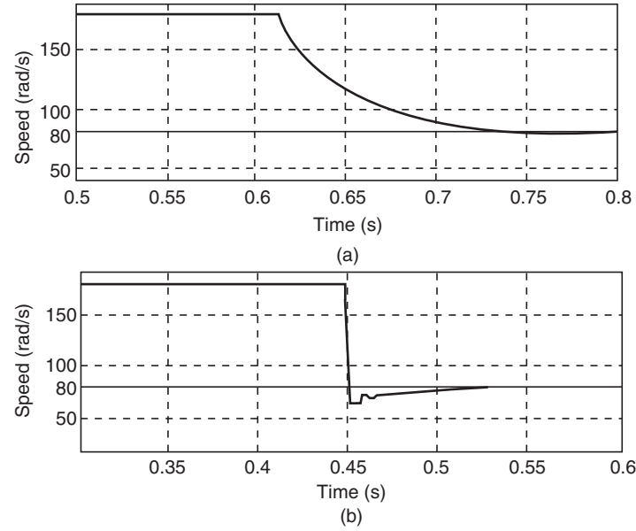
Fig. 9.6. Speed change from 180 to 80 rad s -1 : (a) without feeding and (b) feeding the phase with decreasing inductance
