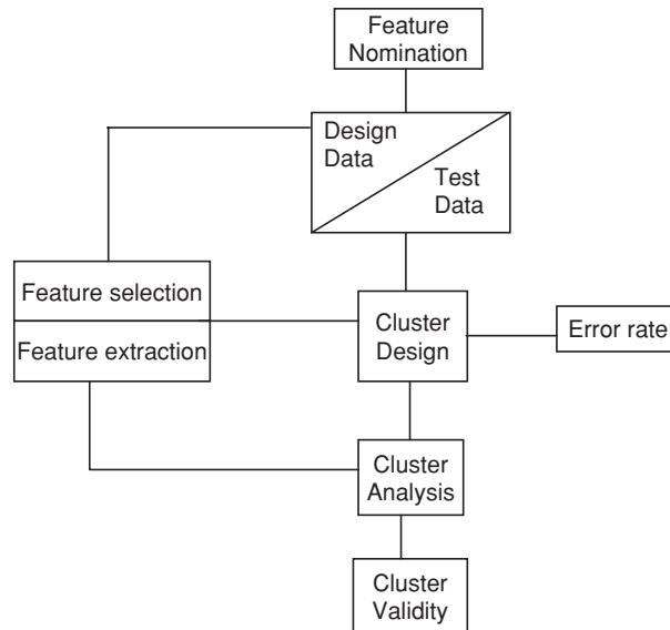
Fig. 8.135. Block diagram of fuzzy pattern recognition
