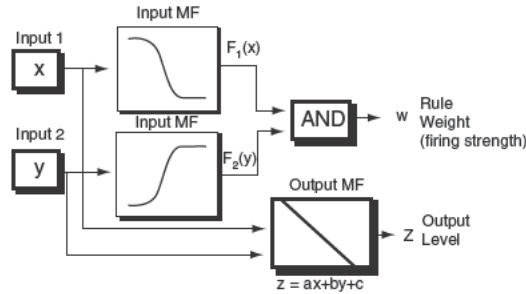
Fig. 6.6. Sugeno rule
