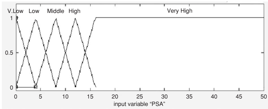
Fig. 8.103. Membership function of PSA
