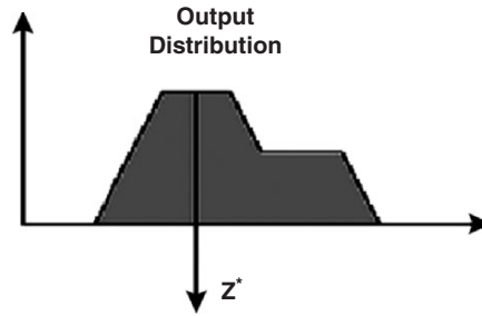
Fig. 6.4. Defuzzification using the mean of maximum
