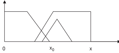
Fig. 8.137. Data sample resemblance
