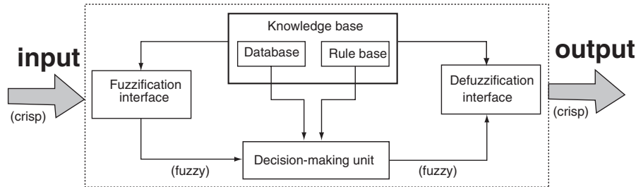
Fig. 6.1. Fuzzy inference system
