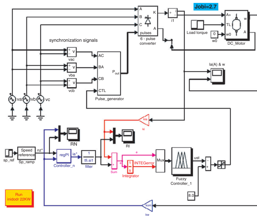
Fig. 9.13. DC drive with fuzzy controller in current loop. PSB is used to build advanced drive model ( upper part of block diagram )
