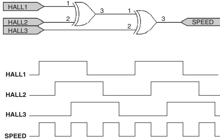
Fig. 9.39. The speed pulse multiplexer
