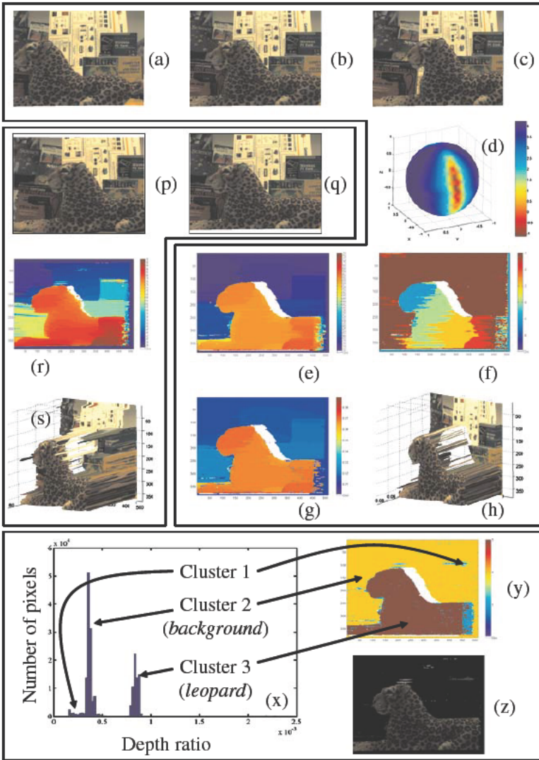
Fig. 12.12. Class 3: (a,b,c) show three frames F_1, F_2, F_3 of the leopardB sequence. (d) shows the computed motion valley. (e,f) show X and Y components of the flow u_{23} between F_2 and F_3 . White regions denote occlusions. (g) shows inverse depth from motion. (h) shows 3D structure from motion. (p,q) show rectified stereo pair of images. (q) is the same as (b). (r) shows inverse depth from stereo. (s) shows 3D structure from stereo. Compare (s) with (h) to see how the background objects appear closer to the leopard in (s) than in (h). (x) shows the histogram of depth ratios and clusters detected by k -means ( k=3 ). (y) shows cluster labels: cluster 2 (yellow) is the background, cluster 3 (red) is the leopard, cluster 1 (light blue) is mostly due to errors in the disparity and flow. (z) shows the moving objects of Class 3 (clusters other than 2) (Reproduced from [1] with permission © 2004 IEEE)
