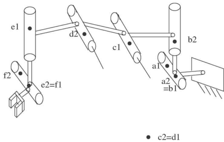
Fig. 19.7. A robot arm of six joints
