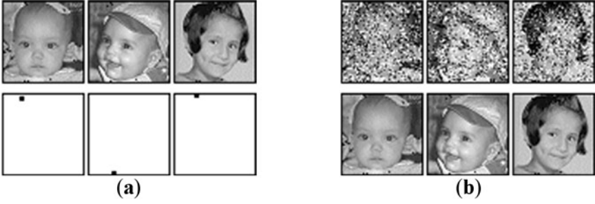
Fig. 4.4. In (a) the top row shows the lattice-independent patterns and the bottom row shows the corresponding nonzero entries in matrix Z used as a minimal representation or kernel. In (b) the top row contains the input patterns corrupted with random noise, while the bottom row illustrates perfect recall using the kernel Z for the memory scheme M_{ZZ} \rightarrow W_{XX} (also the output of memory W_{ZX} )
