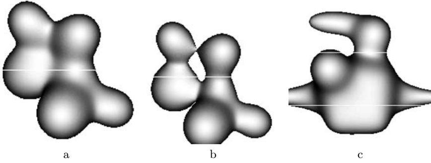
Fig. 18.9. a Equipotential. b Higher threshold. c Other potentials
