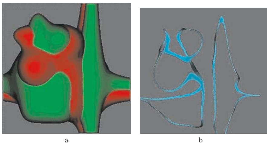
Fig. 18.10. a Union of boundaries of equipotential and b intersection of boundaries
