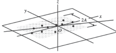
Fig. 14.4. Fitting a space line and a plane to points in space
