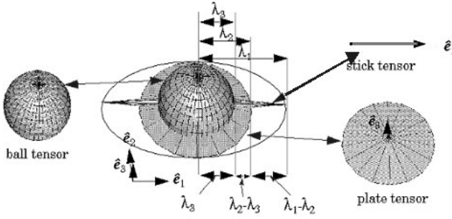
Fig. 16.1. second-order generic tensor and its decomposition into the stick , plate and ball components in 3-D
