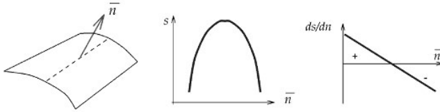
Fig. 16.4. Dense surface extraction in 3-D: ( Left ) Elementary surface patch with normal \mathbf{n} . ( Center ) 3-D surface saliency along normal direction ( Right ) First derivative of surface saliency along normal direction
