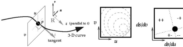
Fig. 16.5. Dense curve extraction in 3-D: ( Left ) 3-D curve with tangent \mathbf{t} and the normal plane. ( Center ) Curve saliency isocontours on the normal plane. ( Right ) First derivatives of surface saliency on the normal plane
