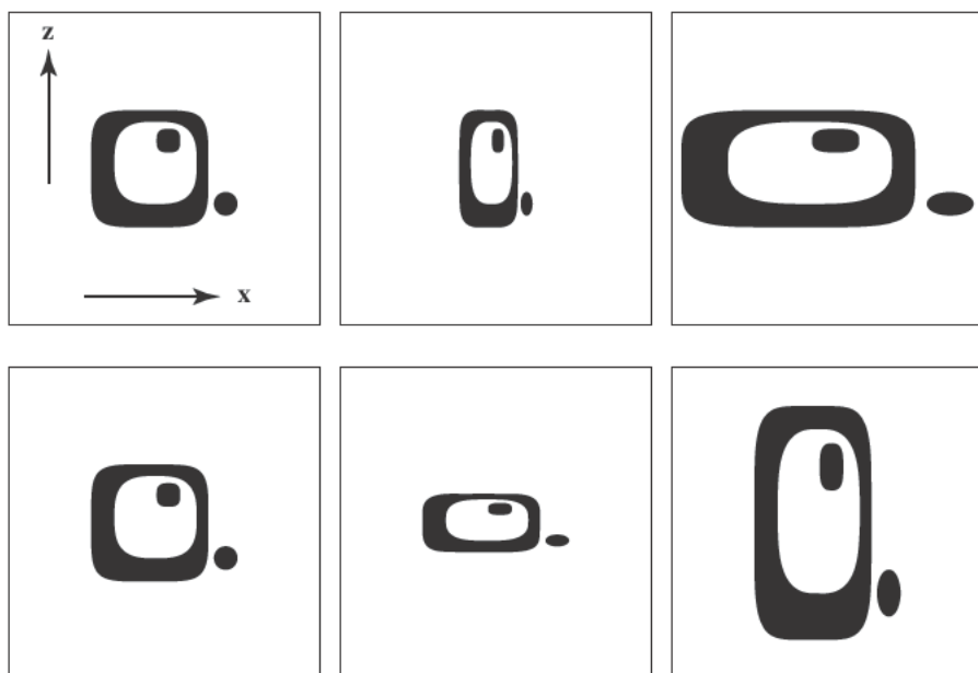
Fig. 6.7. Two types of similarities in \mathbb{I}^2 , in the top row those “of the first-kind” which affect distances and in the bottom row those “of the second-kind” which affect the angles
