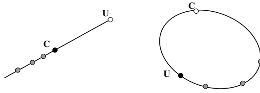
Fig. 9.14. (left) The intersection ambiguity where a point U and several camera centres C lie on a line. (right) The dual resection ambiguity where a camera centre C and several points U lie on a conic curve
