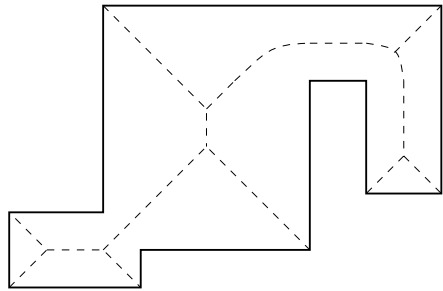
Fig. 23.13. The medial axis of a polygonal region
