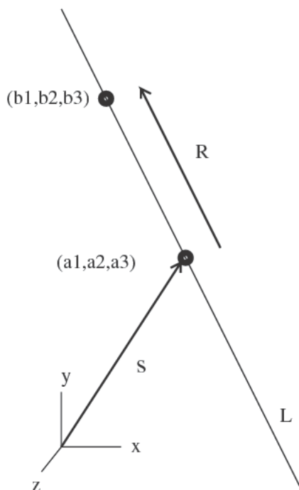
Fig. 19.1. A line in 3-space
