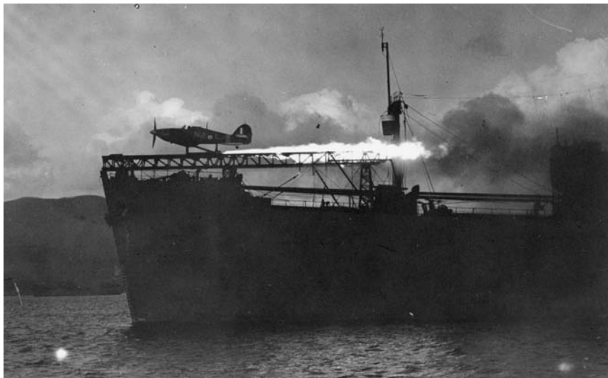
A test launch of a Hurricane from a CAM ship on the Clyde in October 1941. If an alert Condor's crew spotted the brilliant flame of the rocket launch, it could give the Fw 200 time to escape into nearby clouds before the British fighter could intercept. [Imperial War Museum A 9423]
