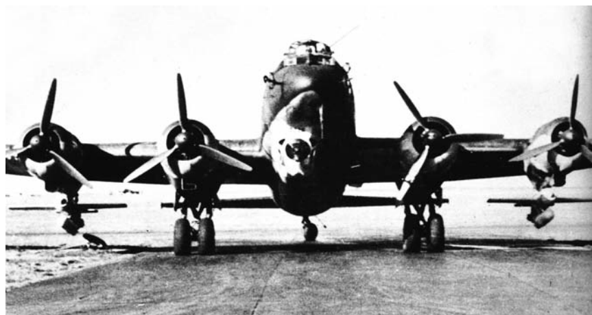
The final version of the Condor, the Fw 200 C-8, could carry two Hs-293 guided bombs. However, by the time that it was operational in December 1943 the Condor was too vulnerable to remain in front-line service. [Author's collection]
