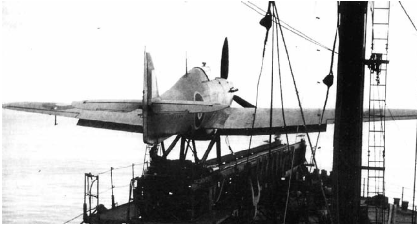
A Hurricane pilot would have to climb a 9m (30ft) ladder in order to reach the Hurricane's cockpit, and then he would sit in the cockpit for a two-hour shift. The catapult was angled toward the starboard bow and the fighter sat atop a trolley that was propelled forward by a series of 3-inch rockets. (Author's collection)
