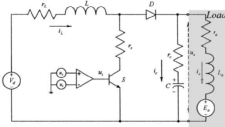
Figure 5.15. High-frequency switching converter
