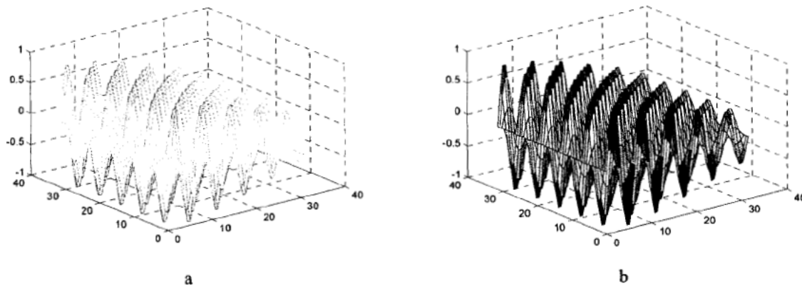
Figures 4.26. Three-dimensional plots
