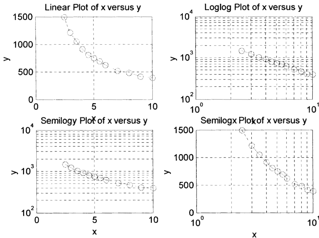
Figure 4.32. Plots
