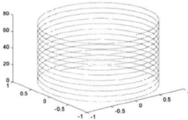
Figure 4.17. Three-dimensional plot
