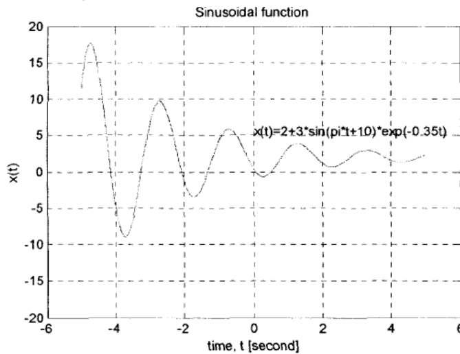
Figure 4.28. Plots of functions x(t) = 2 + 3 \sin(\pi t + 10)e^{-0.35t}
