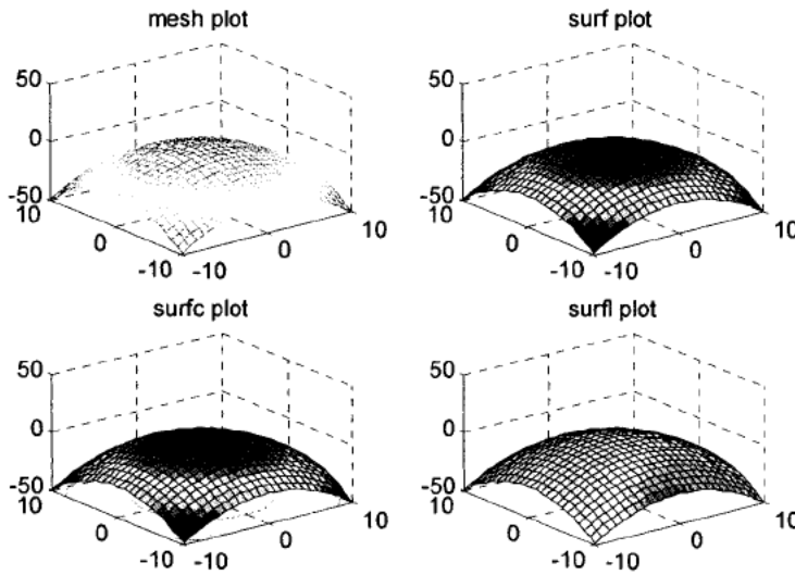
Figure 4.21. Plot of z(x,y) = 1 - \frac{1}{4}x^2 - \frac{1}{4}y^2 if -10 \leq x \leq 10 and -10 \leq y \leq 10 □
