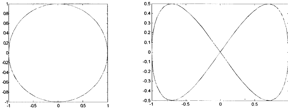
Figure 4.24. Movie frames
