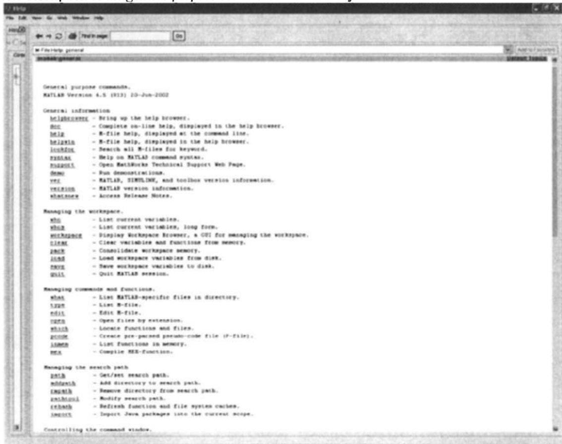
Figure 2.3. Help Window
