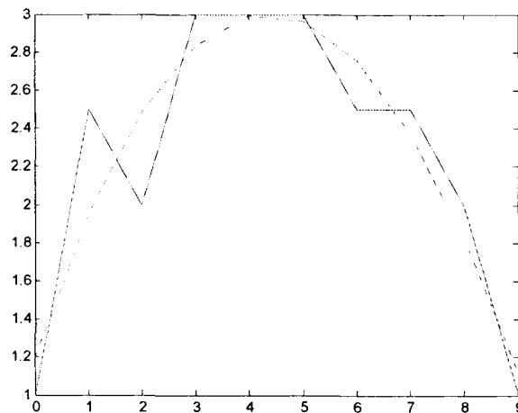
Figure 3.11. Plots of the xy data ( x = [0 \ 1 \ 2 \ 3 \ 4 \ 5 \ 6 \ 7 \ 8 \ 9] and y = [1 \ 2.5 \ 2 \ 3 \ 3 \ 3 \ 2.5 \ 2.5 \ 2 \ 1] ) and its approximation by p(x) = 0.001x^3 - 0.104x^2 + 0.8478x + 1.2028
