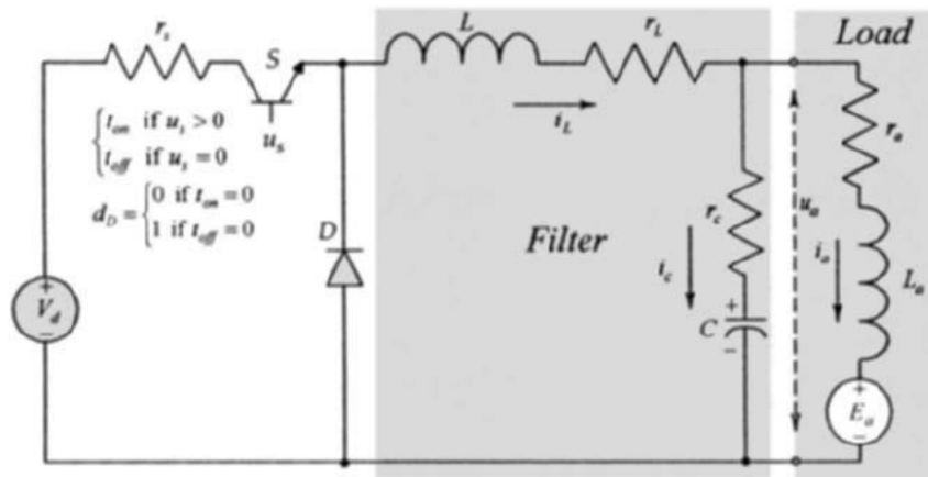
Figure 5.12. Switching converter
