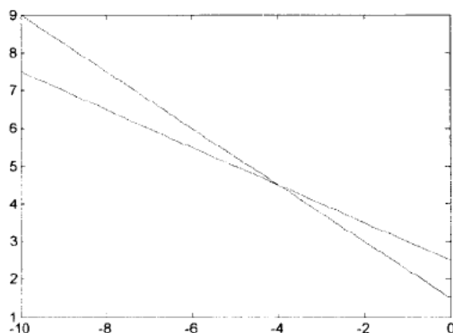
Figure 3.10. Graphical solution of the system of linear equations y + 2z = 5 and 3y + 4z = 6
