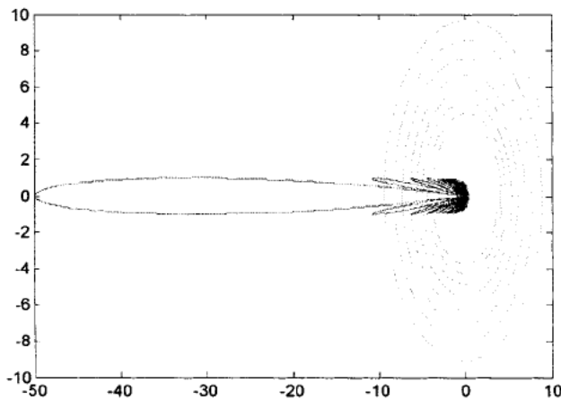
Figure 4.15. Functions plots
