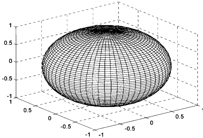
Figure 4.22. Three-dimensional sphere
