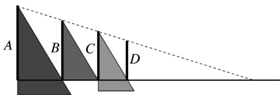
Eratosthenēs’ mechanical method of finding two mean proportionals between magnitudes A and D . The left and right triangles are slid along grooves until by trial and error the four vertices are collinear © Jones
