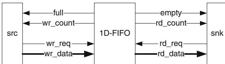
Fig. 5.9 Principle of one-dimensional FIFO communication
