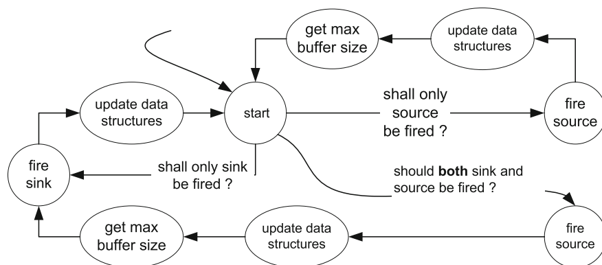
Fig. A.8 Simulation state diagram for a single WDF edge
