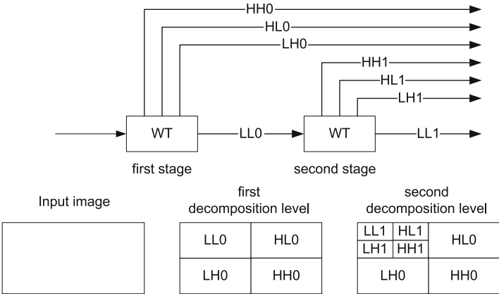
Fig. 2.2 Wavelet transform
