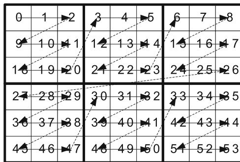
Fig. 5.8 Code-block forming in JPEG2000. Arabic numbers describe the production order of the wavelet coefficients while the arrows depict the read order of the BB. a WDF graph. b WT and BB invocation order
