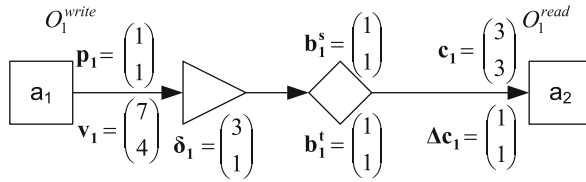
Fig. 5.1 WDF graph with two actors and a single edge for illustration of the introduced notation
