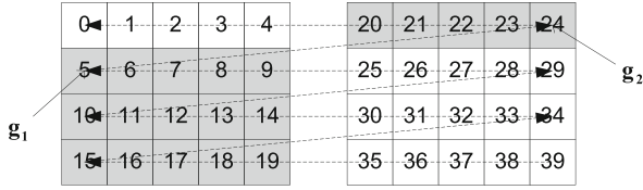
Fig. 6.7 Worst-case distribution of live data elements for the inverse tiling operation and sequential ASAP scheduling. Arabic numbers depict the production order while the dashed arrows represent the read order
