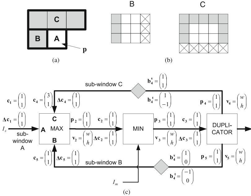
Fig. 5.19 a Irregular window and c its realization in WDF. b shows the border processing assuming an input image size of 3 \times 3 pixels. \mathbf{p} refers to the currently processed pixel (see Eq. (5.11)). Crossed data elements are suppressed
