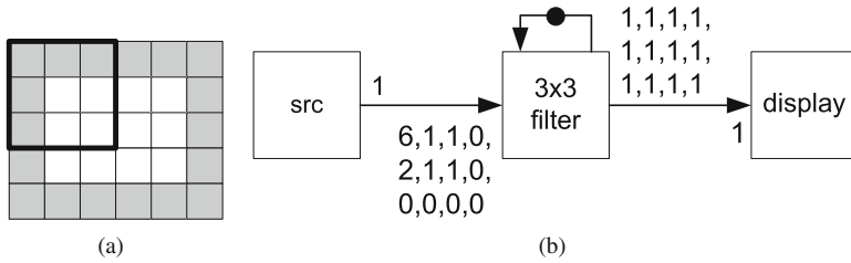
Fig. 3.3 CSDF model applied to a sliding window application. a Sliding window algorithm. b CSDF graph
