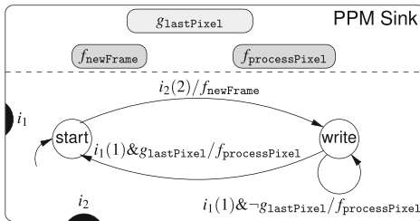
Fig. 4.3 Depiction of the PPM Sink actor from Fig. 4.2 along with the source code of the action f_{\text{newFrame}} . The transitions of the state machine are annotated with activation pattern/action pairs
