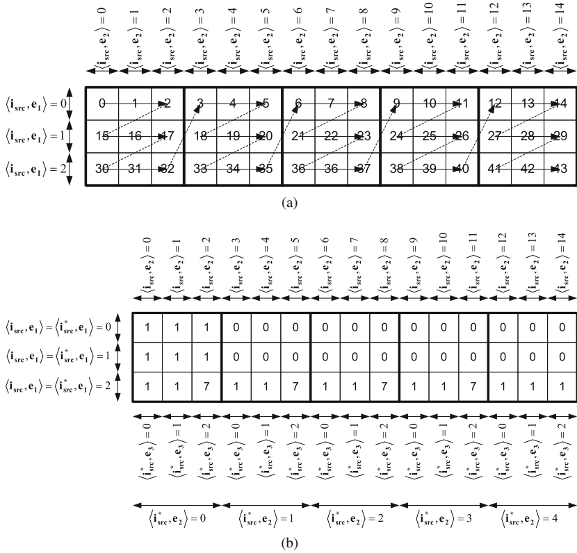
Fig. 8.13 Occurrence of modular dependencies when calculating \Delta snk(i_{src}) for image tiling. a Read and write orders. The write order is depicted by numbers , while arrows represent the read order. i_{src} correspond to the iteration vector describing which data element is currently written. b Number of enabled additional sink invocations \Delta snk(i_{src}) for each write operation. Obviously, all tiles show the same pattern, except the first and the last one. This, however, leads to modular dependencies as described by Eqs. (8.47) and (8.48). Fortunately they can be eliminated by introduction of the source iteration vector i_{src}^*
