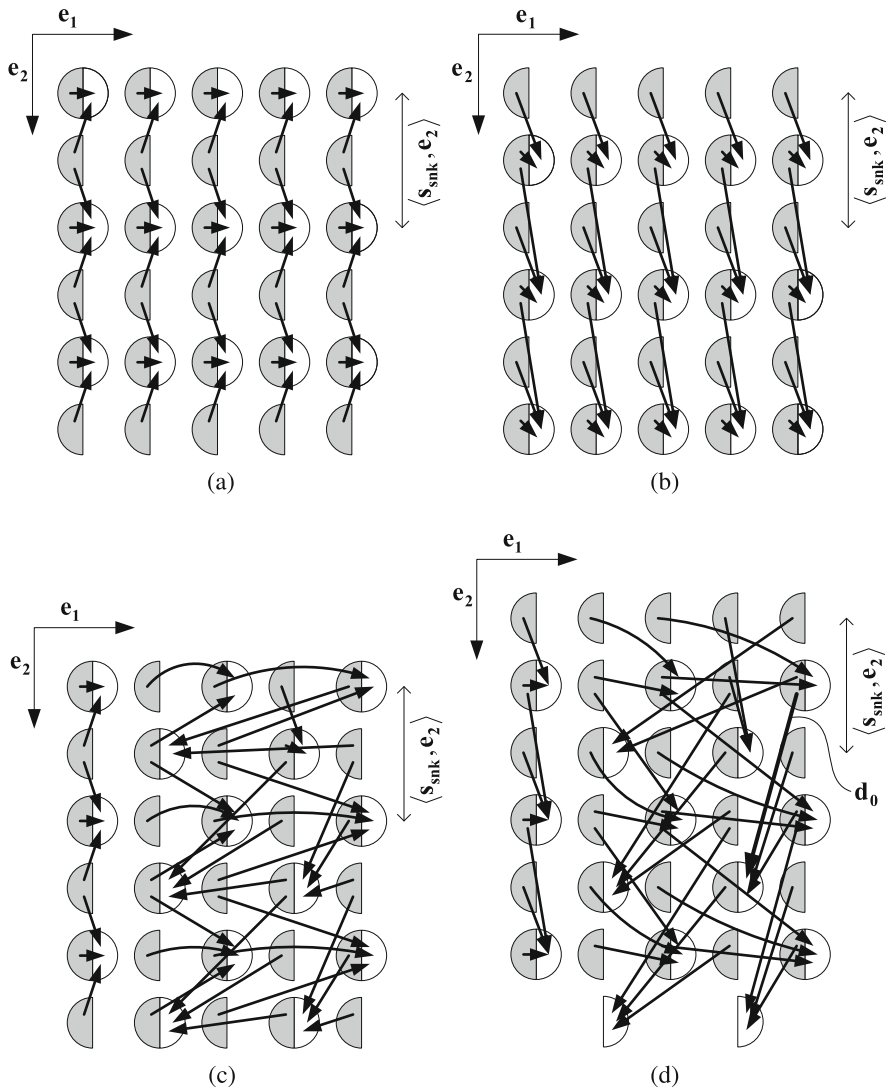
Fig. 7.22 Load-smoothing techniques for a vertical downsampler. Gray-shaded semi-circles correspond to the source, whereas the vertical downsampler is represented by white semi-circles. a Bursty schedule. b Shifted lattice for bursty schedule. c Smoothed schedule. d Shifted lattice for smoothed schedule
