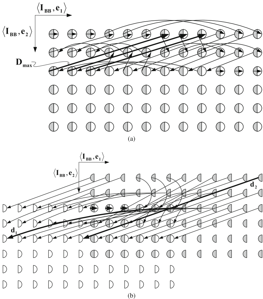
Fig. 7.12 Dependency vectors for the JPEG2000 block building. a Dependency vectors. b Shifted lattices
