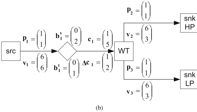
Fig. 5.22 a Lifting scheme for a one-dimensional vertical wavelet transform. Gray-shaded data elements belong to the extended border. b Corresponding WSDF graph
