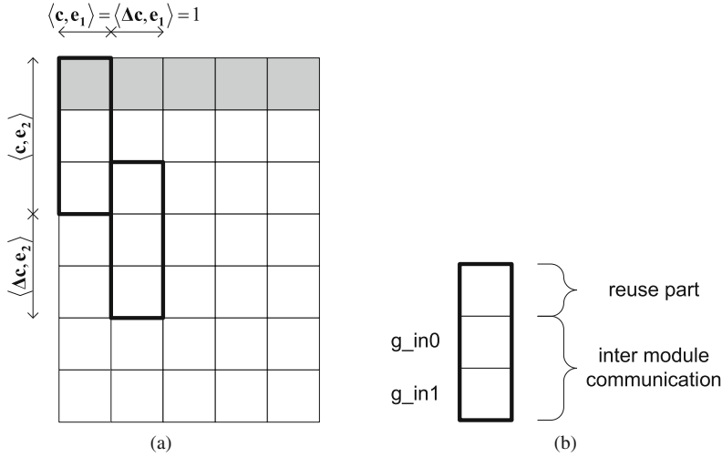
Fig. 8.18 Downampler with data reuse. a Vertical downsampling with a 1 \times 3 sliding window. b Division of the sliding window
