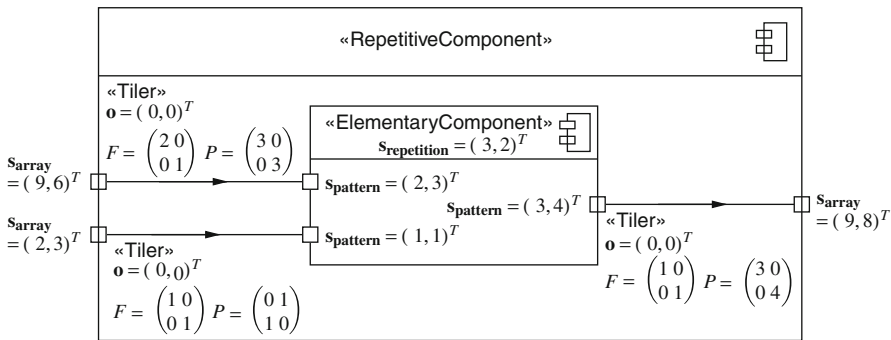
Fig. 3.6 Specification of repetitive tasks via tilers. Each port is annotated with the produced and consumed array size. The number of sub-task invocations is defined by vector \mathbf{S}_{\text{repetition}} . The tiler associated with each communication edge specifies the extraction of sub-arrays
