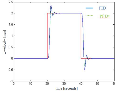
Fig. 7.14 Time response of the system under the action of the PID and PI^\lambda D^\mu controllers.
