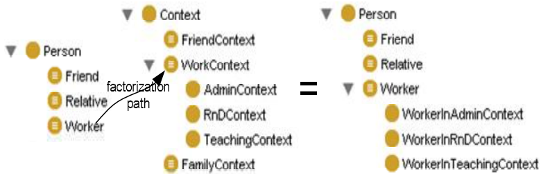
Fig. 9.8 Ontology factorization example
