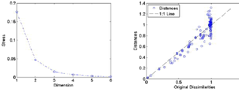
Fig. 3.10 Evaluation of MDS results: Stress test (left); Shepard plot (right)
