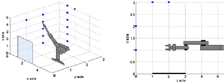
Fig. 3.3 Schematic representation 3D (left) and 2D (right) of the robot and the impact surface on the virtual cartesian coordinate system
