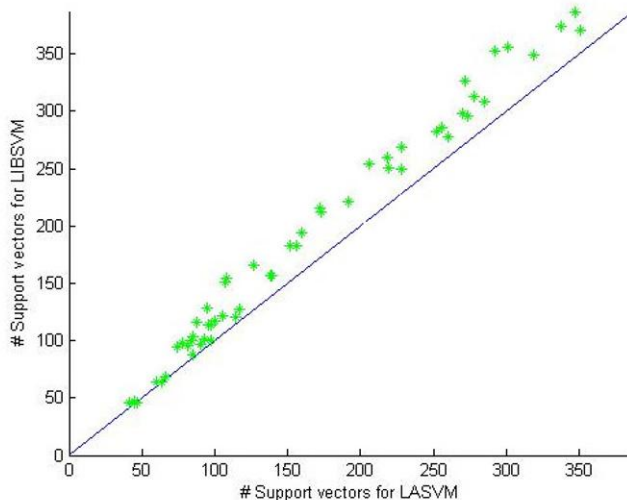
Fig. 6.5 Number of support vectors retained by the individual models trained using profile (5, 7.5). Each point is given by the values from LASVM plotted against the ones from LIBSVM, for each individual family.
