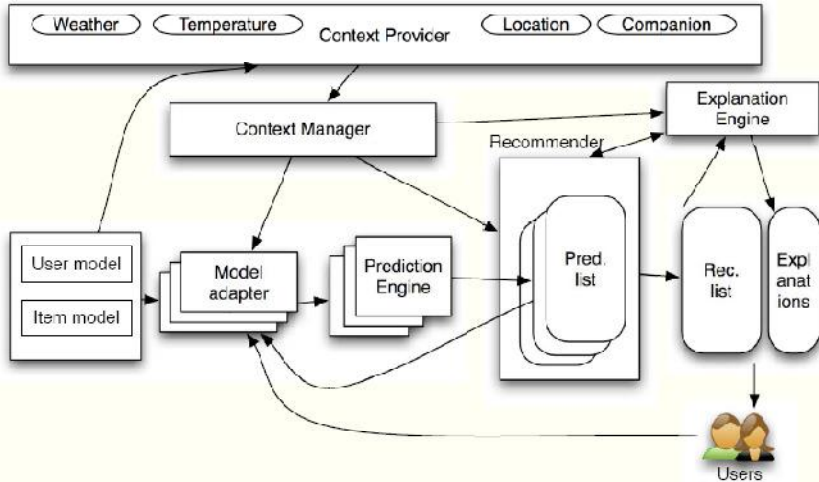
Fig. 9.2 Reference architecture for context-aware recommendation system (Baltrunas 2008)
