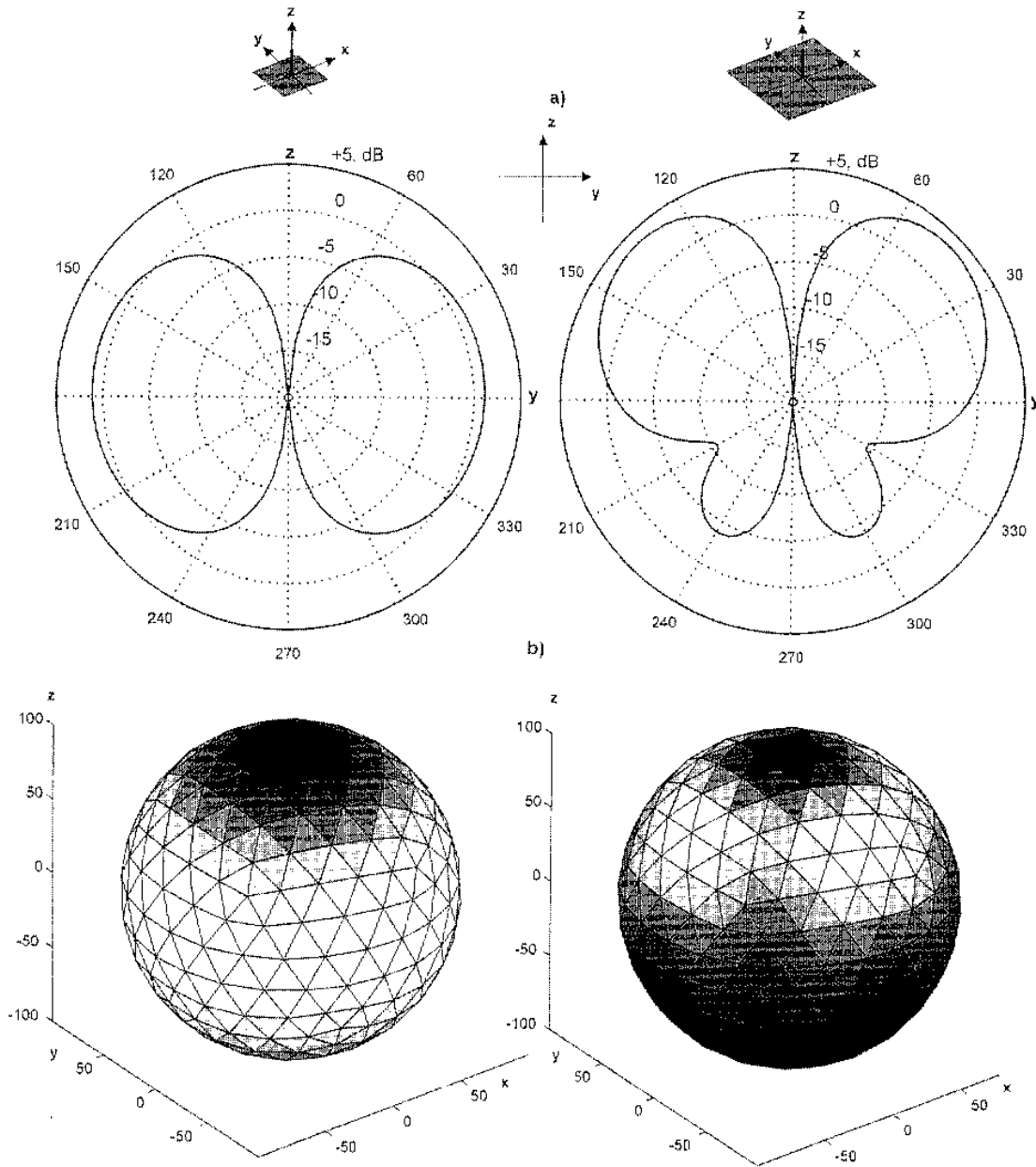
Figure 4.12. Directivity patterns and 3D radiation patterns of the radiated antenna field ( efield3.m ) of the quarter-wavelength monopole at 75MHz. Left: 2 \times 2\text{m} ground plane; right: 4 \times 4\text{m} ground plane. OFFSET = 20dB in the script efield2.m .
