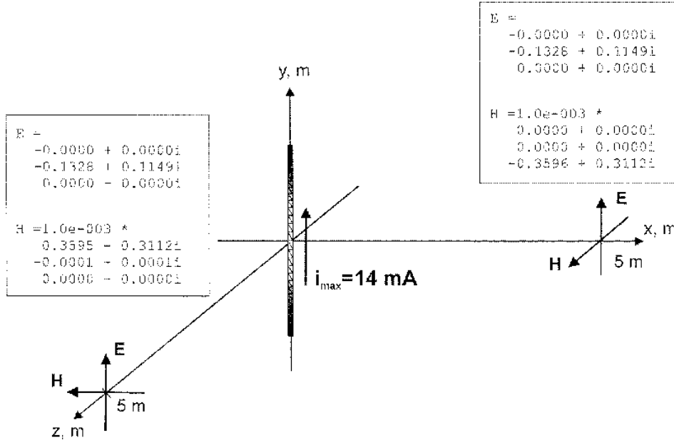
Figure 3.6. Radiated field of a dipole obtained by efield1.m .
