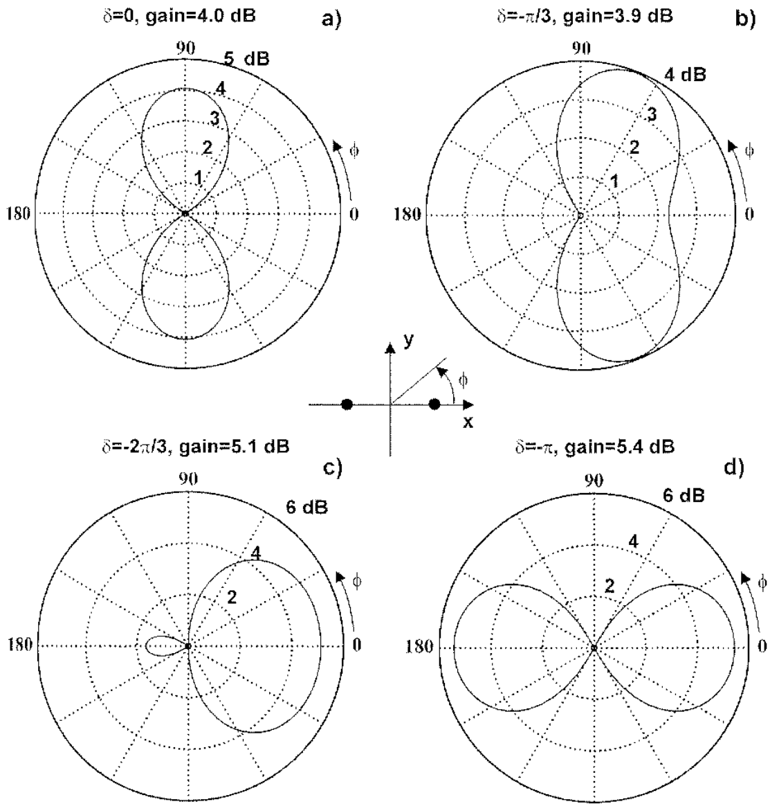
Figure 6.9. (a) Broadside; (b–d) end-fire arrays: Directivity patterns (xy-plane) of the radiated array field ( \epsilon\epsilon_0\mathbf{E}\mathbf{d}^3/\pi ). The array of the two half-wavelength dipoles is considered at \delta = 0 , \delta = -60^\circ , \delta = -120^\circ , and \delta = -180^\circ . The element spacing is d = \lambda/3 = 1.333\text{m} .
