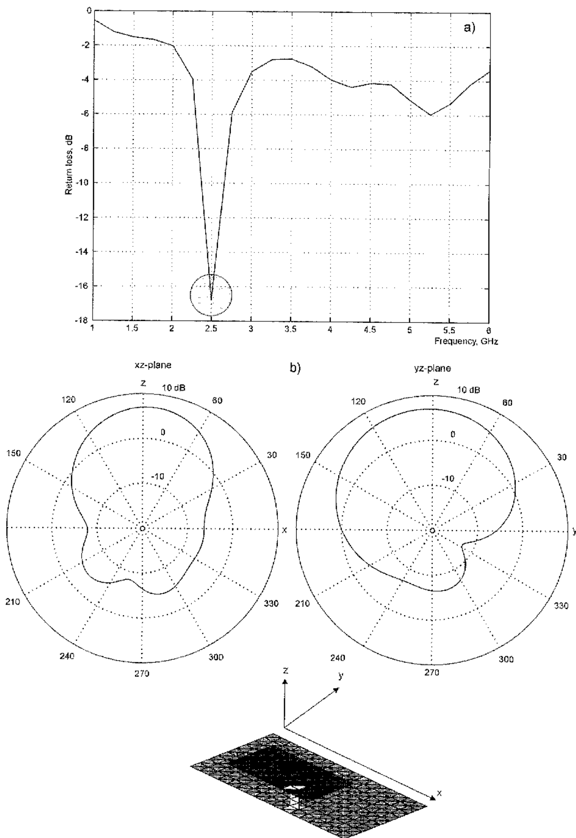
Figure 10.10. Return loss and radiation patterns of the "wide" patch antenna at 2.5 GHz.
