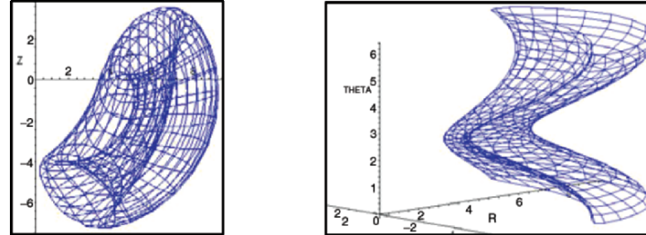
Figure 3. A numerical example for Case A without void, a_1 1.24; \alpha_1 2.41; a_2 5.58, a_3 2.12; d_2 2.22; \alpha_2 0.588, d_3 0.307: a) workspace cross section; b) surface S (u is unit length and angles are in radians).
