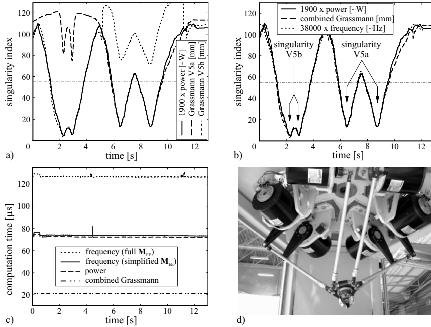
Figure 3. a) and b) Comparison of the singularity closeness indexes; c) Computational time; d) Hexa robot of Collaborative Research Center 562.
