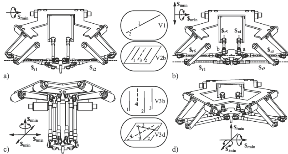
Figure 2. Grassmann variety on the Hexa robot: a) V1; b) V2b; c) V3b; d) V3d.
