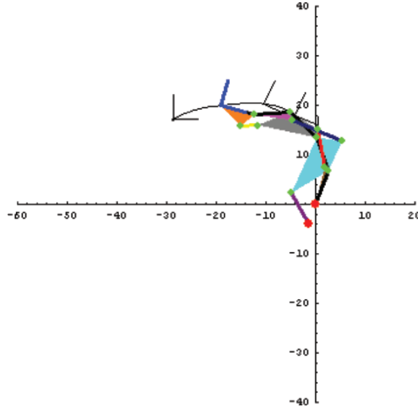
Figure 4. This 10-bar chain is obtained from a 5R that reaches the same five task positions.
