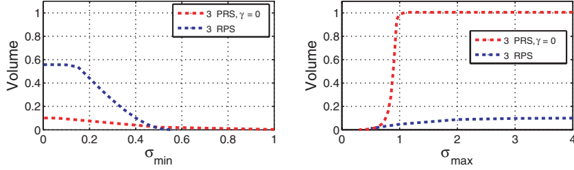
Figure 4. Workspace volume as a function of a minimum (left) and maximum (right) permissible singular values.
