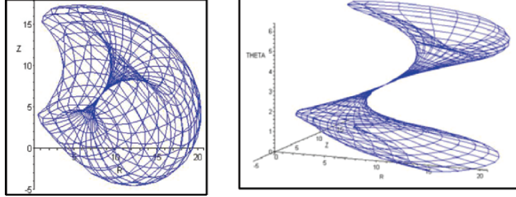
Figure 5. A numerical example for Case B without void, a_1 = 5.32 ; \alpha_1 = 0.777 ; a_2 = a_3 = 6.46 ; d_2 = 8.99 ; \alpha_2 = \pi/2 , d_3 = 0 : a) workspace cross section; b) surface S (u is unit length and angles are in radians).
