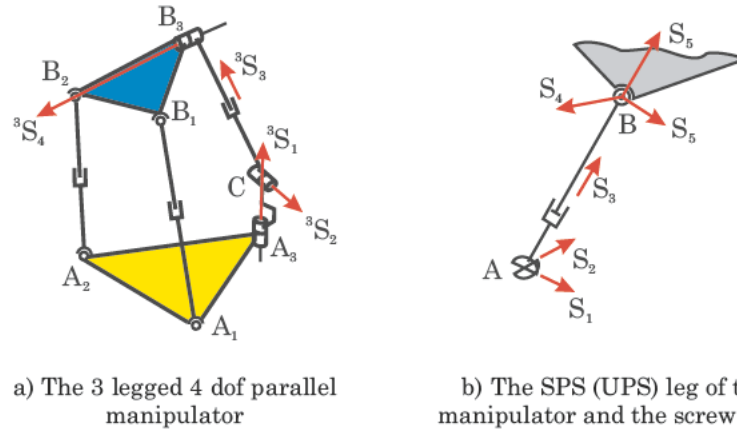
Figure 1. The 3 legged 4 dof parallel manipulator and the joint screw axes.
