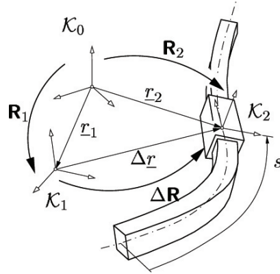
Figure 2. Model of a spline joint.
