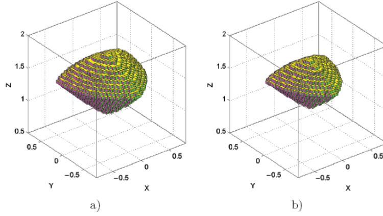
Figure 3. Workspace of the SSM a) constant orientation workspace b) total orientation workspace.
