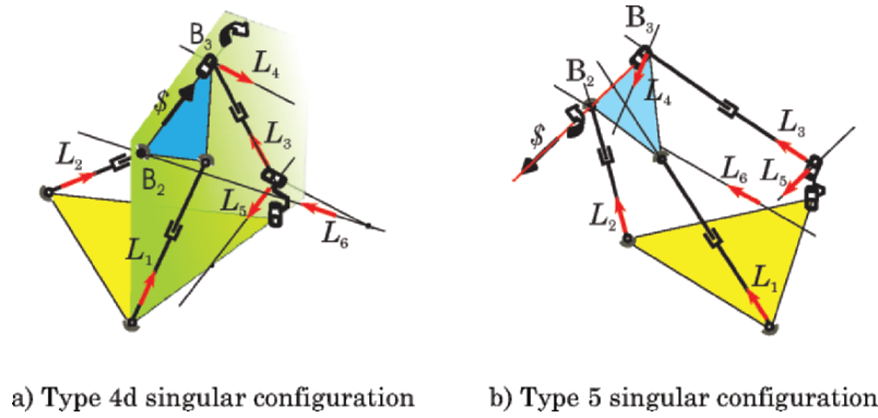
Figure 4. Types 4 and 5 singular configurations.
