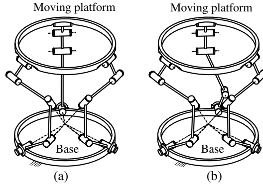
Figure 4. Two UP-equivalent parallel manipulators: (a) \ddot{R}(RRR)_E^{\parallel} -2- \ddot{R}\ddot{R}\ddot{R}(RR)_E^{\perp} , and (b) \ddot{R}\ddot{R}(RRR)_E^{\parallel} -2- \ddot{R}\ddot{R}\ddot{R}(RR)_E^{\perp} .
