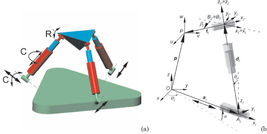
Figure 3. Sketch of the tetrahedral 3 CCR architecture and loop closure for i^{th} limb.
