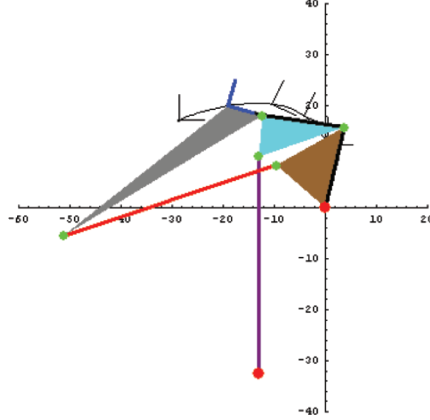
Figure 2. This six-bar chain is obtained by designing two RR chains to constrain the joint movement of a 3R robot, so its end-effector passes through the five specified positions.
