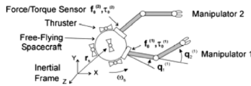
Figure 2. Space robot with sensors between spacecraft and manipulators.
