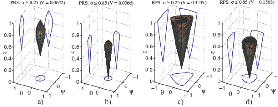
Figure 3. Regions of the workspace corresponding to high end effector velocities and fine resolution over the manipulator pose for the 3- PRS (a and b, respectively) and the 3- RPS (c and d, respectively). Angles \theta and \psi are in radians.
