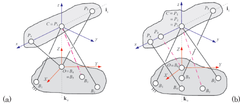
Figure 5. Over-constrained mechanisms.
