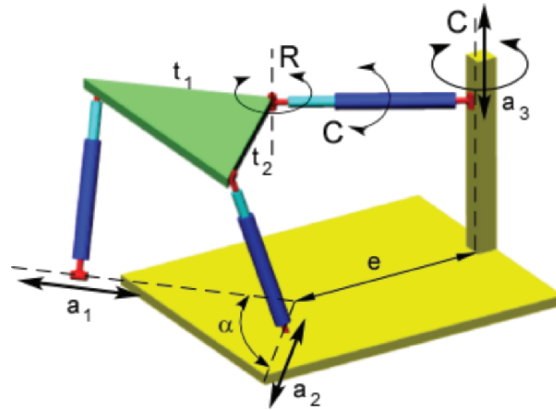
Figure 4. Sketch of the Cartesian 3 CCR architecture.
