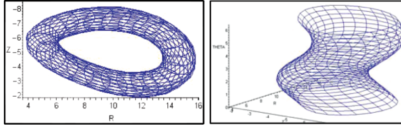
Figure 2. A numerical example for Case A with void, a_1 4.68; \alpha_1 2.90; a_2 9.78, a_3 1.15; d_2 4.48; \alpha_2 0.938, d_3 1.38: a) workspace cross section; b) surface S. (u is unit length and angles are in radians).
