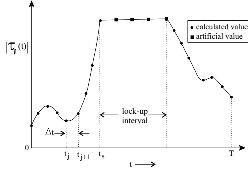
Figure 3. Numerically computed absolute torque values, |\tau_i(t)| , along lock-up trajectory.
