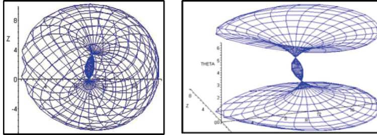
Figure 7. A numerical example for Case C without void, a_1 = 9.87 ; \alpha_1 = 0.852 ; a_2 = 4.36 , a_3 = 4.99 ; d_2 = 1.84 ; \alpha_2 = \pi/2 , d_3 = 0 : a) workspace cross section; b) surface S. (u is unit length and angles are in radians).
