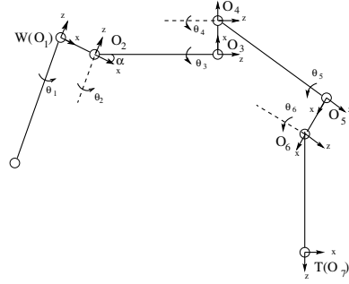
Figure 2. Equivalent model.
