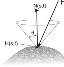
Figure 3. The friction cone.
