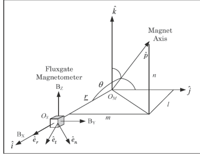
Figure 2. Sensor Diagram.
