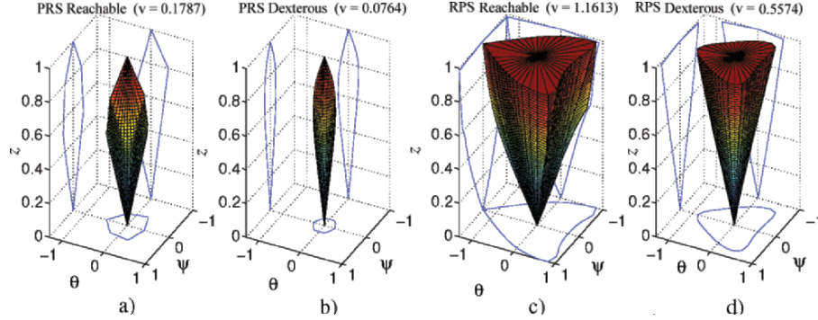
Figure 2. Reachable and Dexterous workspace for the 3- PRS (a and b) and the 3- RPS (c and d). Note \theta and \psi are in radians, r_p = 0.6 , for the 3- PRS : \gamma = 0^\circ and |\mathbf{l}_i| = 1 and for the 3- RPS : |\mathbf{b}_i| = 1 . Dexterous workspace boundary at \text{cond}_{\max} = 6 .
