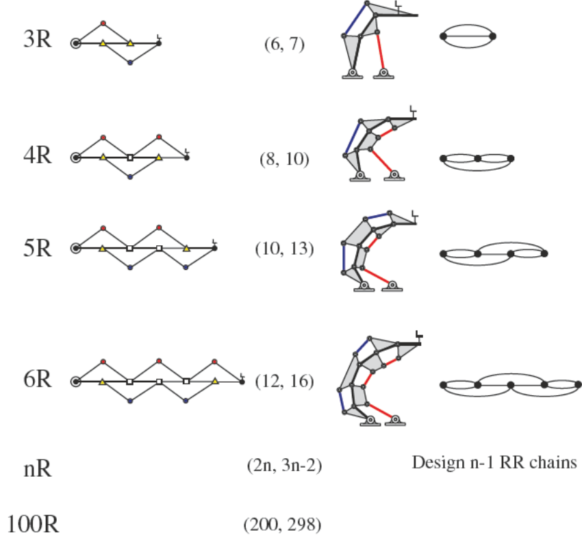
Figure 1. This shows the kinematic structure of mechanically constrained serial chains. The linkage graph is on the left, which has each link as a node and each R joint as an edge. The contracted graph on the right shows only links with three or four edges as nodes. This shows that the structure extends to any length of nR robot.
