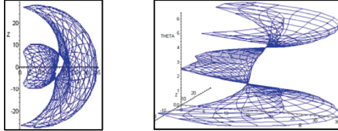
Figure 6. A numerical example for Case C with void, a_1 = 6.23 ; \alpha_1 = 1.23 ; a_2 = 9.47 , a_3 = 19.13 ; d_2 = 0.973 ; \alpha_2 = \pi/2 , d_3 = 0 : a) workspace cross section; b) surface S. (u is unit length and angles are in radians).
