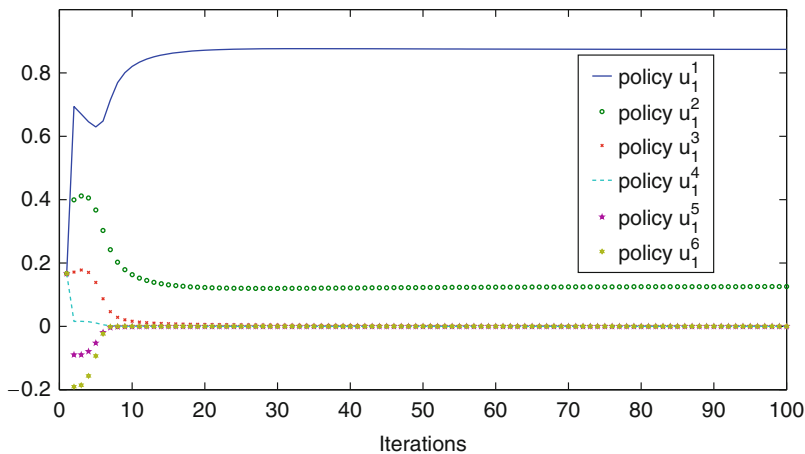
Fig. 3 Replicator dynamic with p = 0.1
