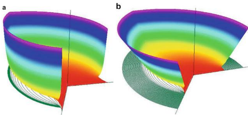
Fig. 20 Value function in the surveillance-evasion game. (a) \nu = 0.588 , \alpha = 130^\circ . (b) \nu = 0.588 , \alpha = 121^\circ
