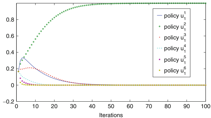
Fig. 2 Replicator dynamic with p = 0.5
