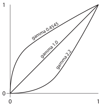
Figure 11.9 Graph of monitor gamma (2.2) with file gamma (0.4545) and linear (1.0). These are the color curves in question, with 0.4545 and 2.2 each acting as the direct inverse of the other.
