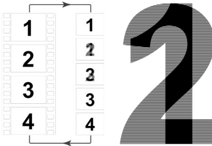
Figure 1.16 Pulldown allows 24-fps footage, the film frame rate, and enables it to play smoothly at 30 fps; without interleaving it into fields in this manner, the motion stutters, as it does if you try to go straight from 30 fps (no pulldown) to 24.
