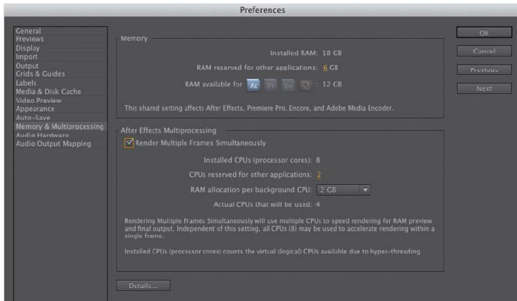
Figure 1.22 This dynamic Preferences panel contains useful information about how After Effects can use the resources on your specific system. Refreshingly, there's little here you need to adjust, other than enabling Render Multiple Frames Simultaneously and then optionally adjusting the amount of memory and number of processors reserved for other applications.
