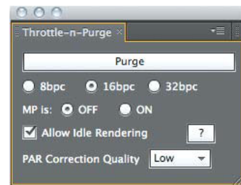
Figure 4.20 Throttle-n-Purge exposes controls to help you manage memory usage as well as offering a one-button option to purge all caches (undos and image buffers) and start over.
