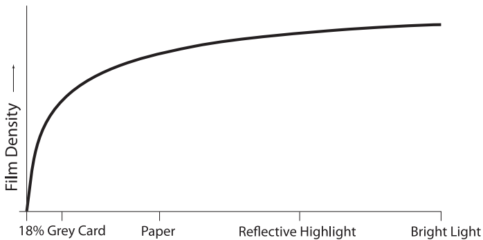
Figure 11.7 Graph the darkening (density) of film as increasing amounts of light expose it and you get a logarithmic curve.
