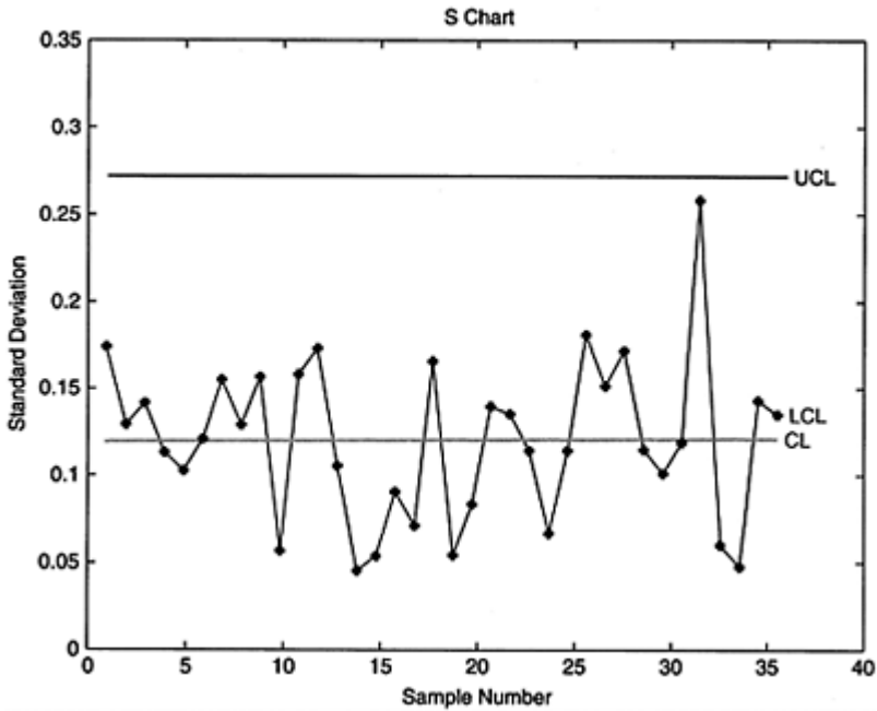
FIGURE 14-2 S chart.
