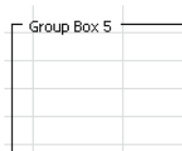
FIGURE 27-5 Group box.
