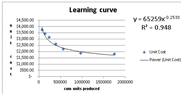
FIGURE 51-5 Learning curve for producing fax machines.
