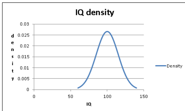
FIGURE 65-1 IQ pdf.
