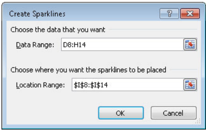
FIGURE 44-3 Creating sparklines.
