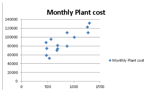
FIGURE 49-3 Scatter plot of operating cost vs. units produced.
