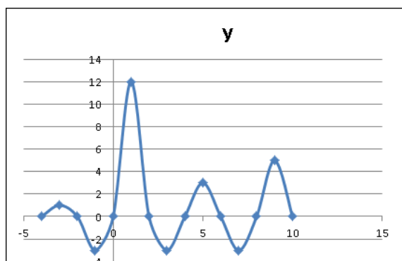
FIGURE 35-3 Maximizing a function with multiple peaks.
