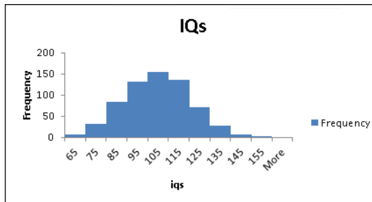
FIGURE 41-6 Symmetric histogram.
