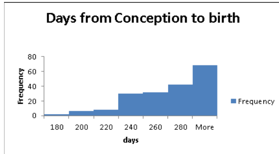
FIGURE 41-8 A negatively skewed histogram of data plotting days from conception to birth.
