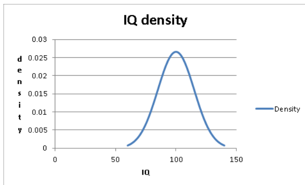
FIGURE 62-2 Probability density function for IQs.
