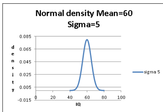
FIGURE 65-2 Normal random variable pdf with a mean equal to 60 and a standard deviation equal to 5.
