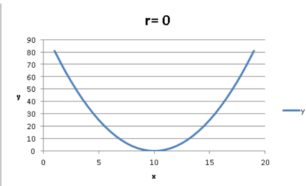
FIGURE 52-3 A correlation of 0, indicating a weak linear relationship between two variables.
