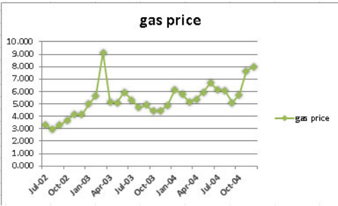
FIGURE 26-9 Gas price line graph: 2002–2004 data.
