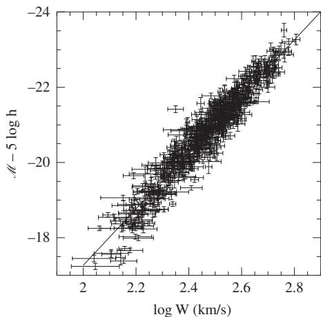
Fig. 2.22. The Tully–Fisher relation in the I -band. Here W is the linewidth of the HI 21-cm line which is roughly equal to twice the maximum rotation velocity, V_{\text{max}} . [Adapted from Giovanelli et al. (1997) by permission of AAS]
