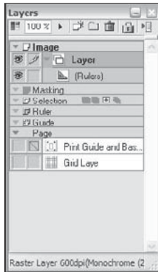
Figure 8-4: Selecting Convert to Layer on the Layer Properties palette creates a localized ruler layer.
