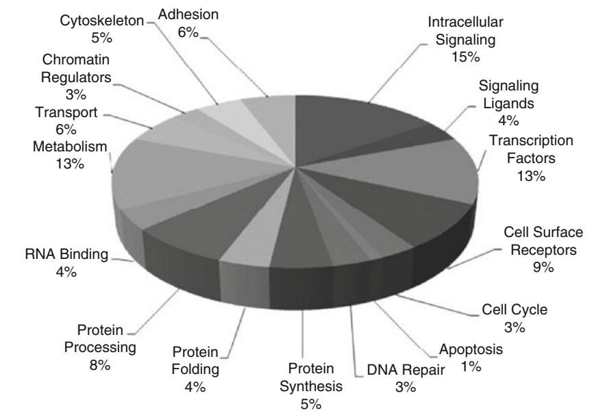
Fig. 9 A pie chart depicting the simulated average results of distribution within the HSC profile for gene products with known or putative functions
