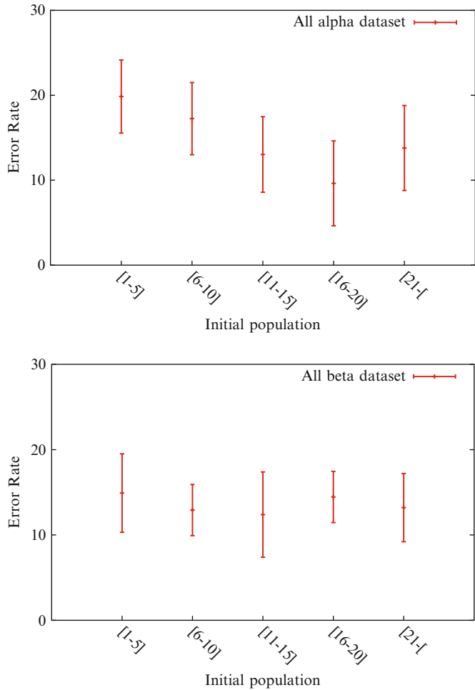
Fig. 4 Error rate as a function of the initial population size. When the initial population size is more than 10, the error rate becomes less than 15%
