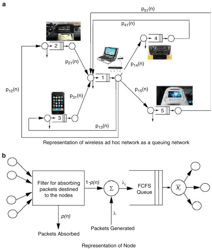
Fig. 4 Network model for ad hoc multimedia network
