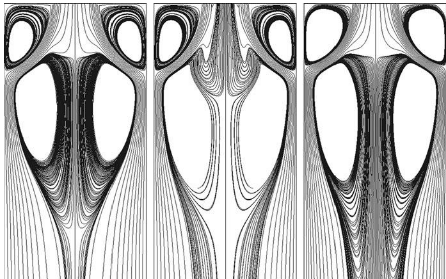
Fig. 4 Comparison of the mean streamlines with 3 k - \varepsilon models: standard ( left ), RNG ( middle ), and realizable ( right )
