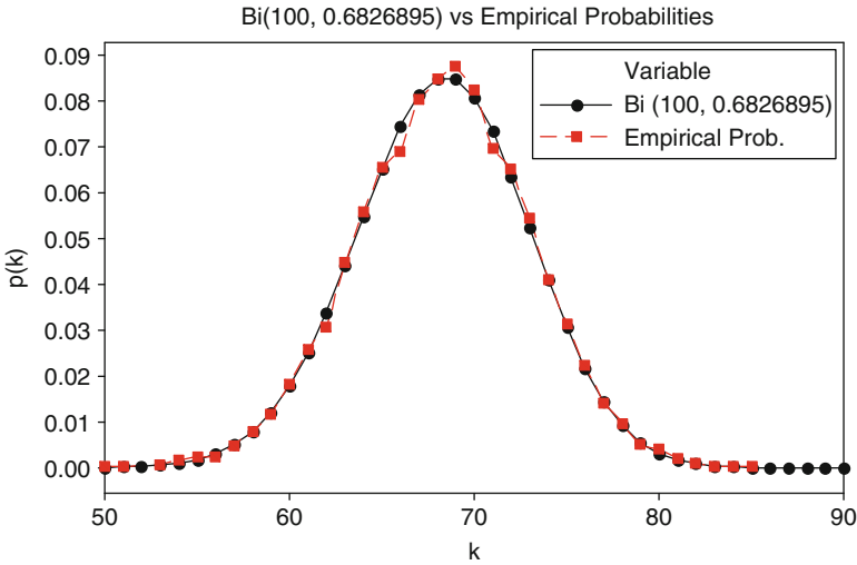
Fig. 7 Comparing empirical and calculate probability density functions of occurrences within the epsilon tube for \varepsilon = 1
