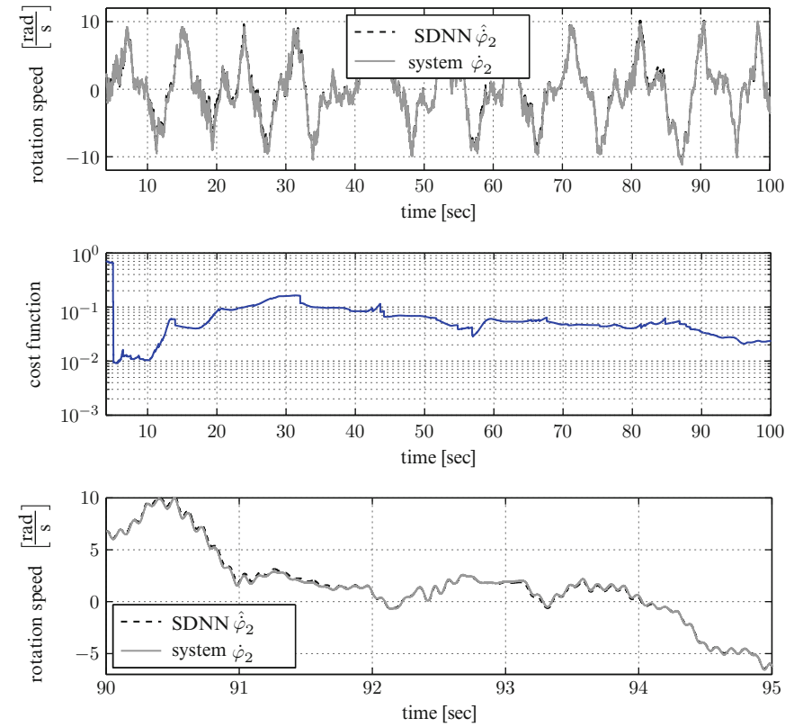
Fig. 8 Output signals of the SDNN model \hat{\dot{\varphi}}_2 and the real TMS \dot{\varphi}_2 with resulting cost function
