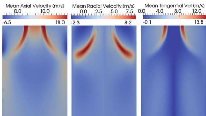
Fig. 3 Mean gas-phase velocities near the inlet with the standard k-\varepsilon model
