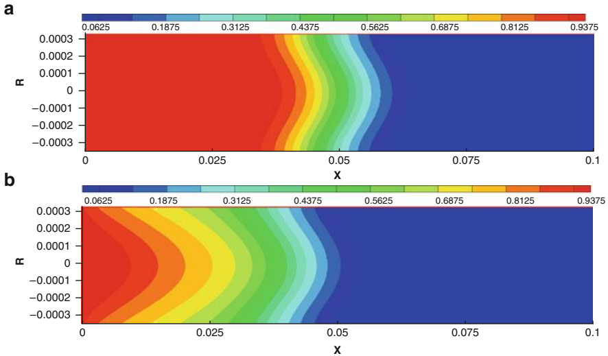
Fig. 4 A snapshot of ligand concentration distribution at t = 10 min in the capillary at the temperature of 37^{\circ}\text{C} and the uniform inlet velocity of u = 5.2\text{ mm/min} . (a) Surface binding is not considered. (b) Ligands bind to receptors and HSPGs on the capillary surface
