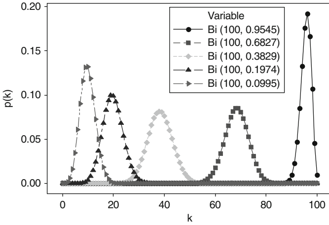
Fig. 6 STE probability density functions for \varepsilon -tubes with \varepsilon = \{2, 1, 0.5, 0.25, 0.125\}
