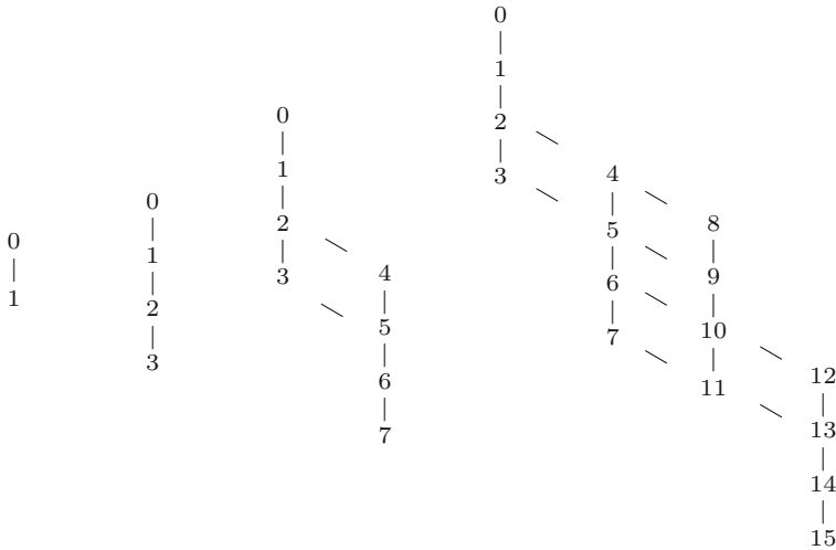
Fig. 1 The intrinsic order graph for n=1,2,3,4
