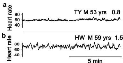
Fig. 9 Time series data of two persons. (a) Normal size healthy mail, age 53. This heartbeat looks normal. This person's EKG during this health check (Fig. 8) showed no problem with his heart, but his scaling exponent was 0.8, slightly below than normal (1.0). The detailed examination of his pulse record finally revealed that he had abnormal heartbeats. (b) A tall, close to 2 m high, healthy mail, age 59. This time the series again looked kind of normal. But this person had a scaling exponent of 1.5 (Fig. 6). Both (a) and (b) were recorded simultaneously at rest. Note that heart rate of (b) is greater than that of (a) in average, though (b) is greatly taller than (a). Generally, big body mass lowers heart rate but here not the case
