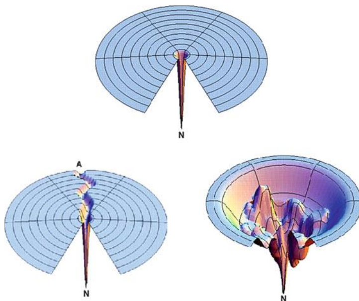
Fig. 1 Evolution in the description of folding paths in an energy landscape. Top, the protein folding according to the Anfinsen theory: a protein can adopt a large number of conformations. Bottom-left, a protein folds by following only one specific path in the conformational space. Bottom-right, from a denatured conformation, a protein searches its native structure whose energy level is minimum in a minimum time
