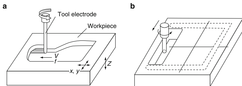
Fig. 1 Example of EDM using rotating tool electrode: (a) machining with the face of end electrode, (b) machining by the side of rotating electrode
