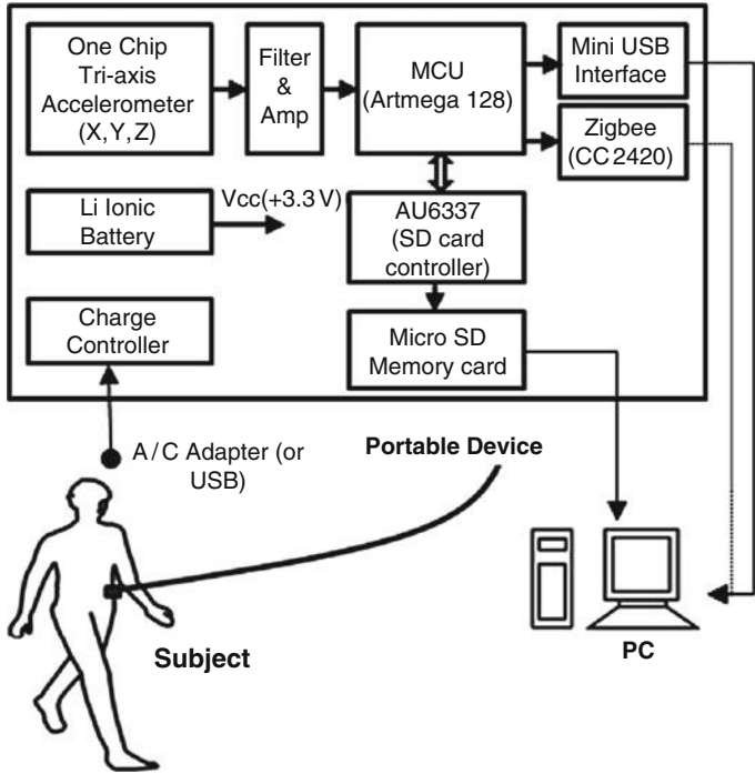
Fig. 1 Architecture of the wearable measurement device
