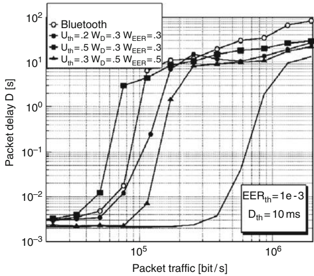
Fig. 5 Packet delay as function of buffered packet traffic
