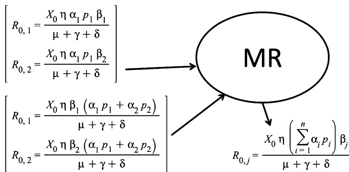
Fig. 2 Inductive mechanized reasoning for the S^nI^mR Model
