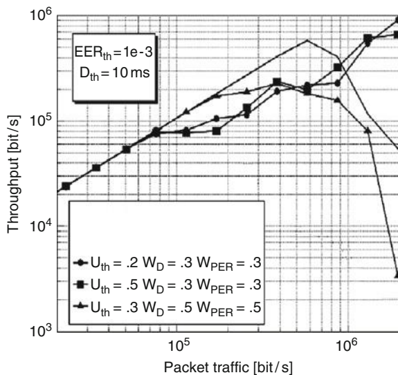
Fig. 6 Throughput as function of buffered packet traffic
