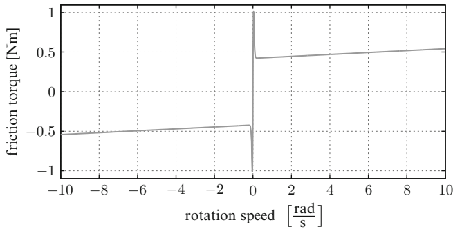
Fig. 10 Friction curve identified by the nonlinear subpart in the 11th layer
