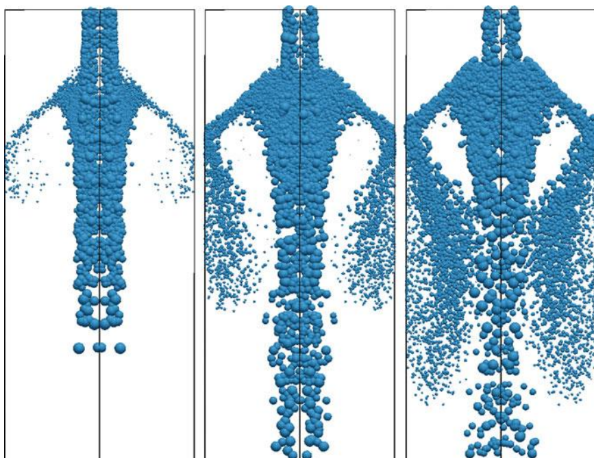
Fig. 2 Parcel motion with the standard k-\varepsilon model at t = 0.05\text{s} (left), t = 0.10\text{s} (middle), and t = 0.15\text{s} (right)
