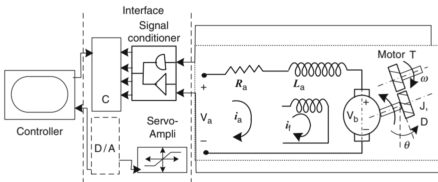
Fig. 5 Hardware setup
