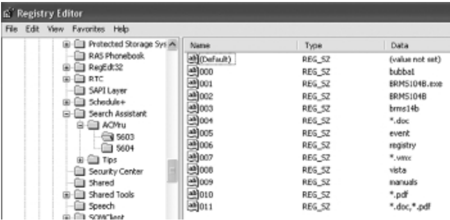
FIGURE 5.55 Examination of the currently logged on user's search activity.
