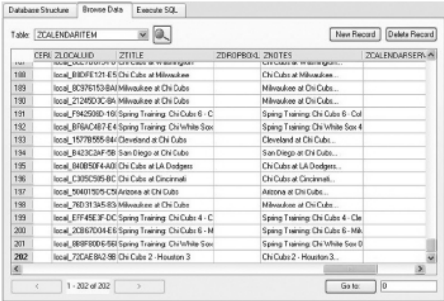
FIGURE 7.11 An example of the iCal database showing information in the calendar.
