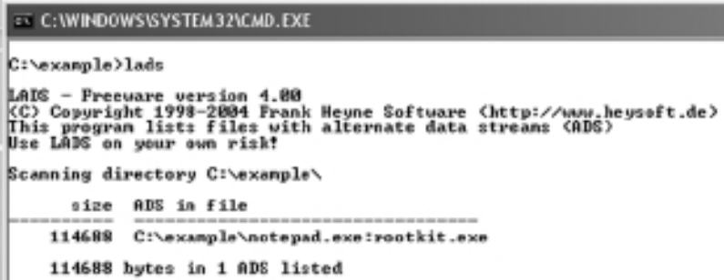
FIGURE 5.10 Example of LADS output.
