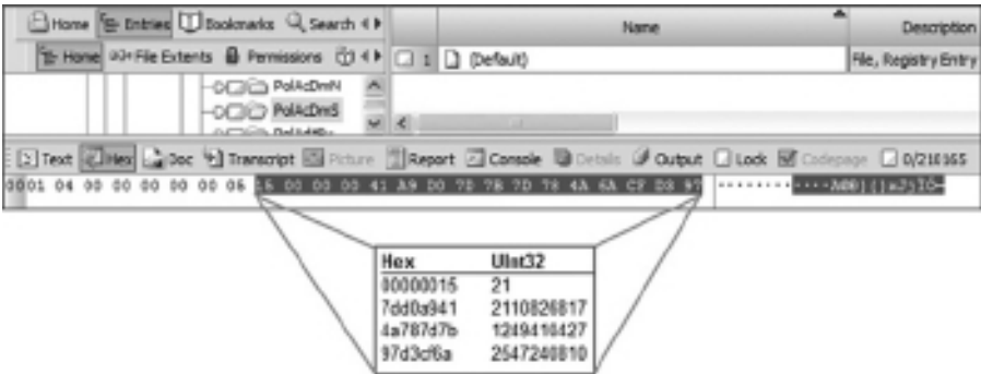
FIGURE 5.27 Translation of the last 16 bytes of the (Default) value as unsigned 32-bit integers.
