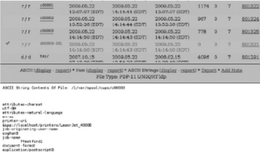
FIGURE 6.11 The contents of "/var/spools/cups" on a Linux system showing file system metadata of control files and a deleted data file.
