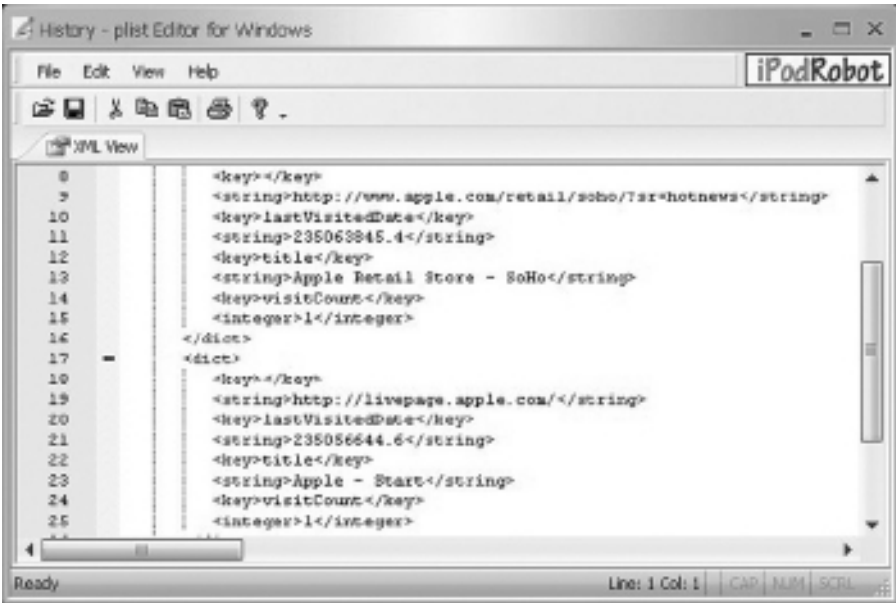
FIGURE 7.7 An exported Safari History.plist file from a Mac OS X 10.4 system.
