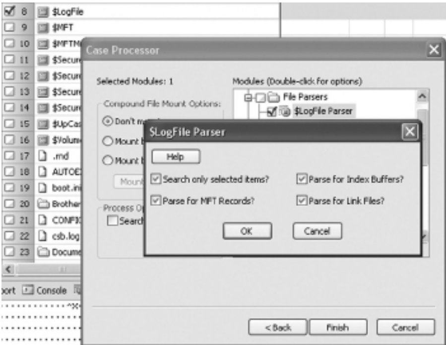
FIGURE 5.6 EnCase forensic $LogFile Parser module (under the Case Processor EnScript).
