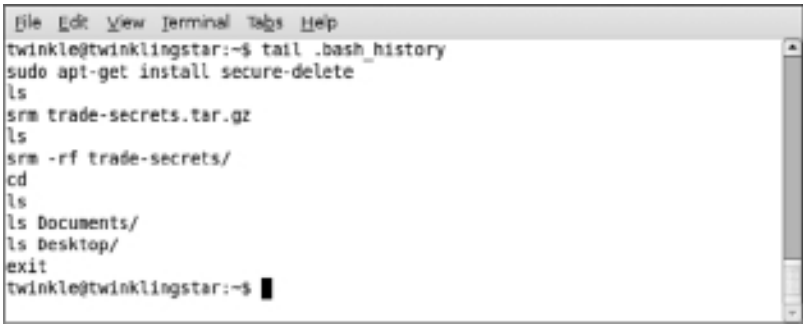
FIGURE 6.7 Command history showing data destruction activities.
