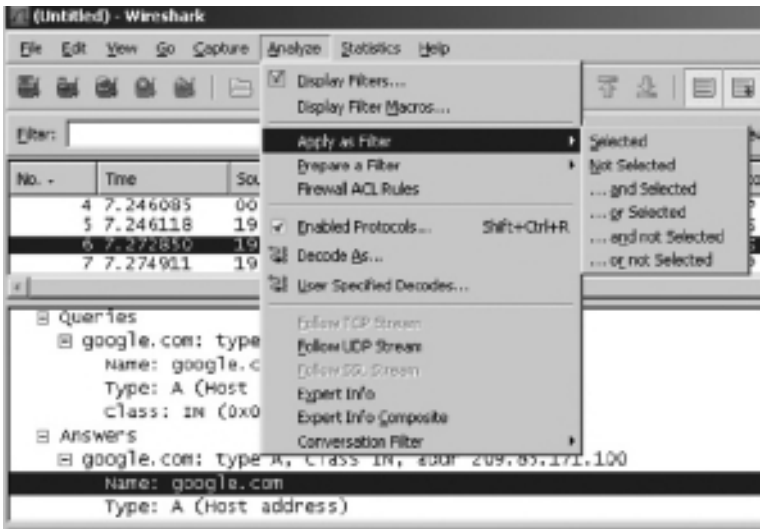
FIGURE 9.20 Using the Wireshark Apply as Filter option to select google.com from a packet and apply it to the entire network capture as a filter.
