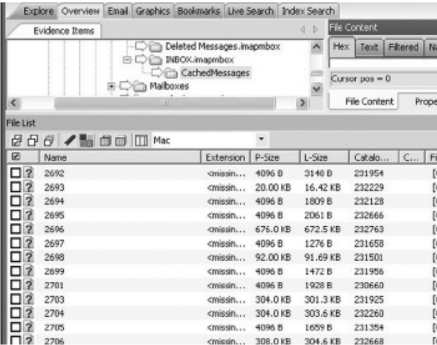
FIGURE 7.9 A representation of the CachedMessages folder for an IMAP account on a Mac OS X 10.3 system viewed using FTK.
