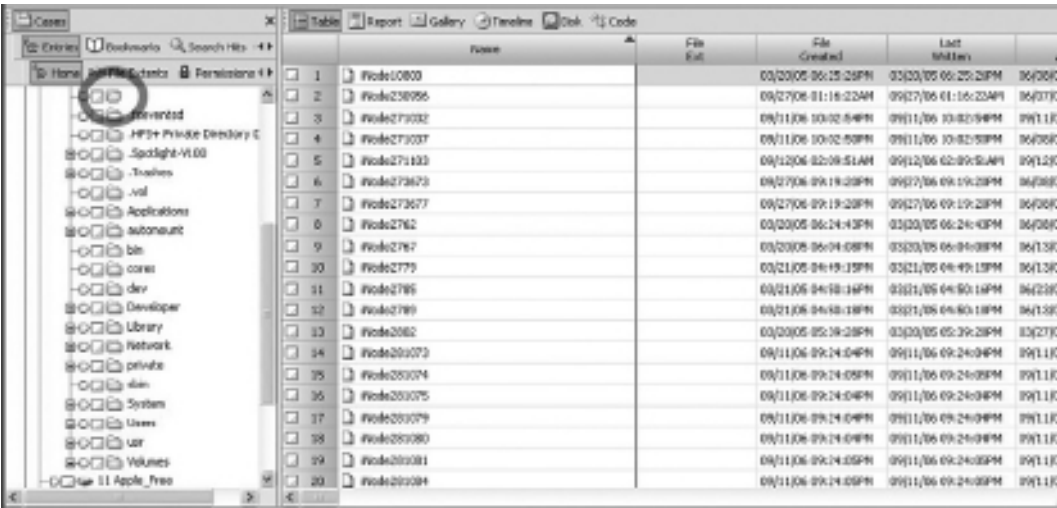
FIGURE 7.3A EnCase displays the iNode files in a nameless folder. The name of this folder has unprintable characters. Previous versions of EnCase have had different interpretations of this folder; one previous name was Cases.
