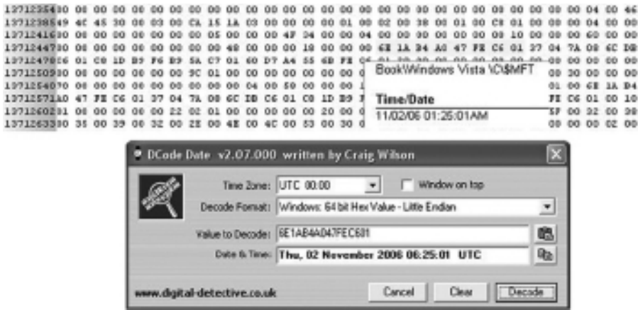
FIGURE 5.13 Interpretation of Windows 64-bit date by EnCase above, set to EST, and DCode (www.digital-detective.co.uk/freetools/decode.asp) below, set to UTC.
