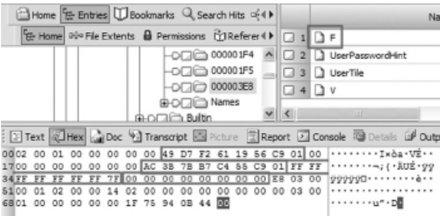
FIGURE 5.25 Date-time stamps contained within the F value for the user account.
