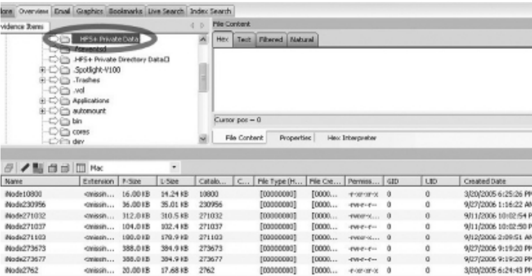
FIGURE 7.3B FTK showing the same folder. FTK displays the folder name differently, either choosing not to display the unprintable characters or to use spaces as placeholders for them.
