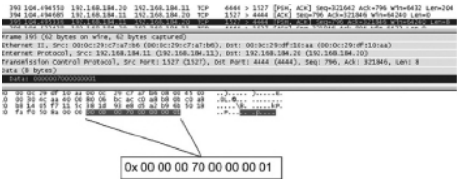
FIGURE 9.34 Part of the data transfer that is not part of the executable file.
