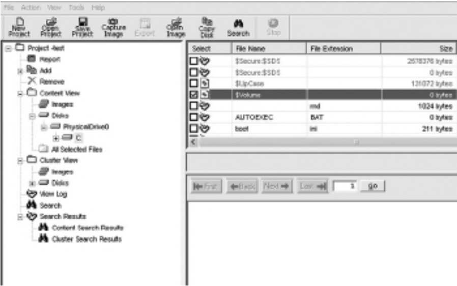
FIGURE 5.7 ProDiscover Basic showing $Volume as an empty file, with no size.
