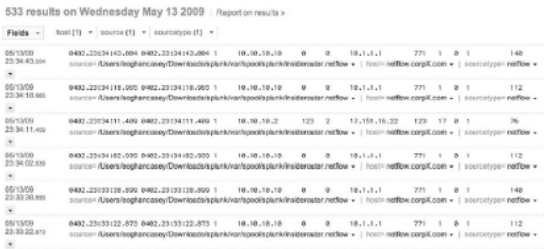
FIGURE 9.36 Splunk unable to interpret default date-time stamp format of NetFlow logs require reformatting of dates to enable correlation with other logs.
