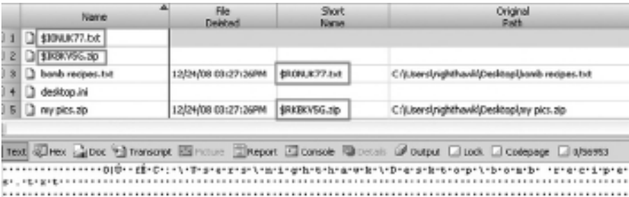
FIGURE 5.41 EnCase view of files in $Recycle.Bin on a Windows Vista system; the $I file (code shown at bottom) contains the file's deletion date-time stamp and original path (in Unicode).
