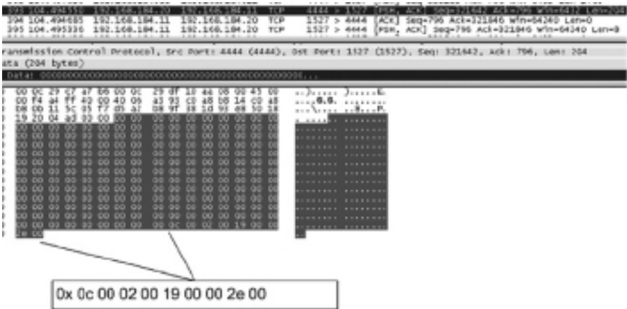
FIGURE 9.33 Possible end of file in packet payload.
