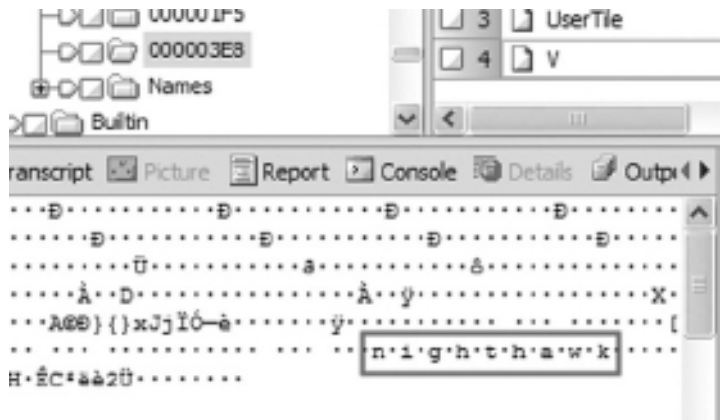
FIGURE 5.24 Content of the V value showing the username nighthawk associated with Relative Identifier 000003E8 (decimal 1000).
