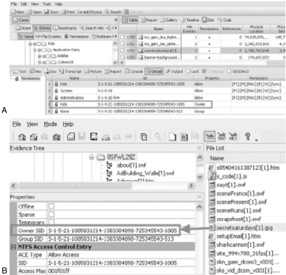
FIGURE 5.9 (a) File permissions viewed in EnCase. (b) File permissions viewed in FTK Imager.
