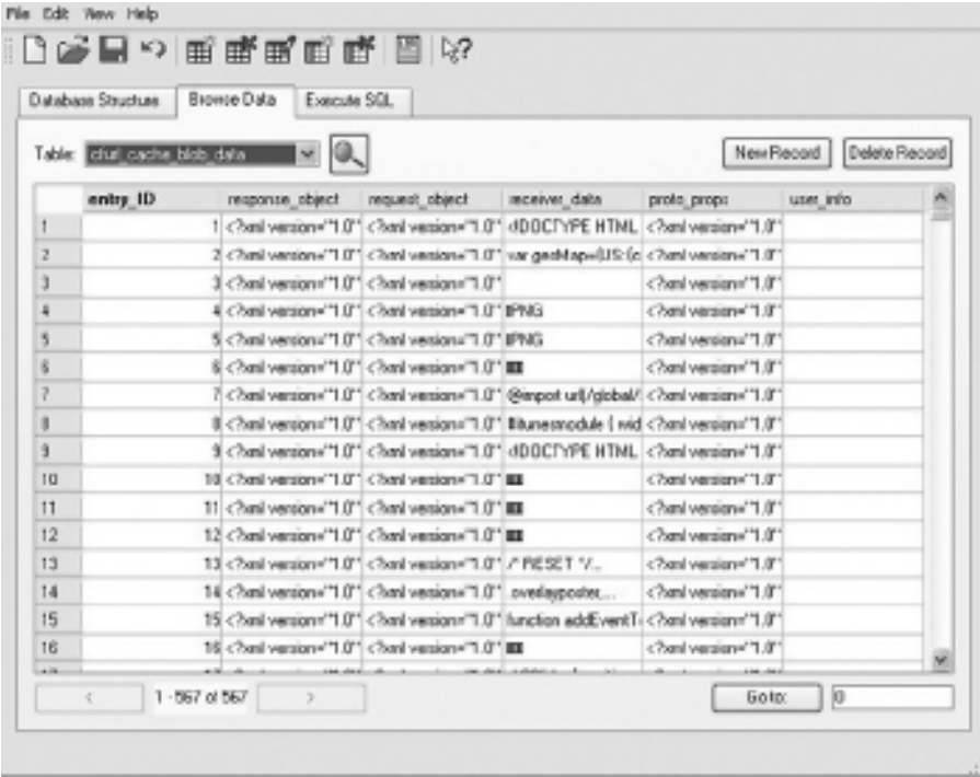
FIGURE 7.6 An example of the Safari Cache.db file in SQLite Database Browser.
