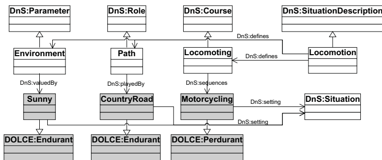
Fig. 4.3 Model for the description "Locomoting"
