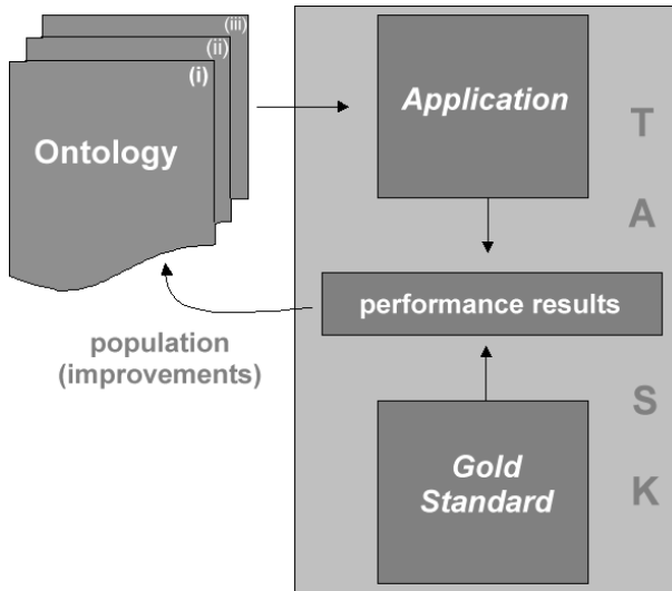
Fig. 3.5 Test Suite Setup with a single task, an application, a gold-standard and one or more ontologies
