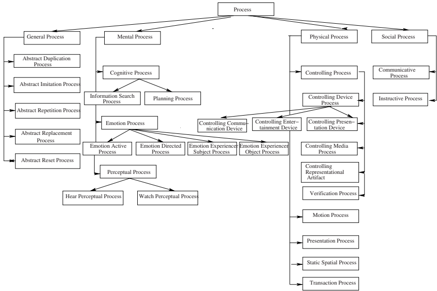
Fig. 3.3 Upper part of the process hierarchy
