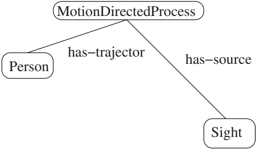
Fig. 3.6 Substitution Type A: The gold-standard relation has-target was substituted with the relation has-source
