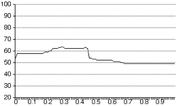
Fig. 3.4 Determining the optimal threshold on the coherent versus incoherent classification data from corpus SRH_0 . The vertical axis shows performance and the horizontal shows the word to concept threshold V
