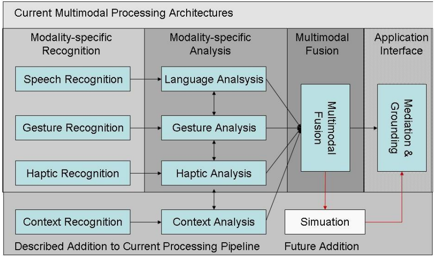
Fig. 5.2 Context-aware multimodal system with simulation
