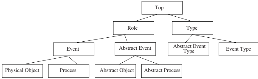
Fig. 3.2 Top-level part of the ontology
