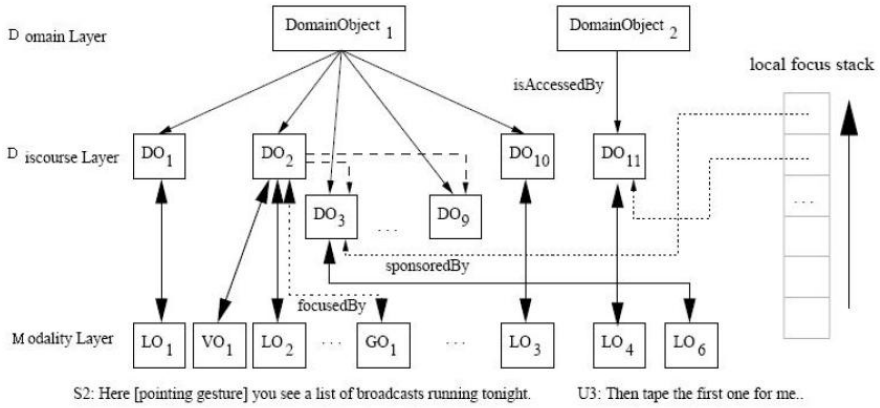
Fig. 3.1 The SmartKom Discourse Model
