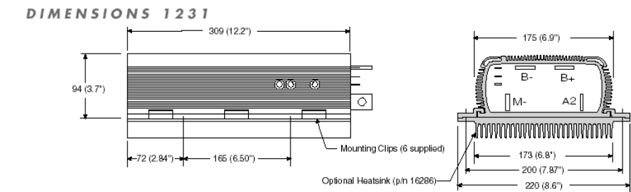
FIGURE 9-8 Dimensions for Models 1221 and 1231. ( www.curtisinst.com/index.cfm?fuseaction=cProducts.DownloadPDF&file=50003%5F1221C%2D1231C%5FRevD%2Epdf .)
