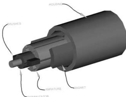
FIGURE 8-6 Three-dimensional (3D) representation of basic motor components.
