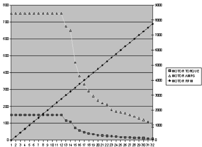
FIGURE 8-30 Advanced DC series motor curves for the L91-4003 at 120 V dc, max. 750 A.
