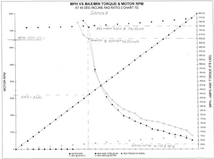
FIGURE 6-13 Wheel rpm value versus max/min torque and motor rpm on a 40-degree incline.
