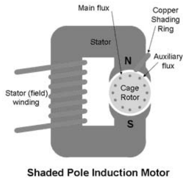
FIGURE 8-25 Basic single-phase ac motor. ( www.mpoweruk.com/motorsac.htm .)
