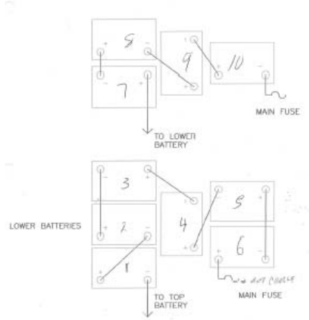
FIGURE 12-16 Battery layout for 10 batteries in series with two fuses.
