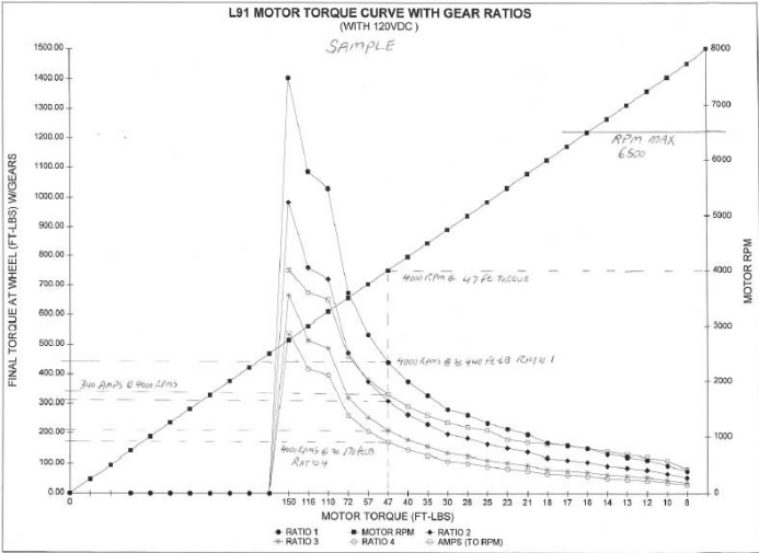
FIGURE 6-12 Advanced DC Motors curves for four-speed transmission with gear ratios.
