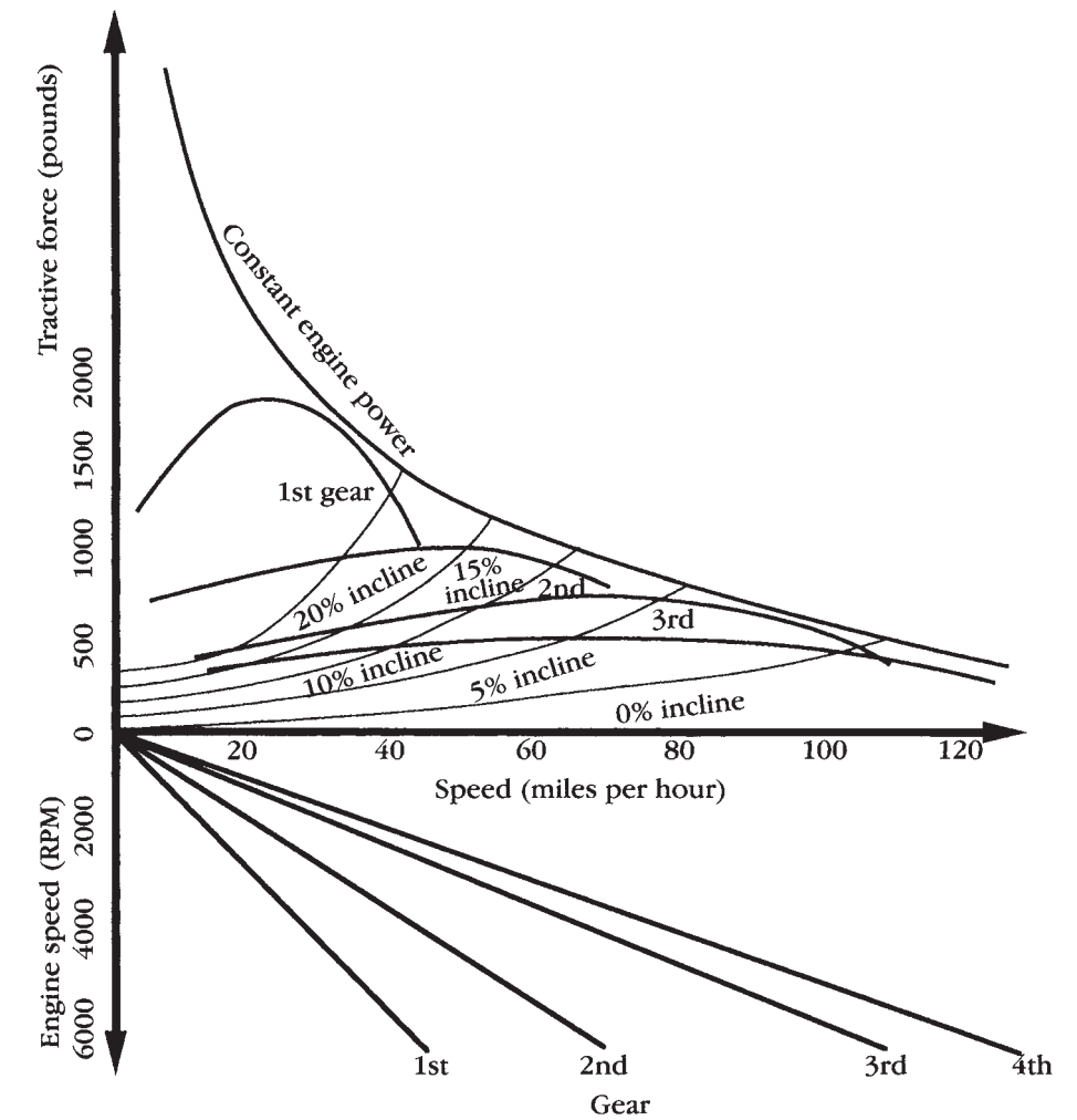
FIGURE 6-9 Transmission gear ratio versus speed and power summary. From Build Your Own Electric Vehicle , Figure 5-8, p. 117.
