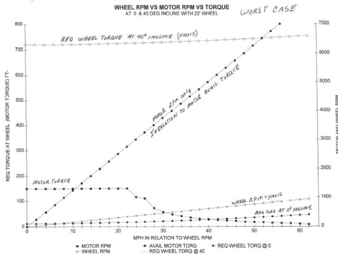
FIGURE 6-14 Wheel rpm versus motor rpm versus torque on 0- and 40-degree inclines.
