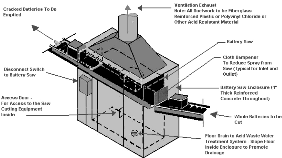
FIGURE 7-29 Battery saw used in recycling batteries. ( www.osha.gov/SLTC/etools/leadsmelter/popups/batterysaw_popup.html .)
