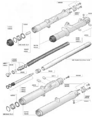
FIGURE 5-12 Typical Harley-style front fork assembly with spring. (Courtesy of Custom Chrome, www.customechrome.com .)
