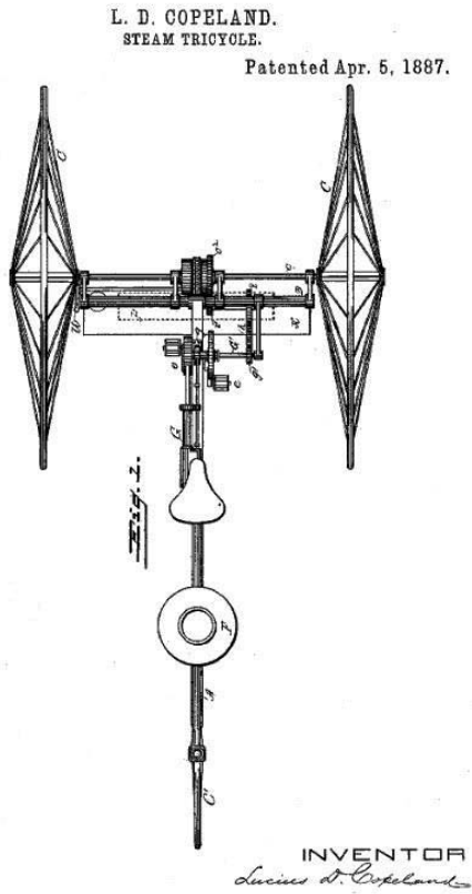
FIGURE 3-3 Inventor's drawings from Copeland's 1887 tricycle patent. ( http://patentpending.blogs.com/photos/uncategorized/early_tricycle_1.jpg .)
