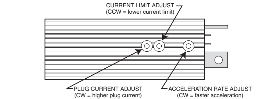
FIGURE 9-9 Basic adjustment location. ( www.curtisinst.com/index.cfm?fuseaction=cProducts.DownloadPDF&file=50003%5F1221C%2D1231C%5FRevD%2Epdf .)
