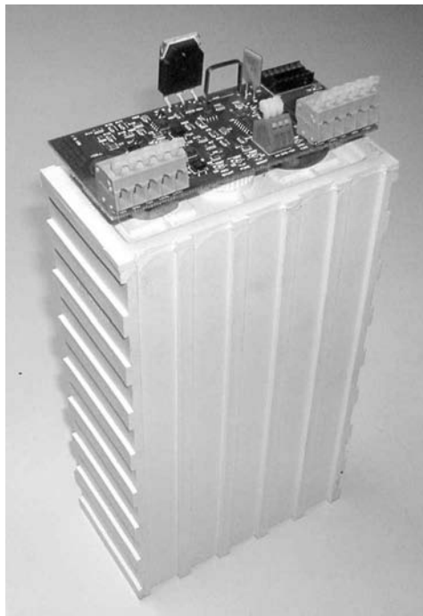
FIGURE 10-16 Battery management system. (Courtesy of Metric Mind Engineering, www.metricmind.com/bms.htm .)
