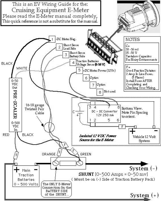
FIGURE 11-3 Link 10 wiring. ( www.xantrex.com .)
