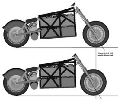
FIGURE 5-11 Effect of fork length on rake and trail: 3D image of the Electra Cruiser.
