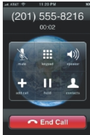
Figure 4-6: Managing calls.
