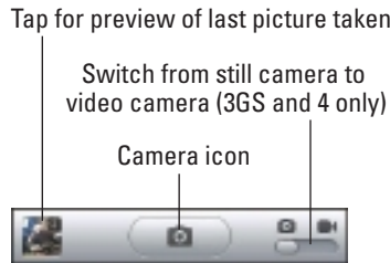
Figure 8-1: Say “Cheese.”
