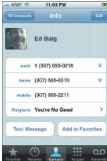
Figure 4-1: Contact me.
