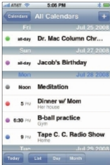
Figure 6-1: List view.
