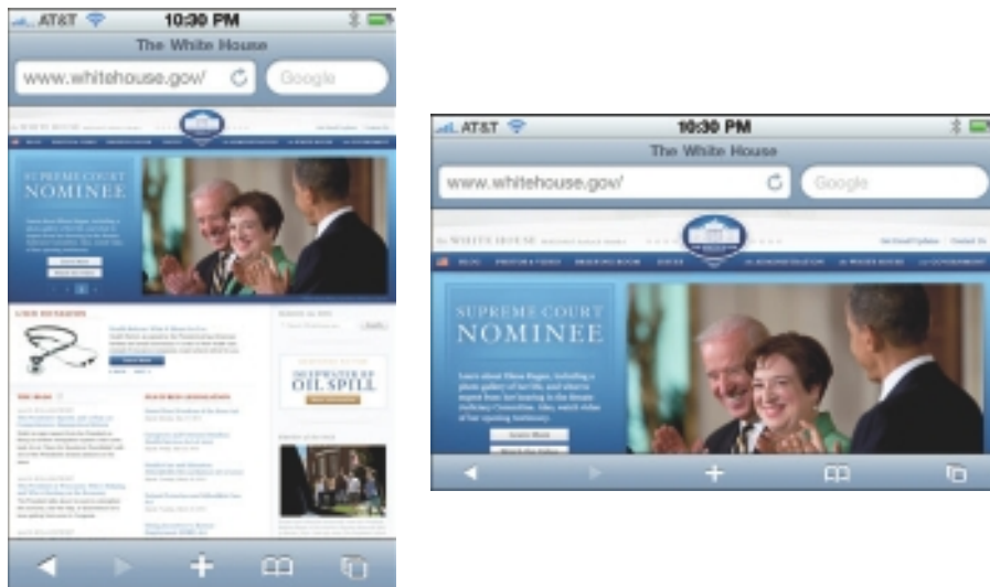
Figure 10-4: Going wide.
