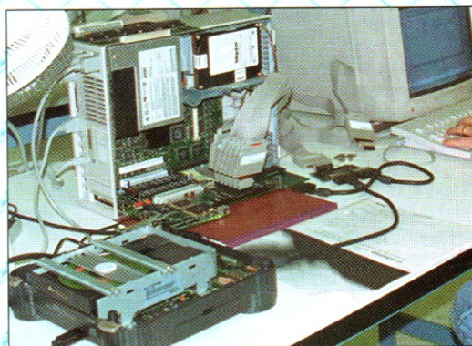
The M2 development system with its guts exposed. First games arrive in six months
