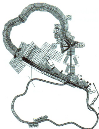
Each course is first designed on paper by Nick Burcombe (right). A 3D wireframe model is then produced in Softimage (left), prior to PlayStation conversion
