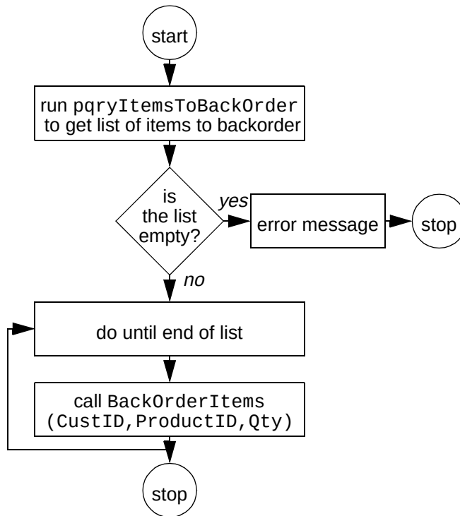
FIGURE 15.15: Flowchart for UpdateBackOrders().
