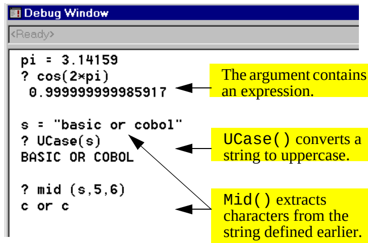
FIGURE 12.1: Interacting with the Visual Basic interpreter.
