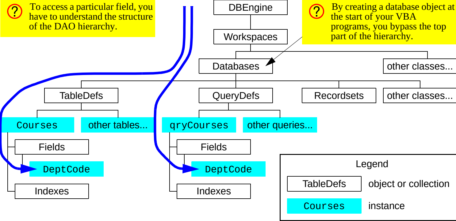
FIGURE 14.1: Navigating the DAO hierarchy.
