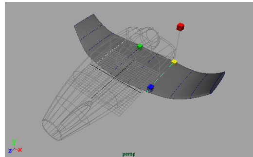
Updated loft surface
