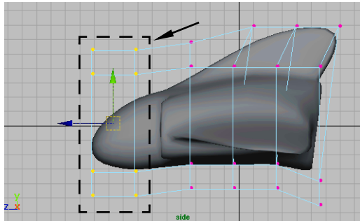
Cockpit area moved forward and down
