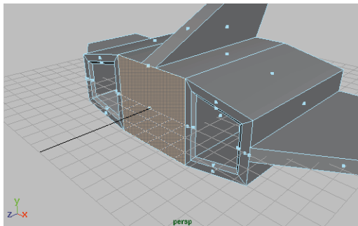
Front facet to be extruded for the cockpit
