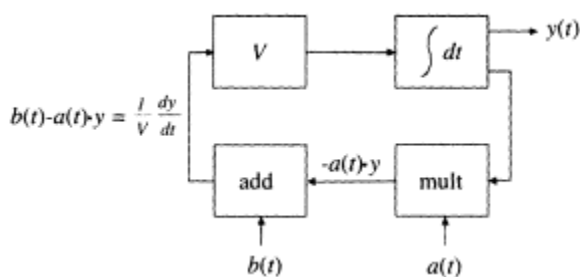
Figure 18 Division by solving a differential equation
