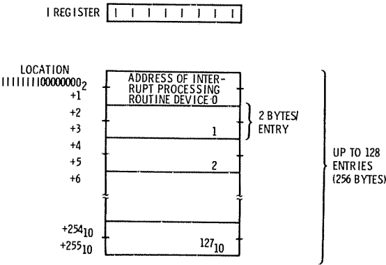
Fig. 7-5. Interrupt mode 2 interrupt vector table.
