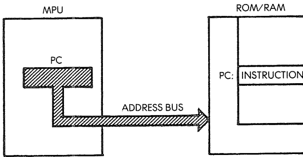
Fig. 2.6: Fetching an Instruction from the Memory
