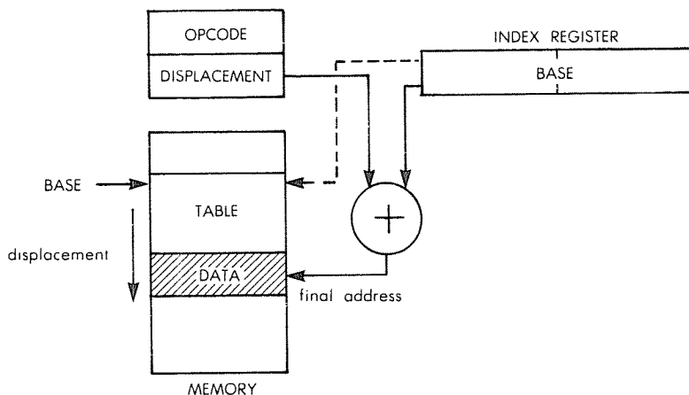
Fig. 5.2: Addressing (Pre-indexing)
