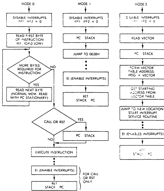
Fig. 6.26: Interrupt Modes
