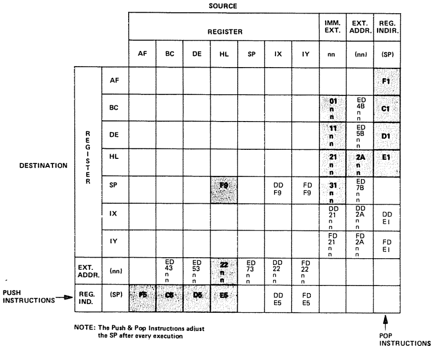
Fig. 4.3: 16-Bit Load Group—‘LD’, ‘PUSH’ and ‘POP’
