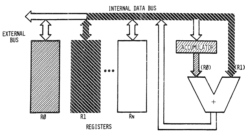
Fig. 2.10: Addition—Second Register R1 into ALU
