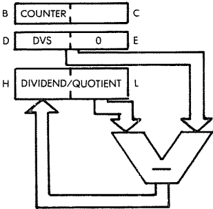
Fig. 3.31: 16 × 8 Division—The Registers
