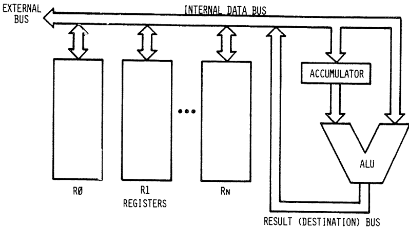
Fig. 2.8: Single-Bus Architecture
