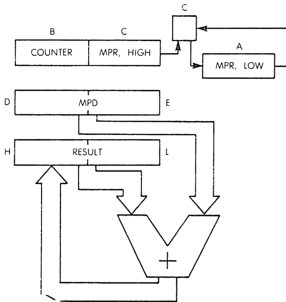
Fig. 3.27: 16 × 16 Multiply—The Registers
