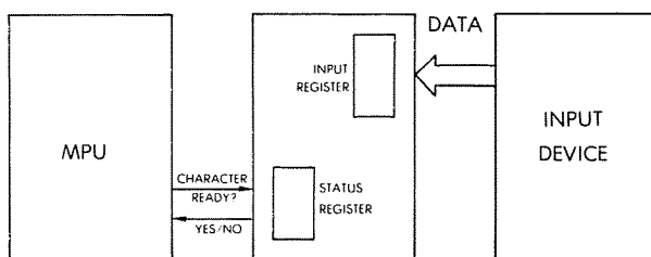
Fig. 6.8a: Handshaking (Input)
