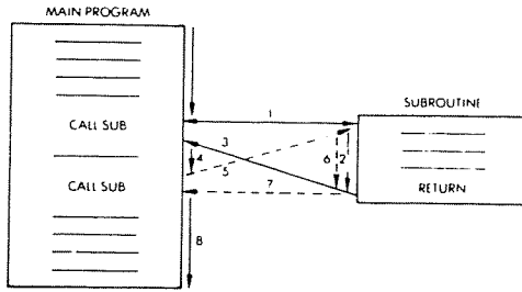
Fig. 3.35: Subroutine Calls
