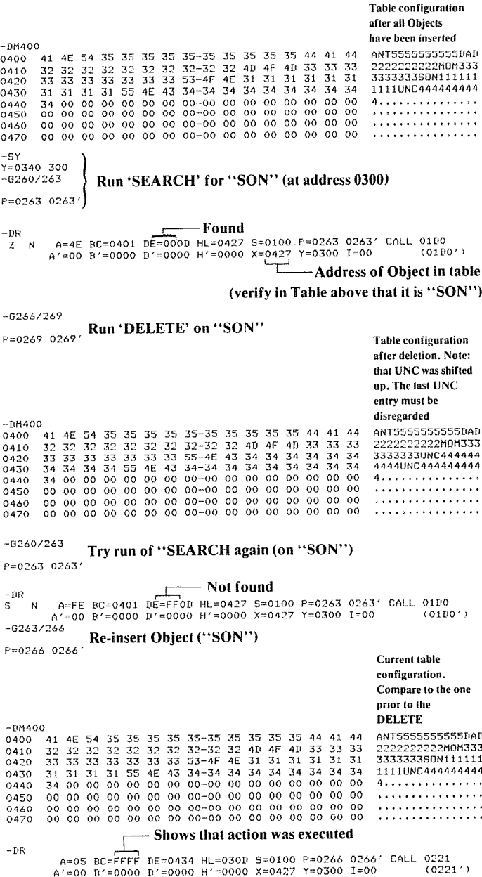
Fig. 9.24: Alphabetic List—A Sample Run (cont.)
