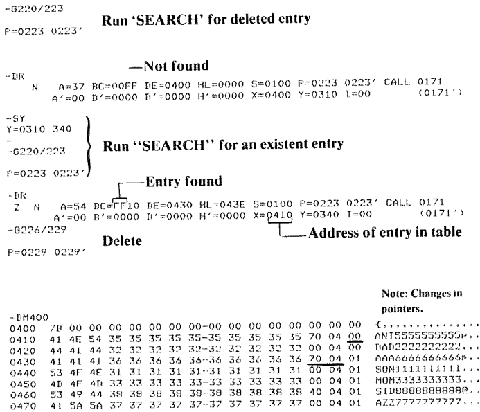
Fig. 9.30: Linked List— A Sample Run (cont.)
