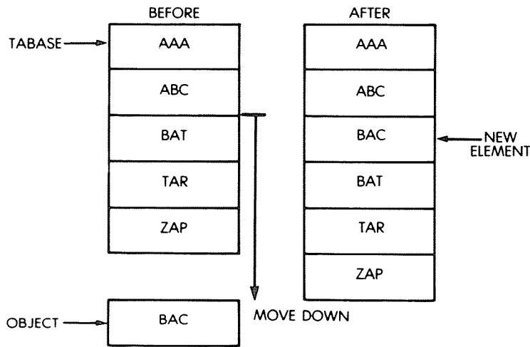
Fig. 9.20: Insert: “BAC”
