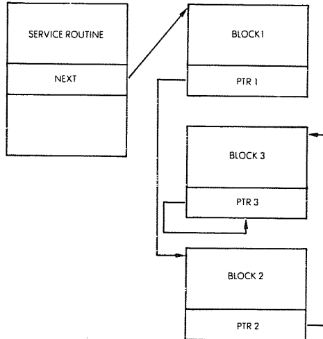
Fig. 9.5: A Queue
