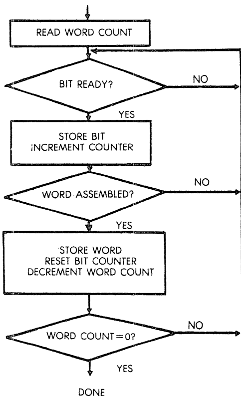
Fig. 6.6: Bit Serial Transfer—Flowchart
