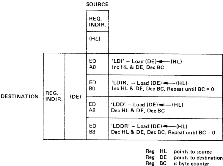
Fig. 4.5: Block Transfer Group
