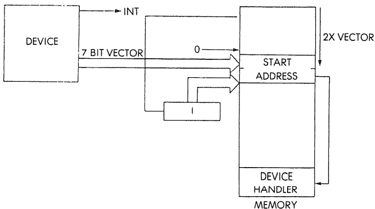
Fig. 6.29: Mode 2 Interrupt
