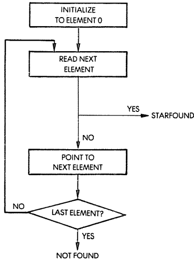
Fig. 5.6: Character Search Flowchart
