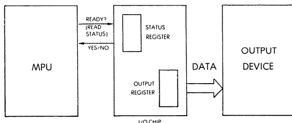
Fig. 6.8: Handshaking (Output)
