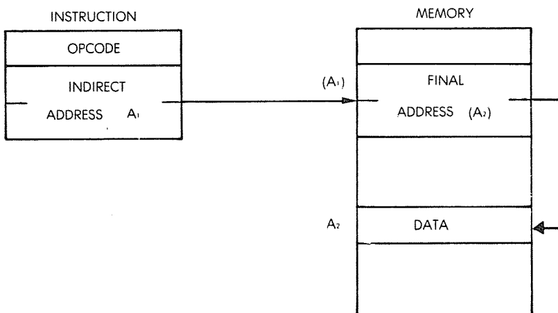
Fig. 5.4: Indirect Addressing
