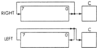
Fig. 4.12: Eight-Bit Rotation
