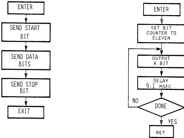
Fig. 6.16: Teletype Output
