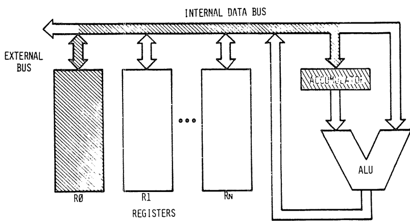
Fig. 2.9: Execution of an Addition— R0 into ACC
