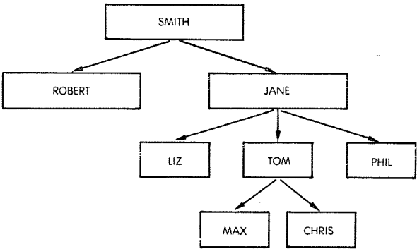
Fig. 9.7: Genealogical Tree
