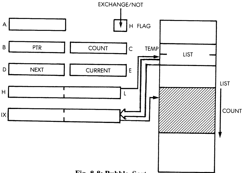
Fig. 8.8: Bubble-Sort
