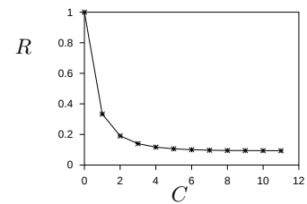
Figure 14.8. The rate of the concatenated Hamming code as a function of the number of concatenations.
