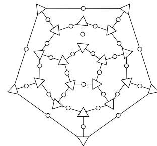
Figure 1.16. The graph defining the (30,11) dodecahedron code. The circles are the 30 transmitted bits and the triangles are the 20 parity checks, one of which is redundant.
