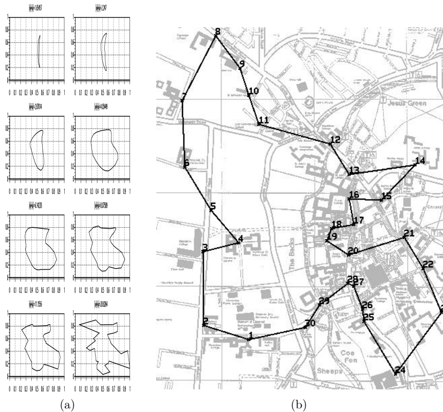
Figure 41.11. (a) Evolution of the state of a continuous Hopfield network solving a travelling salesman problem using Aiyer's (1991) graduated non-convexity method; the state of the network is projected into the two-dimensional space in which the cities are located by finding the centre of mass for each point in the tour, using the neuron activities as the mass function. (b) The travelling scholar problem. The shortest tour linking the 27 Cambridge Colleges, the Engineering Department, the University Library, and Sree Aiyer's house. From Aiyer (1991).
