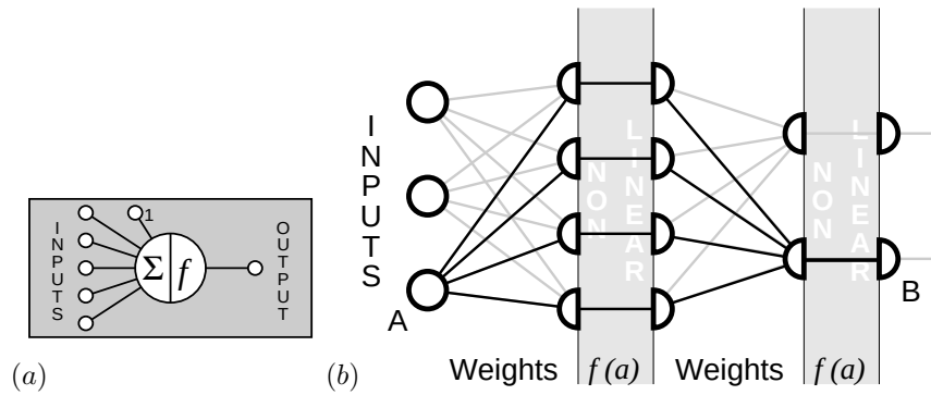
Figure 43.1. Graphical representation of a neural network. (a) A single neuron. (b) A two layer network with 3 inputs, four hidden units and 2 outputs. The weights from input A to the hidden layer have been highlighted, and the weights from the hidden layer to output B.
