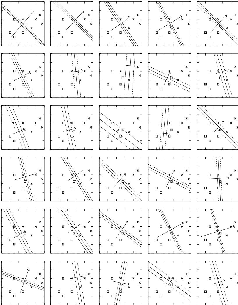
Figure 39.5. Samples obtained by the Langevin Monte Carlo method. The learning rate was set to \eta = 0.01 and the weight decay rate to \alpha = 0.01 . The step size is given by \epsilon = \sqrt{2\eta} . The function performed by the neuron is shown by three of its contours every 1000 iterations from iteration 10000 to 40000. The contours shown are those corresponding to a = 0, \pm 1 , namely y = 0.5, 0.27 and 0.73 . Also shown is a vector proportional to (w_1, w_2) .
