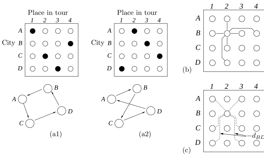
Figure 41.10. Hopfield network for solving a travelling salesman problem with K = 4 cities. (a1,2) Two solution states of the 16-neuron network, with activities represented by black = 1, white = 0; and the tours corresponding to these network states. (b) The negative weights between node B2 and other nodes; these weights enforce validity of a tour. (c) The negative weights that embody the distance objective function.
