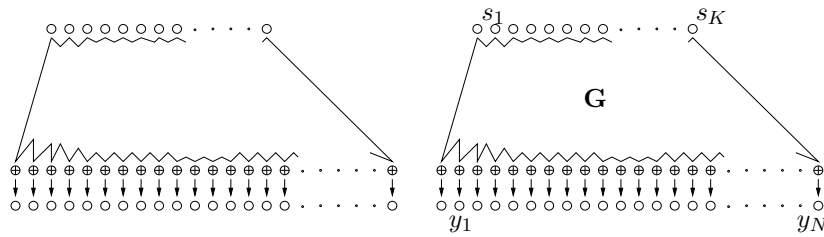
Figure 22.1. Error-correcting codes as latent variable models.
