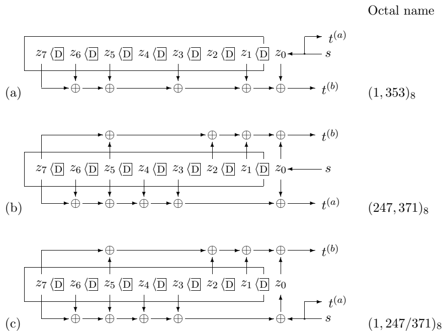
Figure 57.1. Linear feedback shift registers for generating convolutional codes with rate 1/2 . After Frey (1998).
