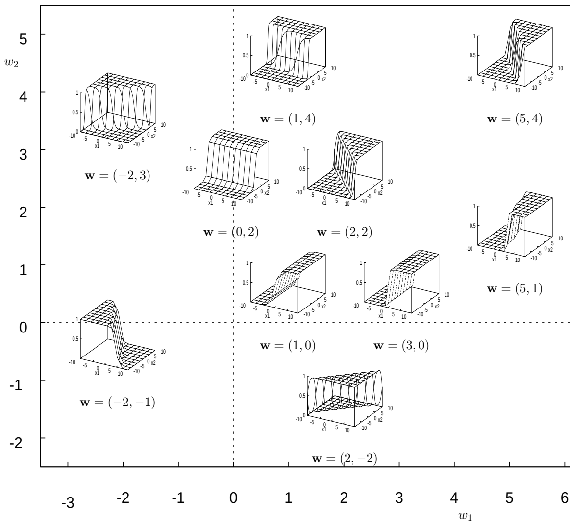
Figure 37.3. Weight space.
