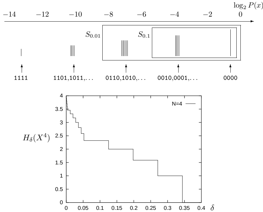
Figure 5.6. The sixteen outcomes of the ensemble X^4 with p_1 = 0.1 , ranked by probability, and the essential bit content H_\delta(X^4) . The upper schematic diagram indicates the strings's probabilities by the vertical lines's lengths (not to scale).
