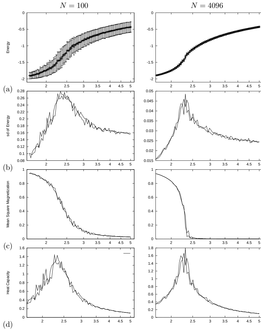
Figure 29.5. Detail of Monte Carlo simulations of rectangular Ising models with J = 1 . (a) Mean energy and fluctuations in energy as a function of temperature. (b) Fluctuations in energy (standard deviation). (c) Mean square magnetization. (d) Heat capacity.
