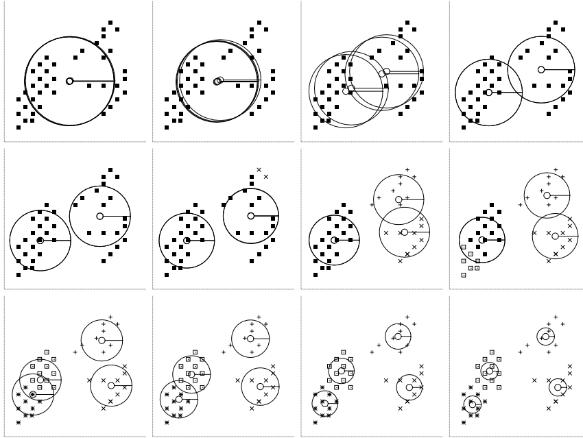
Figure 21.5. Soft K means algorithm, version 1, applied to a data set of 40 points. K = 4 . Implicit lengthscale parameter 1/\beta^{1/2} varied from a large to a small value. Each picture shows the state of all four means, with the implicit lengthscale shown by four circles surrounding them, after running the algorithm for several tens of iterations. At the largest lengthscale 1/\beta^{1/2} , all four means converge exactly to the data mean. Then the four means separate into two groups of two. At shorter lengthscales, each of these pairs itself bifurcates into subgroups.
