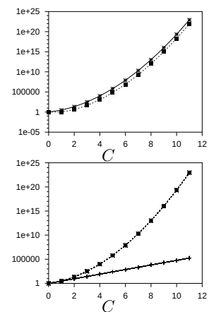
Figure 14.9. The parameters (N, K) (upper figure) and (N, d) (lower figure) of the concatenated Hamming code as a function of the number of concatenations. d is the minimum distance.
