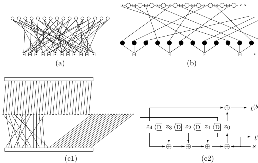
Figure 55.1. Graphs of three sparse graph codes. (a) A rate 1/4 low-density parity-check code (Gallager code) with blocklength N = 16 , and M = 12 constraints. Each white circle represents a transmitted bit. Each bit participates in j = 3 constraints, represented by \square squares. Each \square constraint forces the sum of the k = 4 bits to which it is connected to be even. (b) A repeat-accumulate code with rate 1/3. Each white circle represents a transmitted bit. Each black circle represents an intermediate binary variable. Each \square constraint forces the variables to which it is connected to be equal. (c) A turbo code with rate 1/3. (c1) The circles represent the codeword bits. The two rectangles represent rate 1/2 convolutional codes, with the systematic bits occupying the left half of the rectangle and the parity bits occupying the right half. (c2) Each trellis is generated by a (21/37)_8 recursive filter which has a state space of 4 bits.
