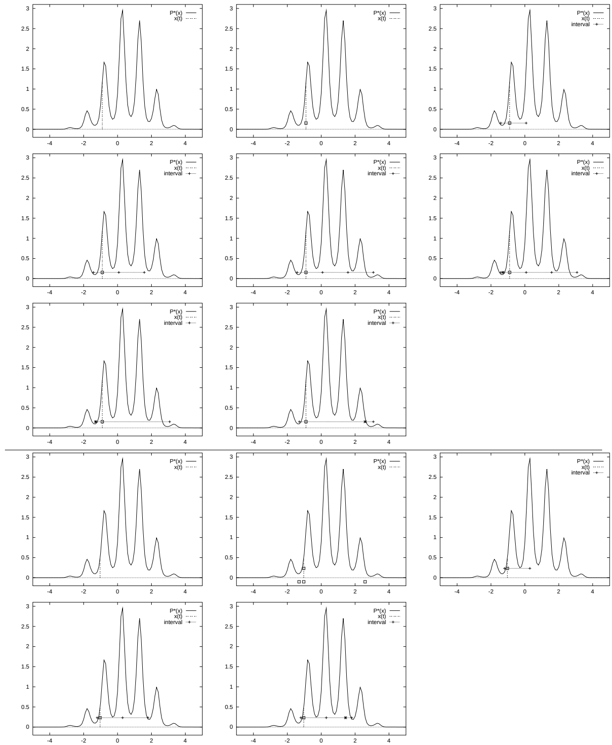
Figure 27.13. Slice sampling
