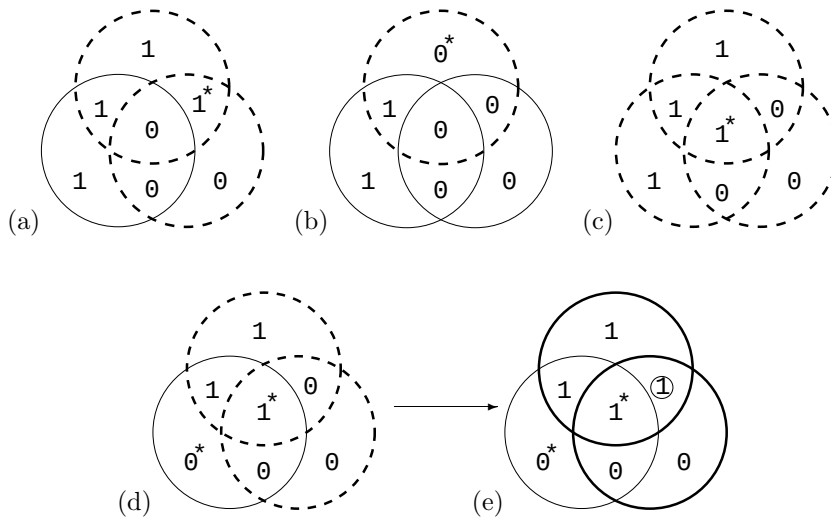
Figure 1.11. Pictorial representation of decoding of the Hamming (7,4) code. The bits that are flipped relative to figure 1.9(b) are labelled by \star . The violated parity checks are highlighted by dashed circles. One of the seven bits is the most probable suspect to account for each ‘syndrome’, i.e., each pattern of violated and satisfied parity checks.
