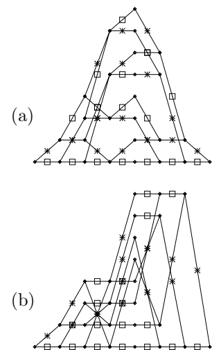
Figure 23.6. Trellises for the permuted (7,4) Hamming code generated from (a) the generator matrix by the method of figure 23.5; (b) the parity-check matrix by the method on page 318. 1110001001111010 Each edge in a trellis is labelled by a zero (shown by a square) or a one (shown by a cross).
