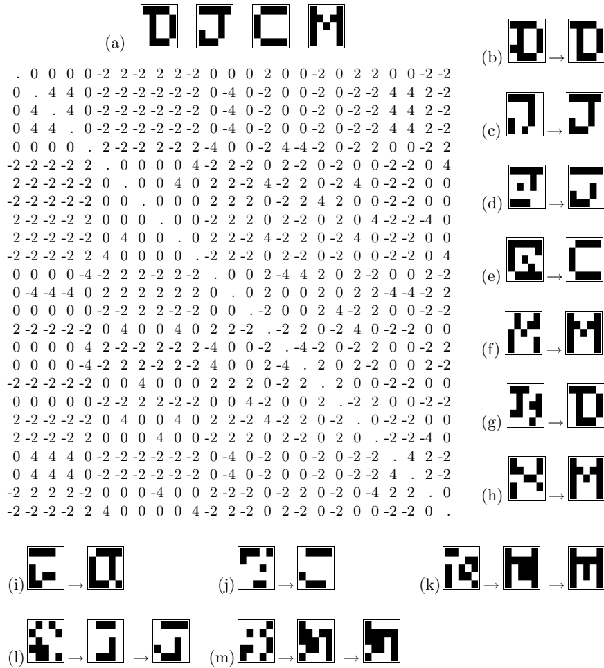
Figure 41.3. Binary Hopfield network storing four memories. (a) The four memories, and the weight matrix. (b–h) Initial states that differ by one, two, three, four, or even five bits from a desired memory are restored to that memory in one or two iterations. (i–m) Some initial conditions that are far from the memories lead to stable states other than the four memories; in (i), the stable state looks like a mixture of two memories, ‘D’ and ‘J’; stable state (j) is like a mixture of ‘J’ and ‘C’; in (k), we find a corrupted version of the ‘M’ memory (two bits distant); in (l) a corrupted version of ‘J’ (four bits distant) and in (m), a state which looks spurious until we recognize that it is the inverse of the stable state (l).
