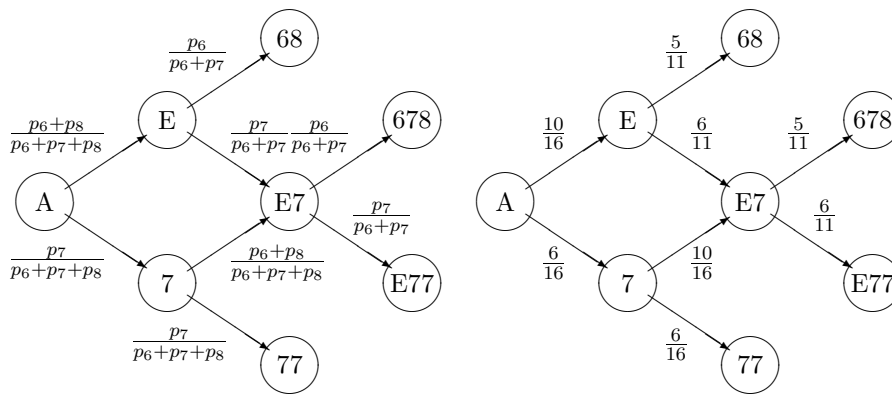
Figure 25.3. Markov process describing the Las Vegas dice game, pruned of all irrelevant outcomes. The end states 68 and 678 are wins for Joe. States E77 and 77 are wins for you. Please do not confuse this state diagram, in which arrows indicate which states can follow from each other, with a graphical model, in which each node represents a different variables and arrows indicate causal relationships between them.
