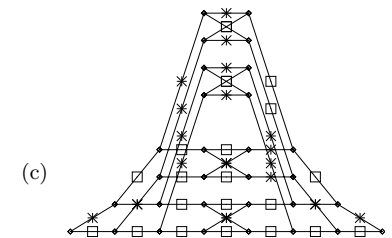
(7,4) Hamming code
