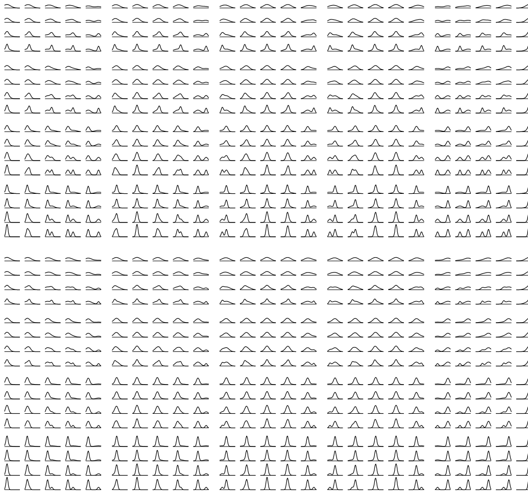
Figure 24.4. Mixture of two Gaussians. Each mini-figure shows the probability density of x for \mu . The mixing coefficients are 0.6, 0.4 in the top half and 0.8, 0.2 in the bottom half. Means \mu_1 and \mu_2 are horizontally separated by 4 units, and standard deviations \sigma_1 and \sigma_2 are vertically separated by 4 units (a Cauchy distribution) and (2, 4) (light line), and a Gaussian distribution with mean \mu = 3 and standard deviation \sigma = 3 , shown on linear vertical scales (top) and logarithmic vertical scales (bottom). Notice that the heavy tails of the Cauchy distribution are scarcely evident in the upper ‘bell-shaped curve’.
