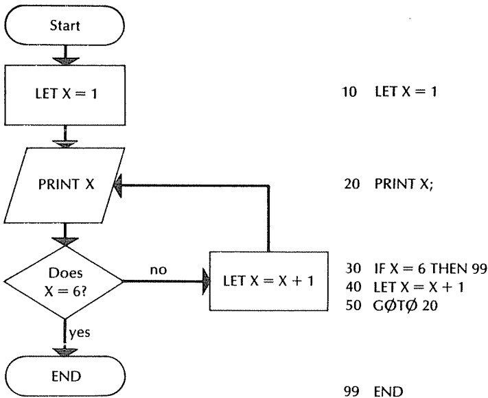
Fig. 3-1. Flowchart for LØØP1 for printing six integers.
