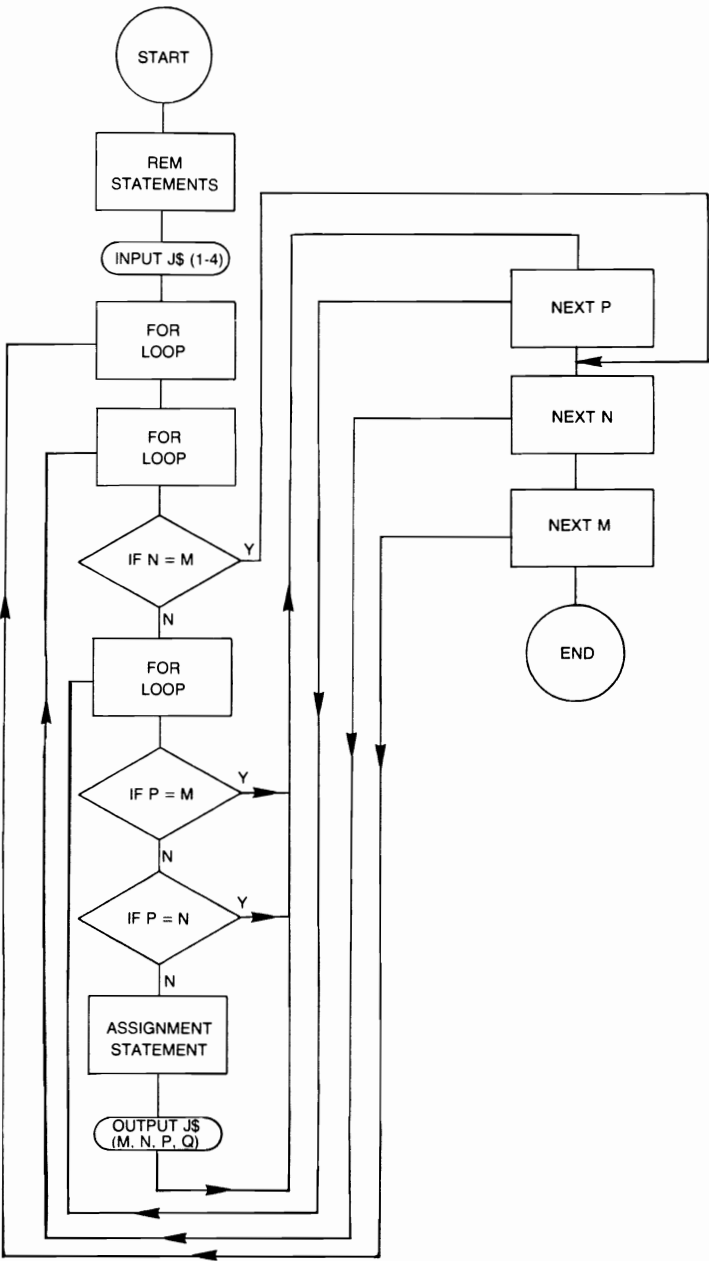
Flowchart for String manipulation.
