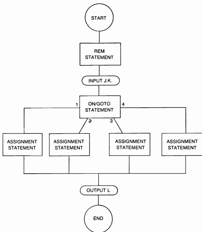
Flowchart for ON/GOTO statement.
