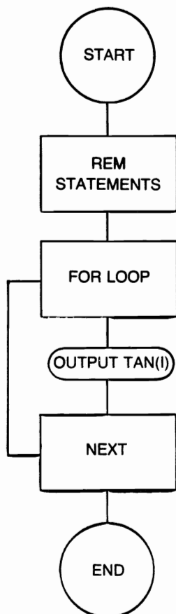
Flowchart for TAN function.
