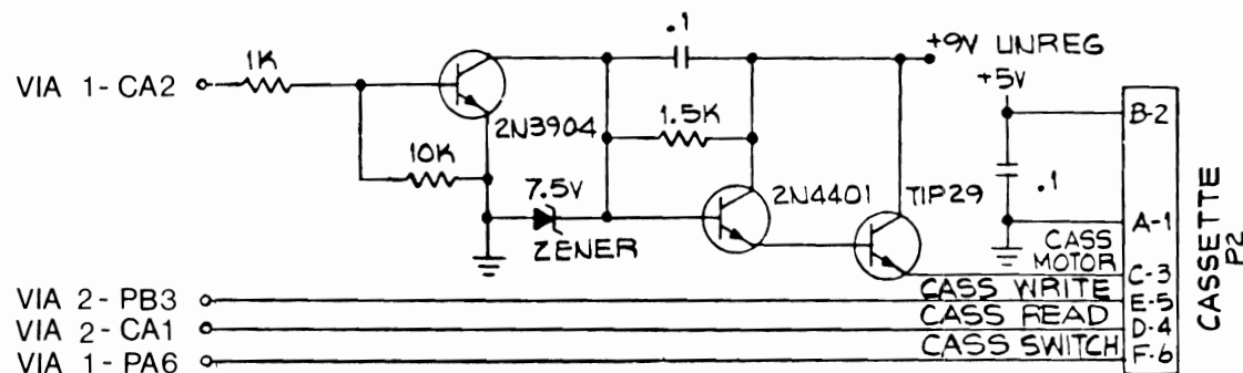
Fig. 26 — The cassette circuit and its connection to the 6522 chips.
