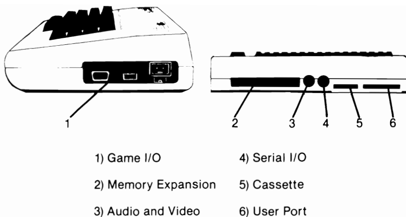
Fig. 20 — Position of the different VIC I/O outputs.
