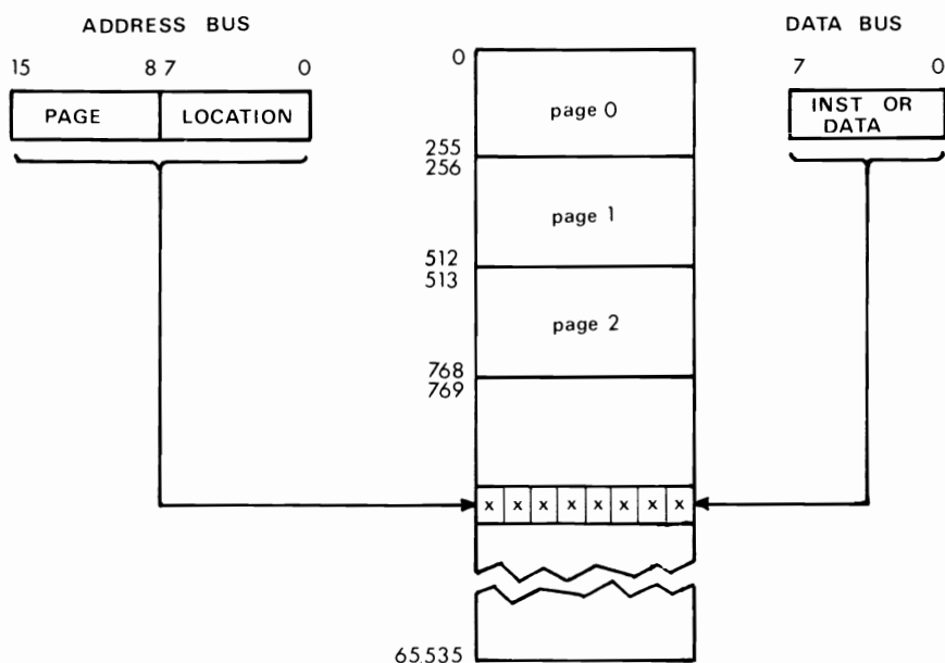
Fig. 2 — Relation between address, data, and memory location.
