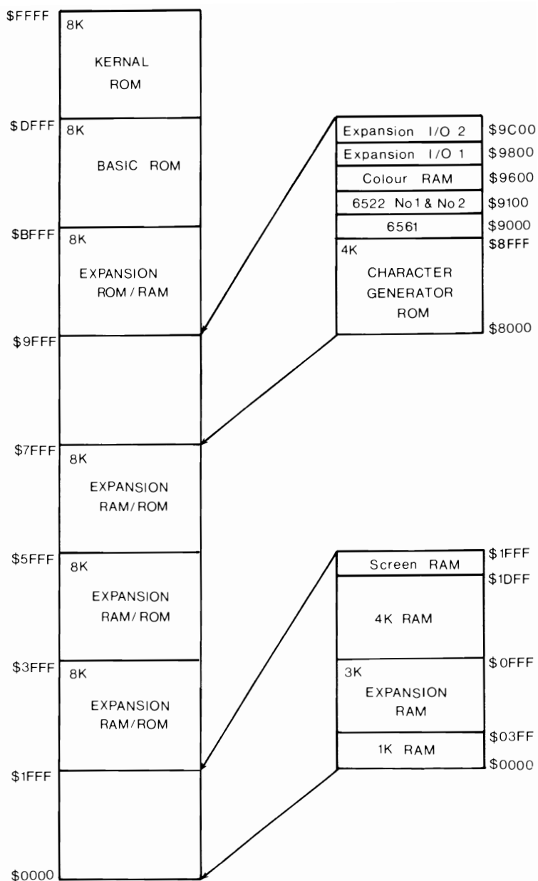
Fig. 8 — VIC memory map.
