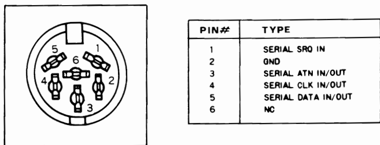
Fig. 39 — The allocation and function of pins on the IEEE Port connector.
