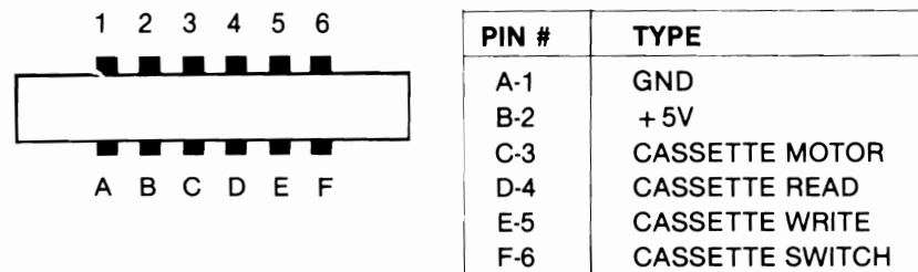
Fig. 25 — The allocation and function of pins on the Cassette connector.
