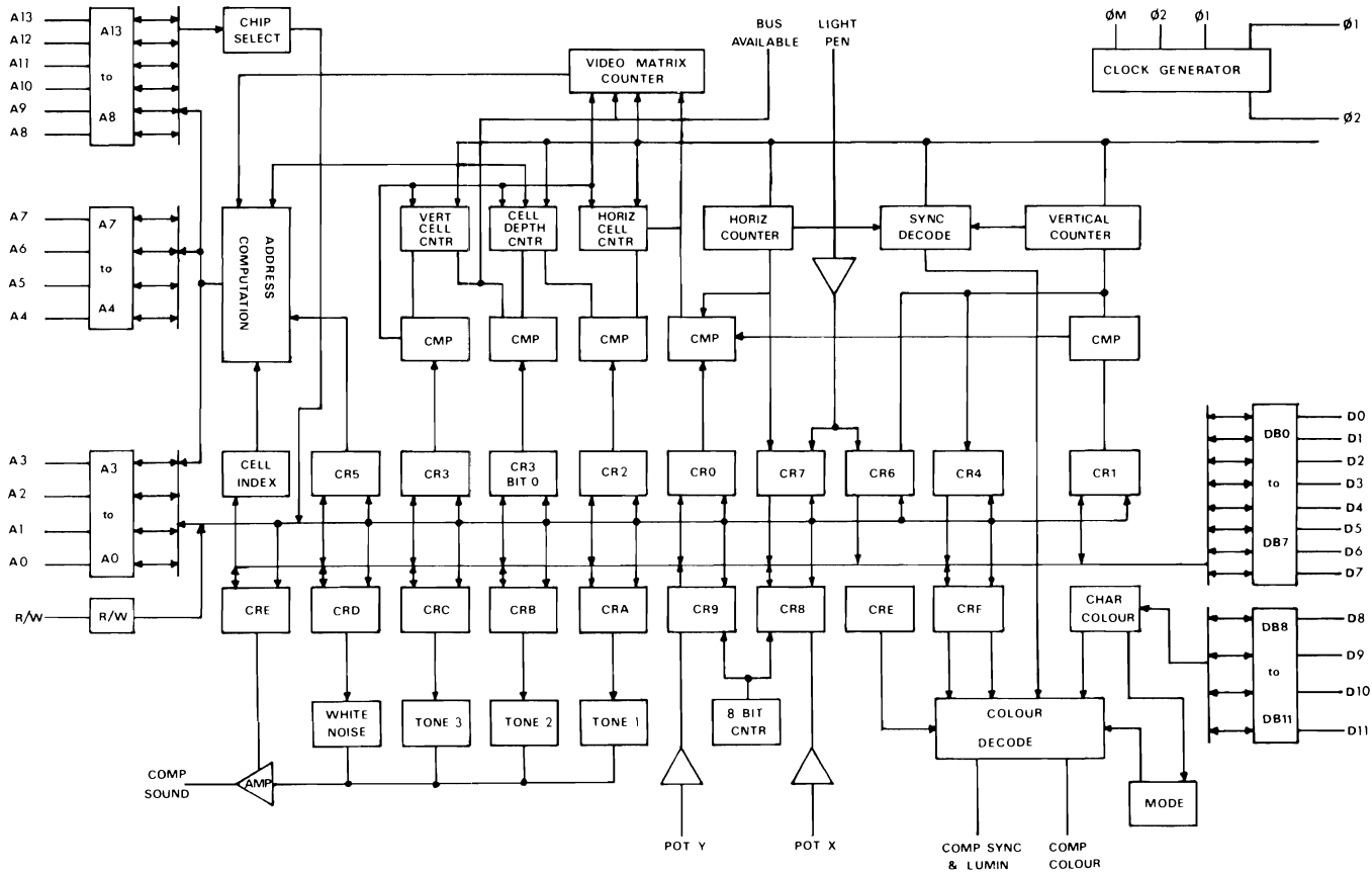
Fig. 13 — Block diagram of the 6561 Video Interface chip.
