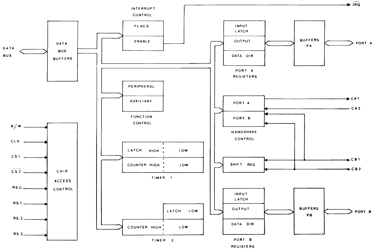
Fig. 18 — Block diagram of the 6522 Versatile Interface Adapter chip.
