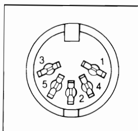
Fig. 23 — The allocation and function of pins on the Audio/Video connector.
