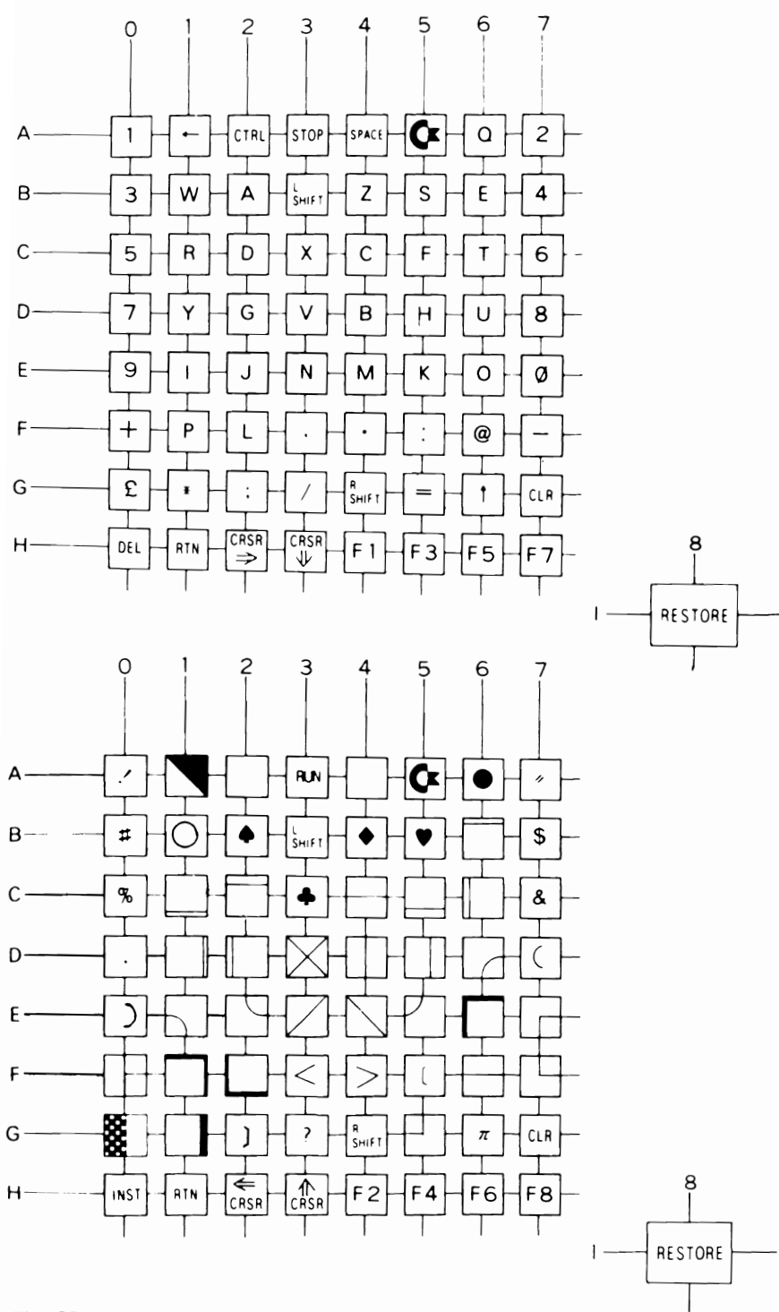
Fig. 29 — Matrix of keyboard connections to 6522 I/O lines.
