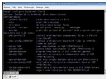
Running configure with the --help parameter outputs a lot of text, so pipe it through less to make it easier to read
