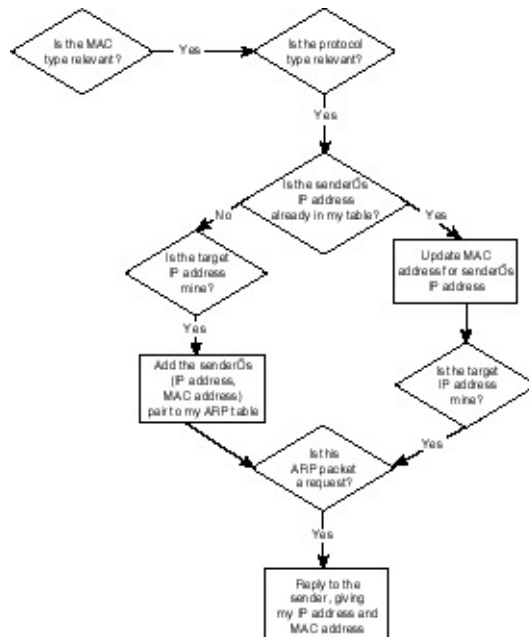
Figure 4.3. A receipt of an ARP packet (constructed from information in RFC 826).
