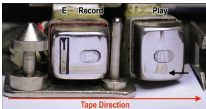
Figure 2: Two of the three Echoplex heads clearly show signs of wear, although not as extreme as the Roland Space Echo heads in Fig. 1. To the left is the combo erase/record head, mounted on a slider to increase the distance between it and the play head to the right.
