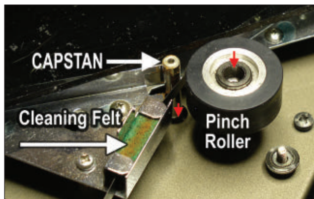
Figure 3: The Space Echo's capstan and pinch roller, the latter with its retaining cap removed. Notice how the pinch is lifted up and staying in position because the lubricant is so stiff (not good).
