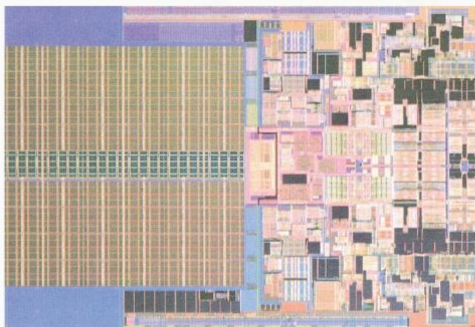
Intel's Penryn at a glance. To the left, you can see the massive 6MB of cache that supports each die's two cores.
